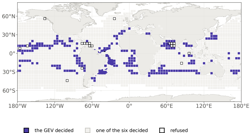
(b) where Anderson–Darling among seven names the GEV, daily maxima
