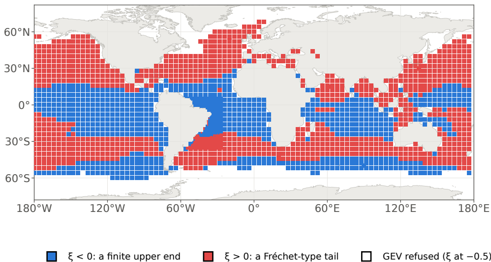
(a) the sign of the GEV shape \xi , daily maxima (certified; every box excludes zero)
