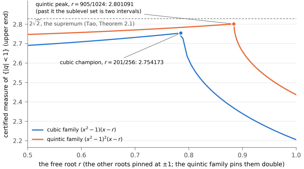
Figure 1: The two families against the free root r : 163 certified enclosures recomputed for this document (the plotted value is the upper end; widths are far below the resolution of the picture). The quintic family is drawn at step 1/128 and, between r = 3600/4096 and 3664/4096 , at step 1/4096 . Both families reach their maximum where their sublevel set is still one interval and descend as soon as it splits.
