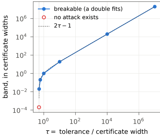
(b) the band dial on erdos1038.upper
