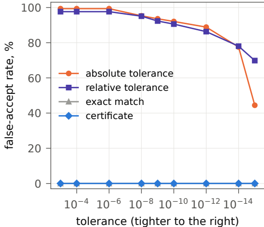
(a) false-accept rate against tolerance
