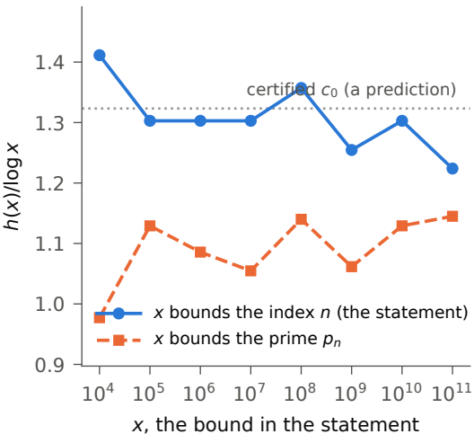
(a) the ratio under the two readings
