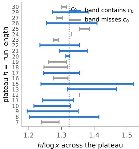
(b) each plateau of h as a band
