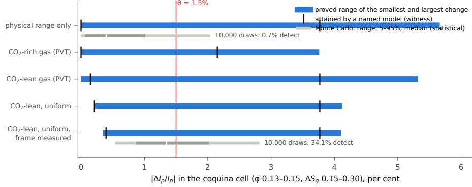
Figure 3: The headline cell: the proved range of |\Delta I_p/I_p| and the attained extremes under each knowledge state, against the pilot’s resolution; beside K0 and K4, the range, the 5–95% band and the median of 10,000 uniform draws of the same envelope (statistical, not certified).
