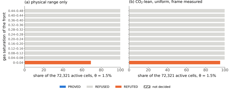
Figure 2: The share of the field’s active cells by verdict at 1.5% for each gas saturation of the front: (a) the physical range alone; (b) CO 2 -lean gas, uniform, frame measured.
