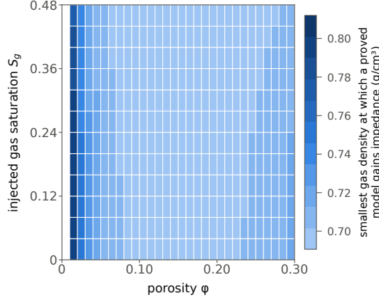
Figure 4: The sign map under the physical range: the smallest injected-gas density at which a proved admissible model gains impedance, per cell; hatched cells are those where no gaining model was found within the budget. Above the mapped density the sign of the 4D change is not guaranteed.
