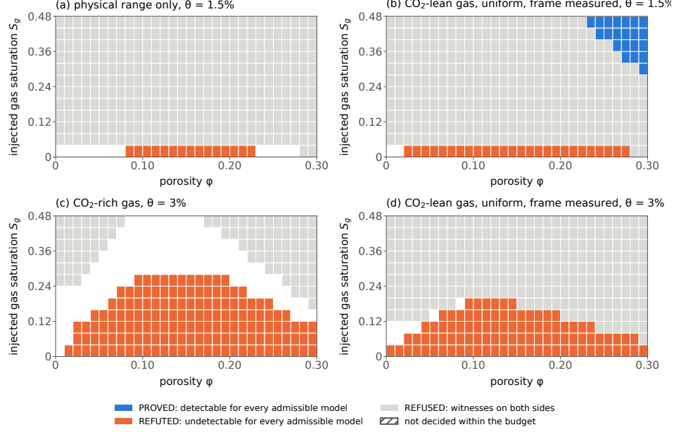
Figure 1: The decidability map: each cell a porosity bin by an injected-gas-saturation bin, decided over every declared range. (a) The physical range alone at the pilot’s resolution of 1.5%; (b) CO 2 -lean gas, uniformly distributed, frame stiffness measured, at 1.5%; (c) CO 2 -rich gas at 3%; (d) as (b) at 3%.
