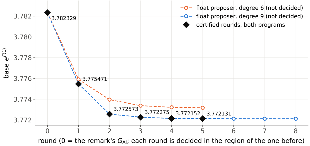
Figure 2: The certified bases of the 6 rounds (filled diamonds, both programs) beside the float proposer's sequences (hollow markers on dashed lines, never decided). Decided and proposed values share neither colour nor mark.
