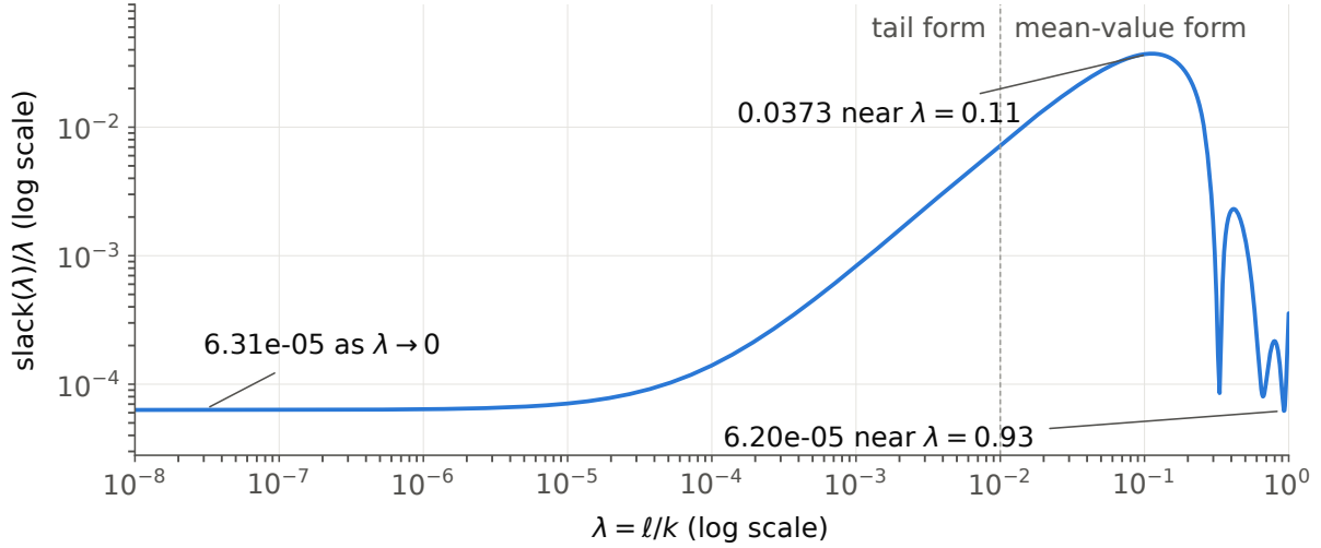
Figure 1: Round 1: the slack of Theorem 3’s inequality divided by \lambda , as the lower end of an interval enclosure at each of 160 points (the decision is the cover of Table 3, not these points). It is flat near 6.31 \times 10^{-5} for small \lambda , rises to 0.0373 near \lambda = 0.11 , falls to 6.20 \times 10^{-5} near \lambda = 0.93 , and ends at 3.56 \times 10^{-4} at \lambda = 1 . The flat left end and the three dips between 0.6 and 0.95 are where a coarser witness, or a slightly more ambitious q , is refused; the control that moves the linear coefficient to -0.3870 fails at the left end.
