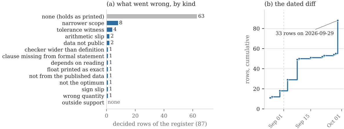
Figure 1: (a) The 87 decided rows by defect kind; the vocabulary’s kinds with no row are drawn empty. (b) The register as a dated diff: cumulative rows by the day a record first held them, with the month boundary dashed. Both panels are drawn from certs/claims-ledger.json .
