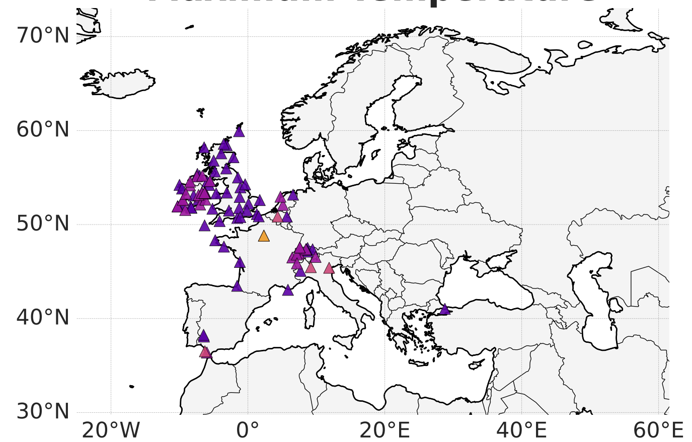
Maximum Temperature
