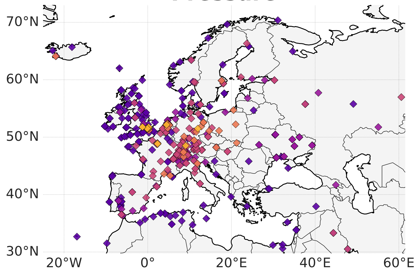
Pressure
