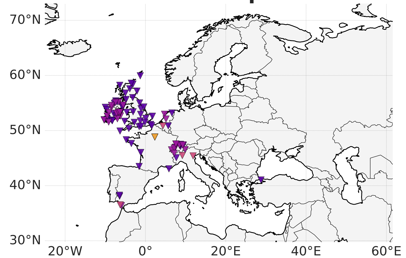
Maximum Temperature
