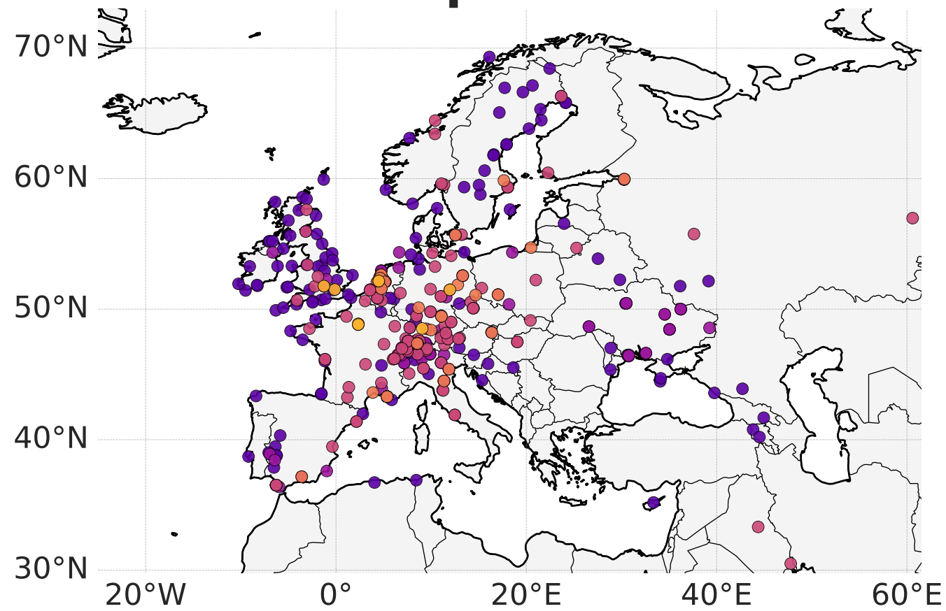
Pressure
