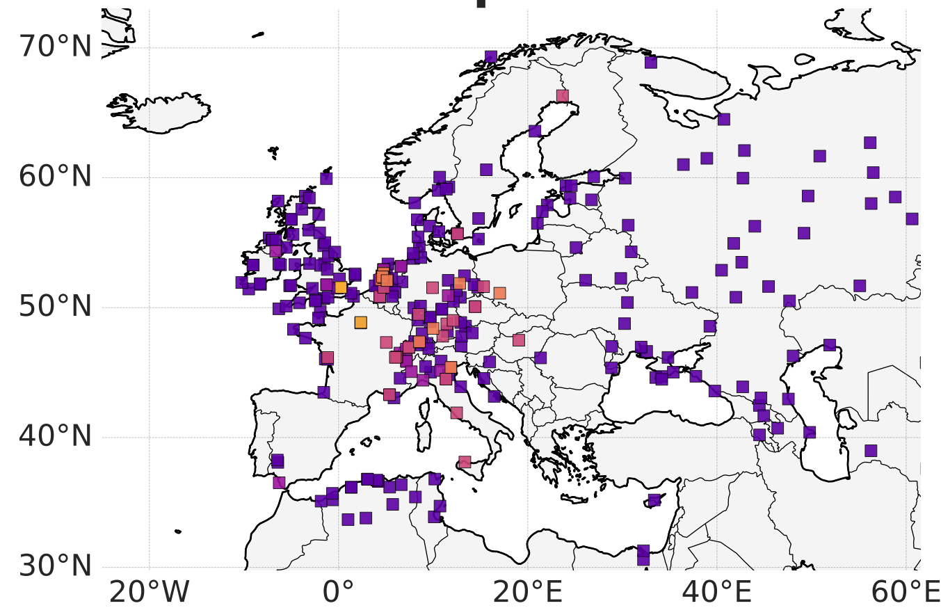
Wind Direction
