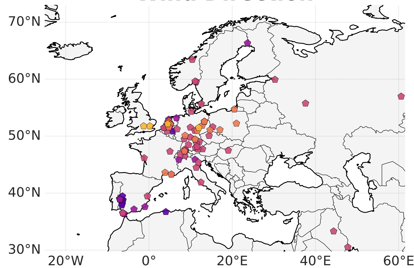
Wind Direction
