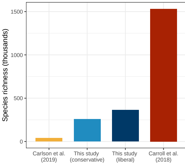
A Estimated global diversity of mammal-infective viruses
