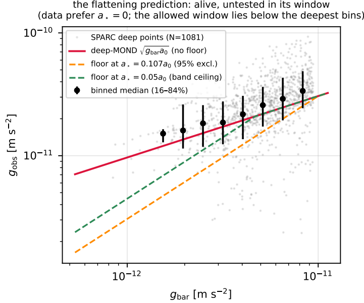
Figure 4: The deep-MOND flattening prediction against SPARC’s deepest decade (agent CC): the binned medians follow the \sqrt{g_{\text{bar}} a_0} law with no downturn; a floor at a_* = 0.107 a_0 (orange) is excluded at 95%, while the allowed window ( a_* < 0.05 a_0 , green curve illustrating the band ceiling) lies below the deepest usable bins — the prediction is alive and untested where it must be tested.
