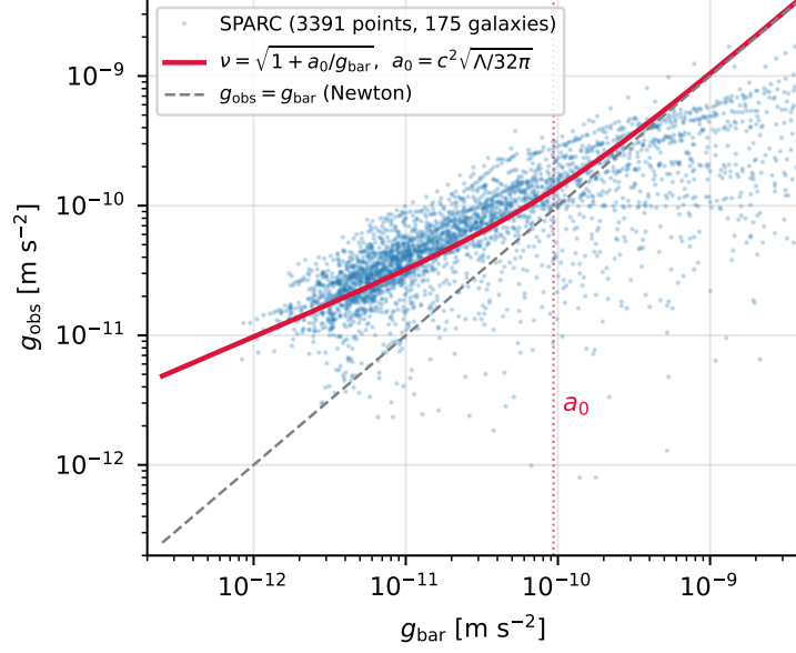
Figure 1: The radial acceleration relation on SPARC (175 galaxies, locked conventions \Upsilon_d = 0.52 , framework footing): the kernel a_0 = c^2 \sqrt{\Lambda/32\pi} with the baseline interpolation \nu = \sqrt{1 + a_0/g_{\text{bar}}} . Generated from the repository data by make_figures.py (as are all figures; no illustration is hand-drawn).
