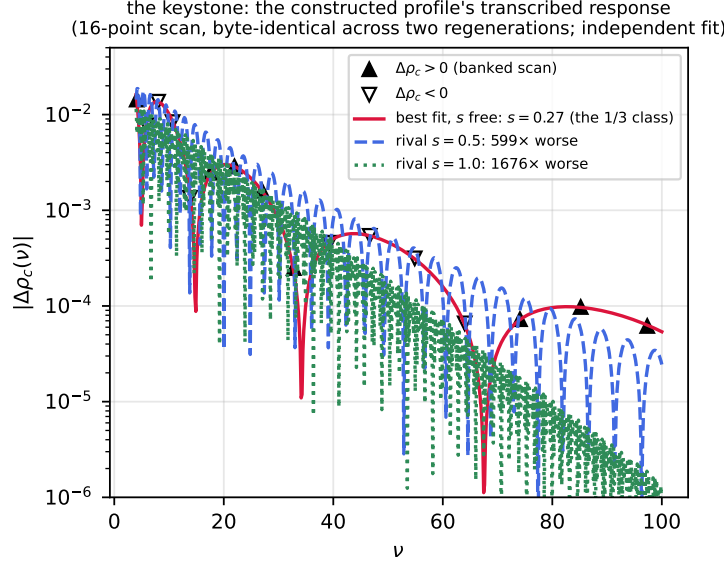
Figure 5: The Link 5 keystone (agent HH): the constructed pump profile's transcribed worldline response (the 16-point scan, byte-identical across two independent regenerations; triangles mark sign). The free-index fit lands in the index-1/3 class ( s = 0.27 , within the window's \pm 0.06 identifiability of 1/3 ); rival index classes fit \geq 599\times worse (seed-matched reproduction of the banked protocol; the s=1 ratio varies 1120\text{--}1676\times across multistart draws, decisive in all).
