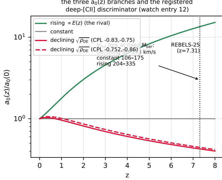
Figure 2: The three a_0(z) branches (the framework’s declining \sqrt{\rho_{\text{DE}}} under both locked CPL sets; constant; the rival rising E(z) ) and the registered deep-[CII] discriminator: at REBELS-25 ( z = 7.31 ), one rotation curve extended past r_{\text{MOND}} splits the branches by \times 2.3\text{--}2.4 in asymptotic velocity at fixed baryonic mass (watch entry 12).
