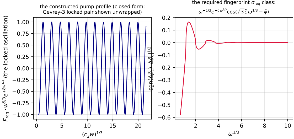
Figure 6: The constructed objects in closed form (framework footing): left — the pump profile F_{\text{req}} with envelope removed, showing the locked Gevrey-3 oscillation the dynamics must be handed; right — the required spectral fingerprint class \omega^{-1/3} e^{-\tilde{c}\omega^{1/3}} \cos(\sqrt{3}\tilde{c}\omega^{1/3} + \tilde{\varphi}) (signed square-root scale). The generation-obstruction theorem says the left panel cannot be composed by any structureless scale-invariant gain — only transcribed.
