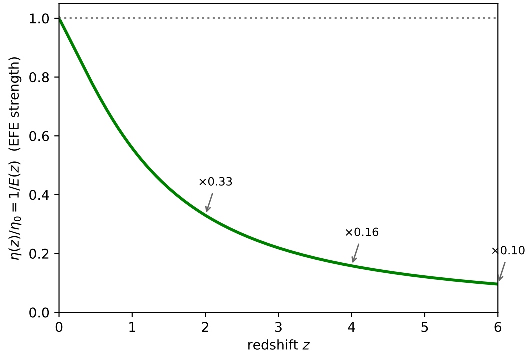
(b) the External Field Effect weakens with z
