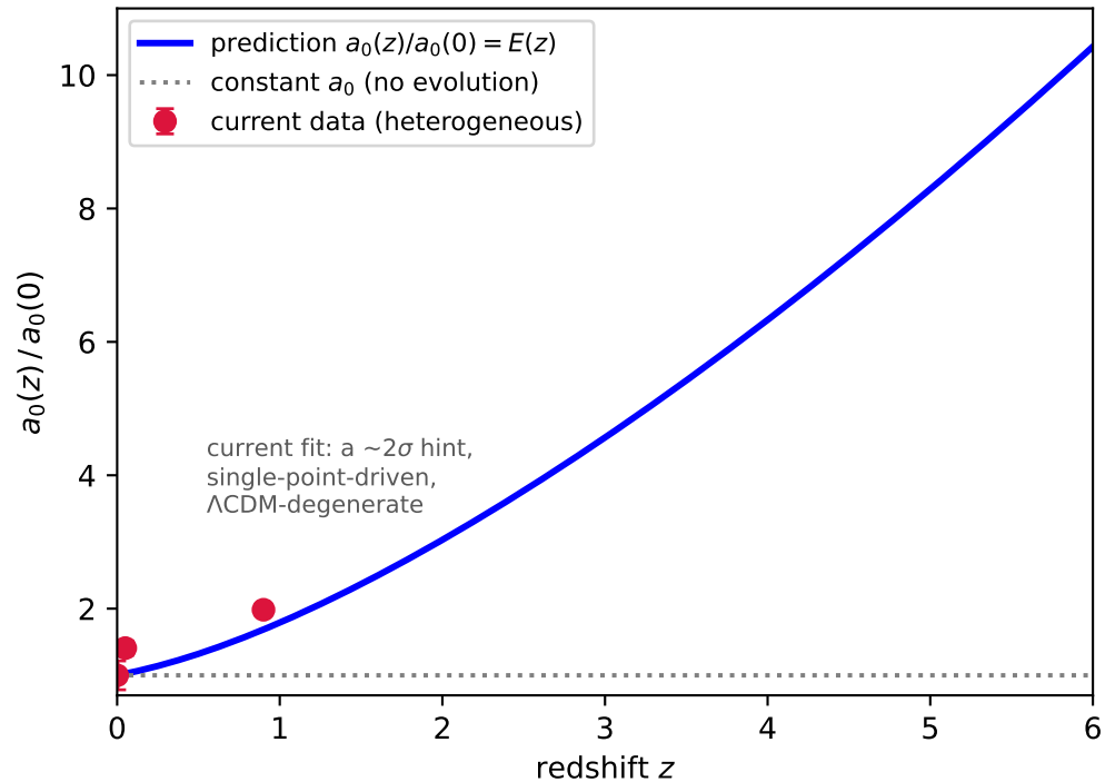
(a) the evolving scale a_0(z) = a_0(0) E(z)
