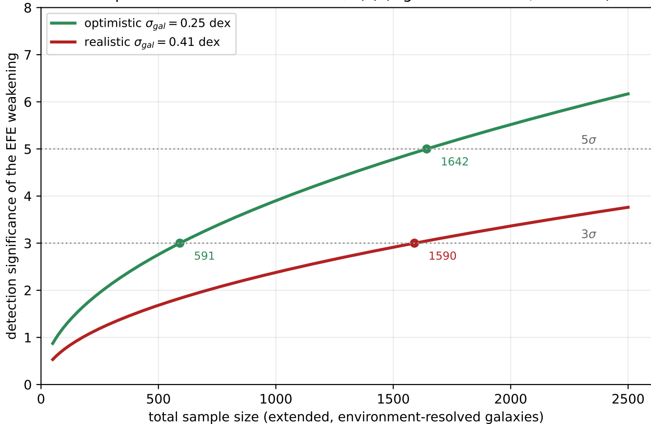
Sample needed to detect EFE \propto 1/E(z) (signal \approx 0.12 dex, z = 0 \rightarrow 6 )
