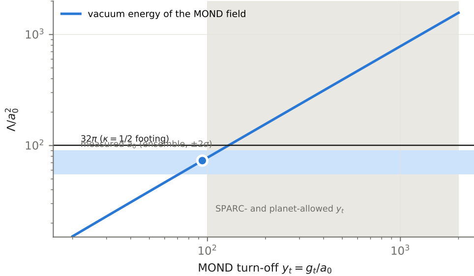
Figure 1: The MOND field’s vacuum energy \Lambda c^4/a_0^2 against its turn-off y_t (blue). Horizontal band: the value required by the observed \Lambda with measured a_0 ( \pm 2\sigma ); the dot marks the central solution y_t = 94 . Black line: the \kappa = \frac{1}{2} footing. Shaded: turn-offs allowed by SPARC and the planets.
