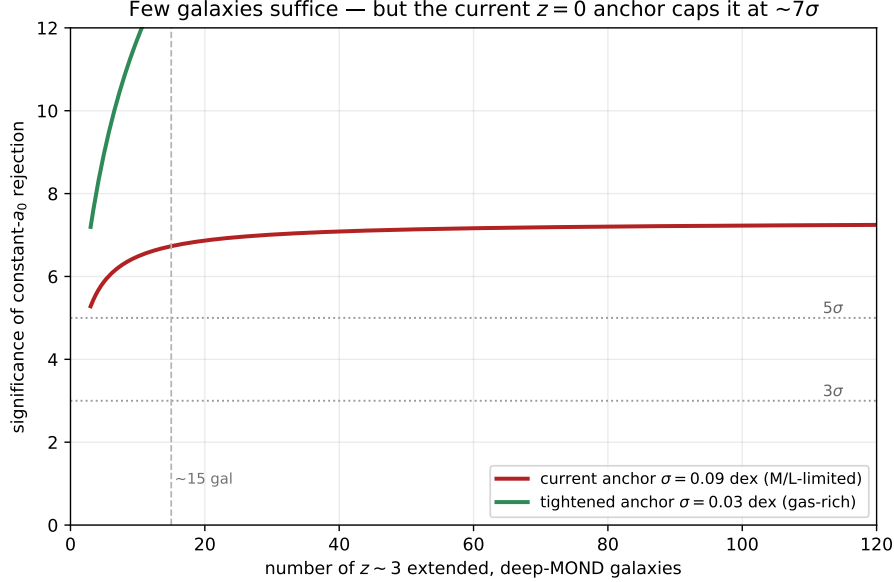
Figure 2: Constant- a_0 rejection versus sample size at z \simeq 3 ( \sigma_{\text{gal}} = 0.15 dex). The current z = 0 anchor caps the significance near 7\sigma (red); a tighter anchor (green) unlocks higher significance.
