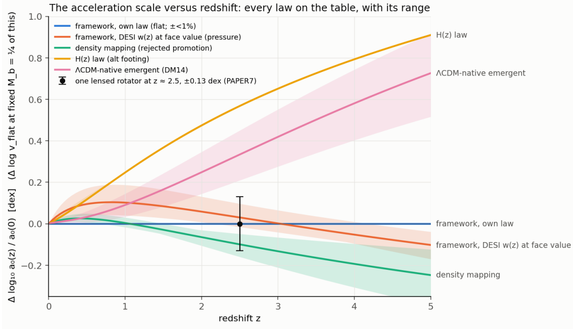
Figure 1: \Delta \log_{10} a_0(z)/a_0(0) for every law on the table, with its range: the framework’s own law (flat), the framework with DESI’s w(z) at face value through the pressure law, the rejected density mapping, the H(z) law (the alternative a_0 footing), and the \Lambda CDM-native emergent scale. The black bar is the pre-registered single-rotator precision, \pm 0.13 dex at z \simeq 2.5 . \Delta \log V_{\text{flat}} at fixed baryonic mass is one quarter of the vertical axis.
