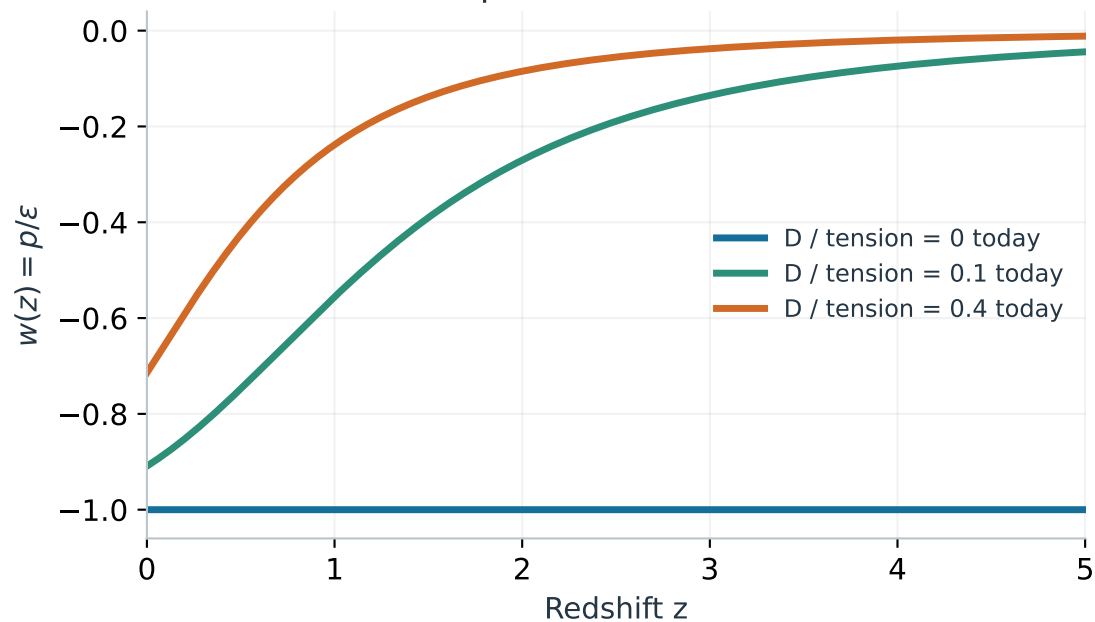
Same constant pressure and scale, different w
