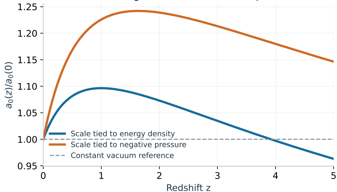
Same evolving fluid, different scale predictions
