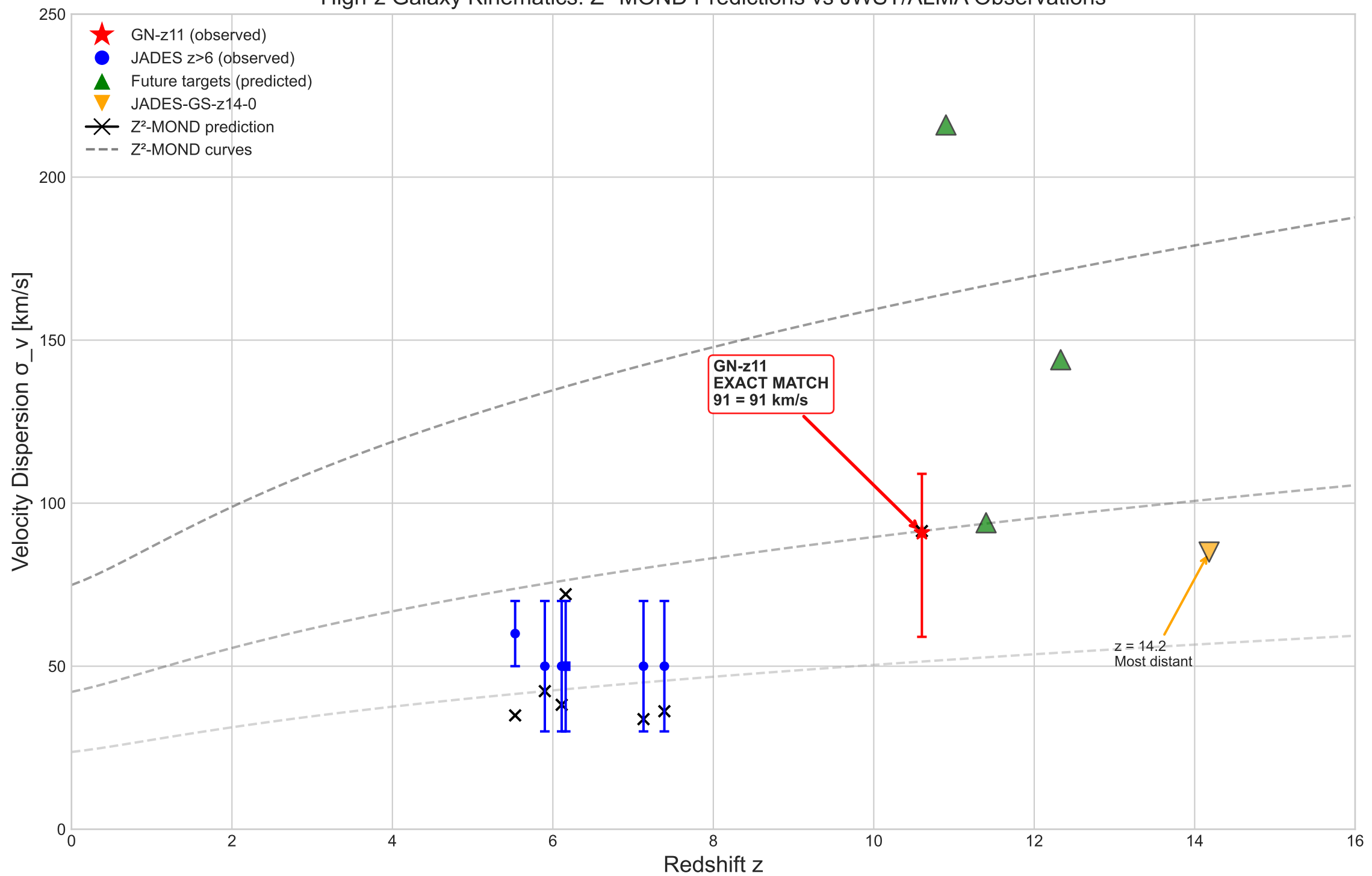
High-z Galaxy Kinematics: Z 2 -MOND Predictions vs JWST/ALMA Observations
