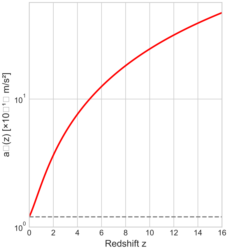
C) MOND Scale Evolution
