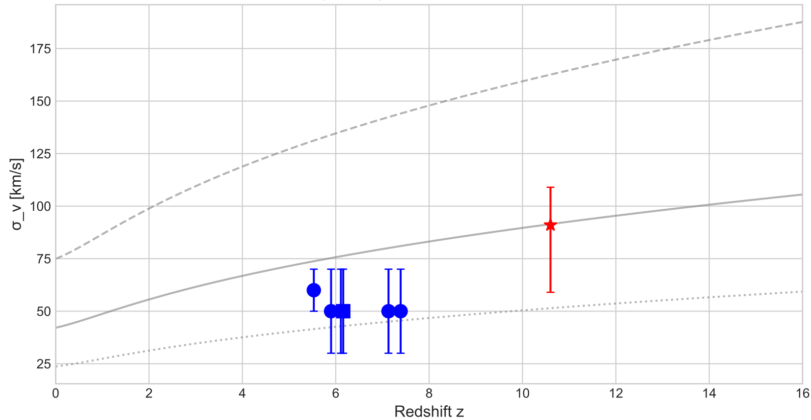
A) Velocity Dispersion vs Redshift
