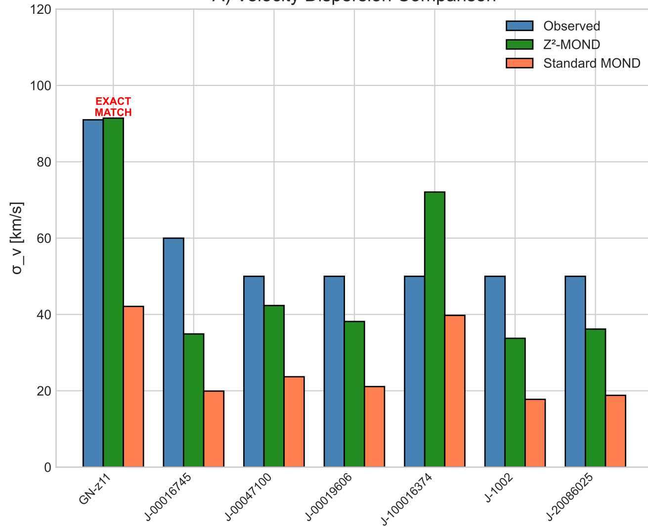
A) Velocity Dispersion Comparison
