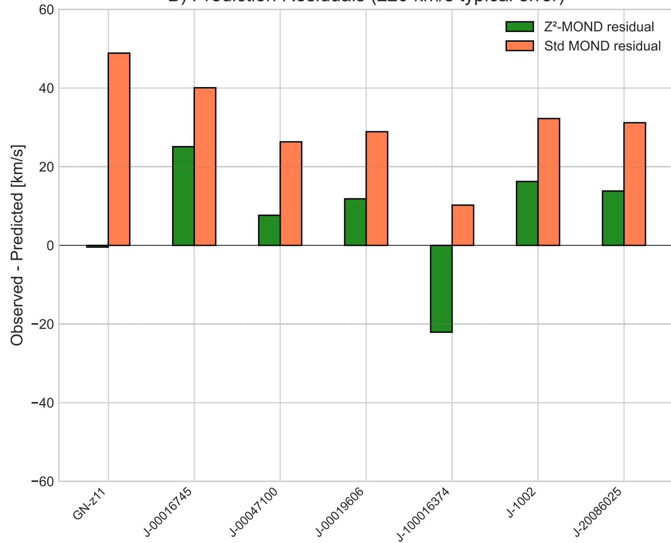
B) Prediction Residuals ( \pm 20 km/s typical error)
