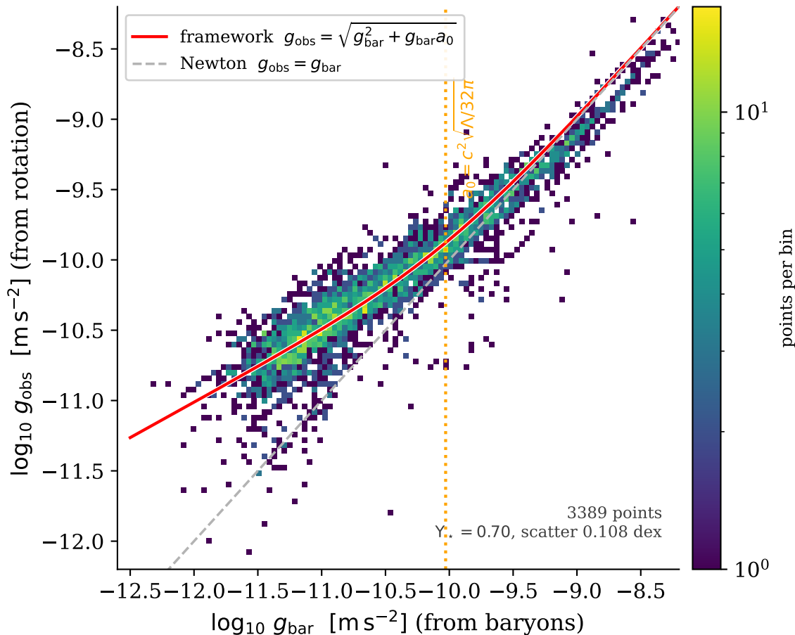
The radial-acceleration relation: 175 SPARC galaxies vs the horizon-derived a_0 (no dark matter, no fit to these points)
