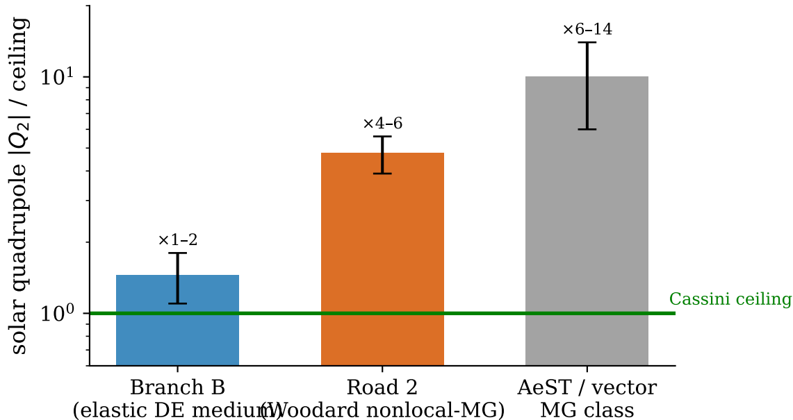
Cassini Q_2 : no-dark-matter lensing roads vs the bound (Branch B least-constrained; all are dark-matter-free)
