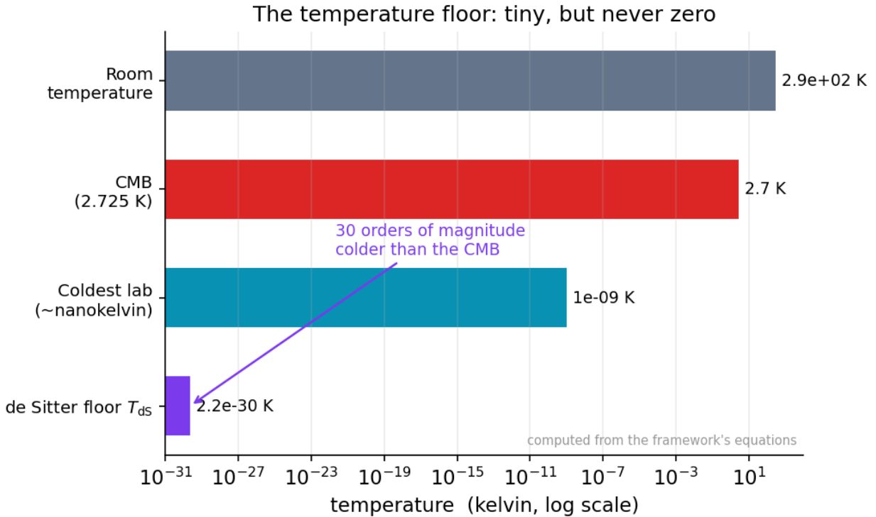
Figure 43: Horizontal bar chart on a log temperature scale comparing room temperature, the CMB, a nanokelvin lab, and the de Sitter floor, which is vastly smaller.
