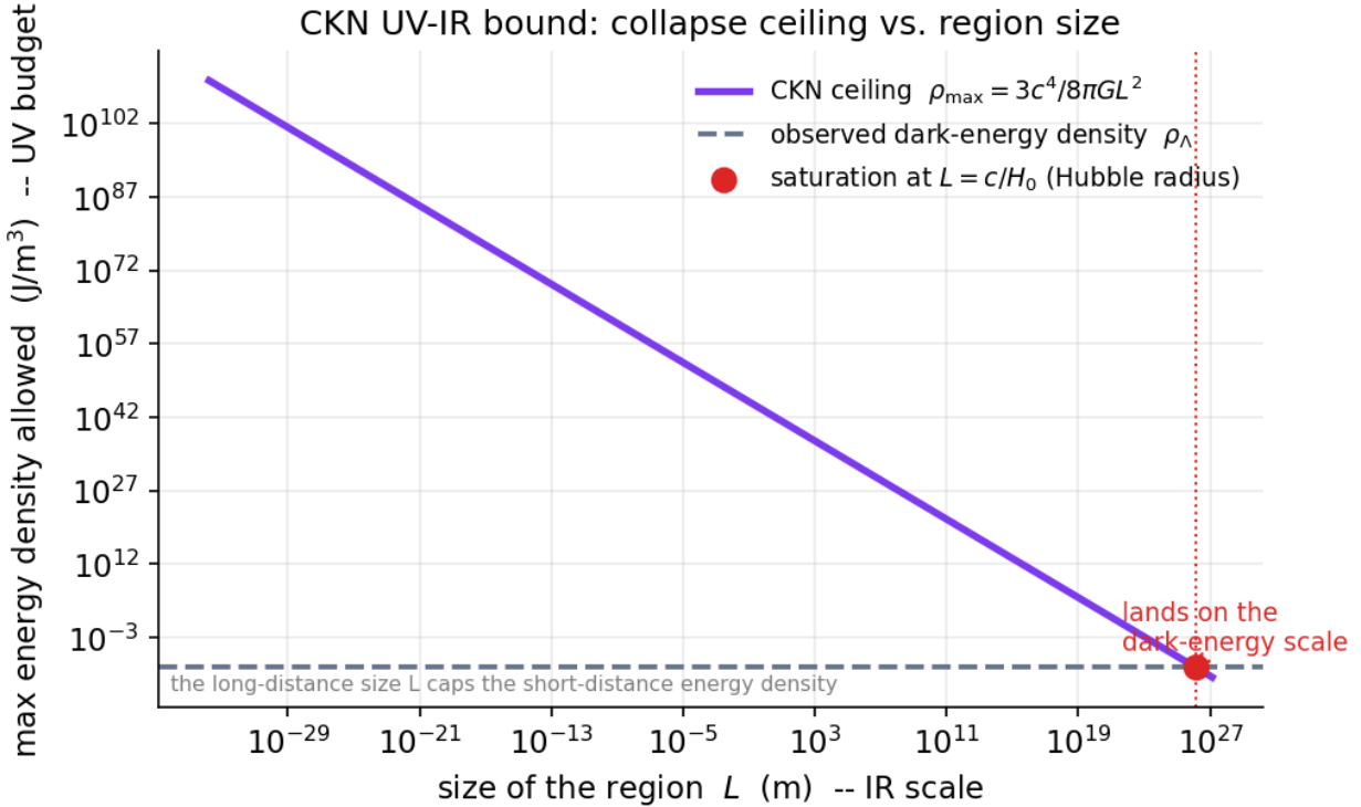
Figure 47: The CKN energy-density ceiling falling as 1/L -squared, saturating at the Hubble radius
