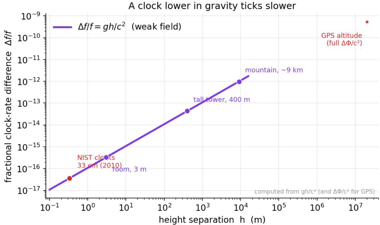
Figure 21: Log-log plot of fractional clock-rate difference gh/c^2 versus height separation, with markers for the 33 cm NIST clocks, a 3 m room, a 400 m tower, a 9 km mountain, and GPS altitude
