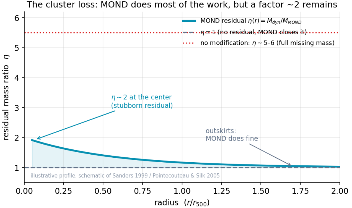
Figure 56: Residual mass ratio \eta plotted against cluster radius, starting near 2 at the center and decaying to 1 in the outskirts, with a dotted line at 5.5 for the unmodified case
