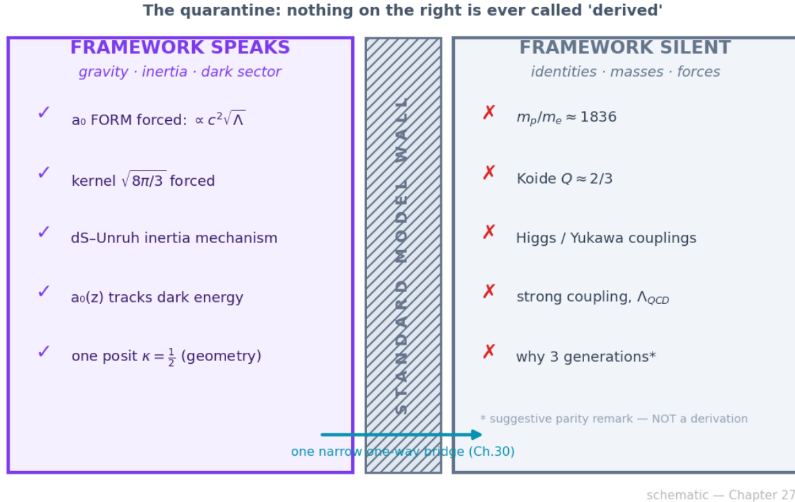
Figure 79: Schematic of the two countries divided by the Standard Model wall
