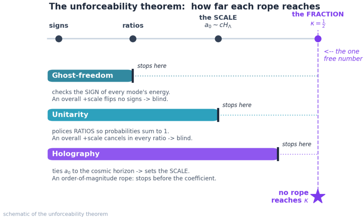
Figure 68: Schematic of three principles as ropes, each reaching part way along a ladder of constrainable quantities and stopping before kappa
