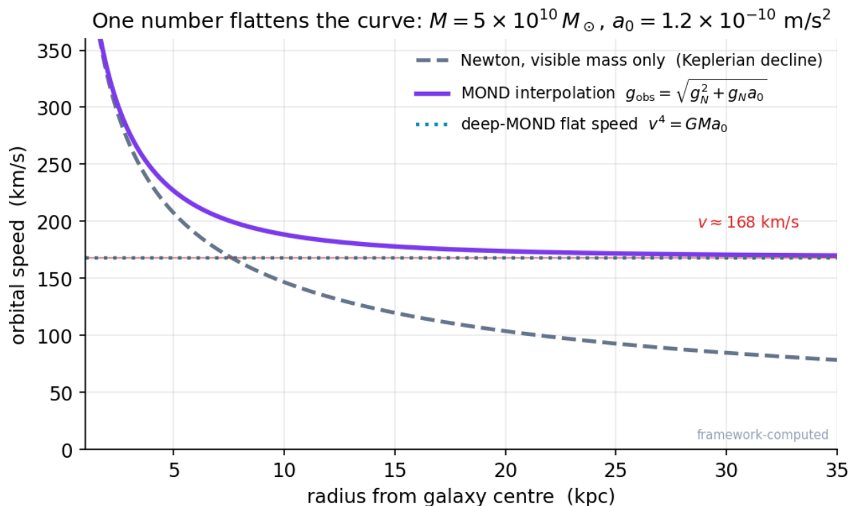
Figure 50: Rotation curve: Newtonian decline versus flat MOND curve
