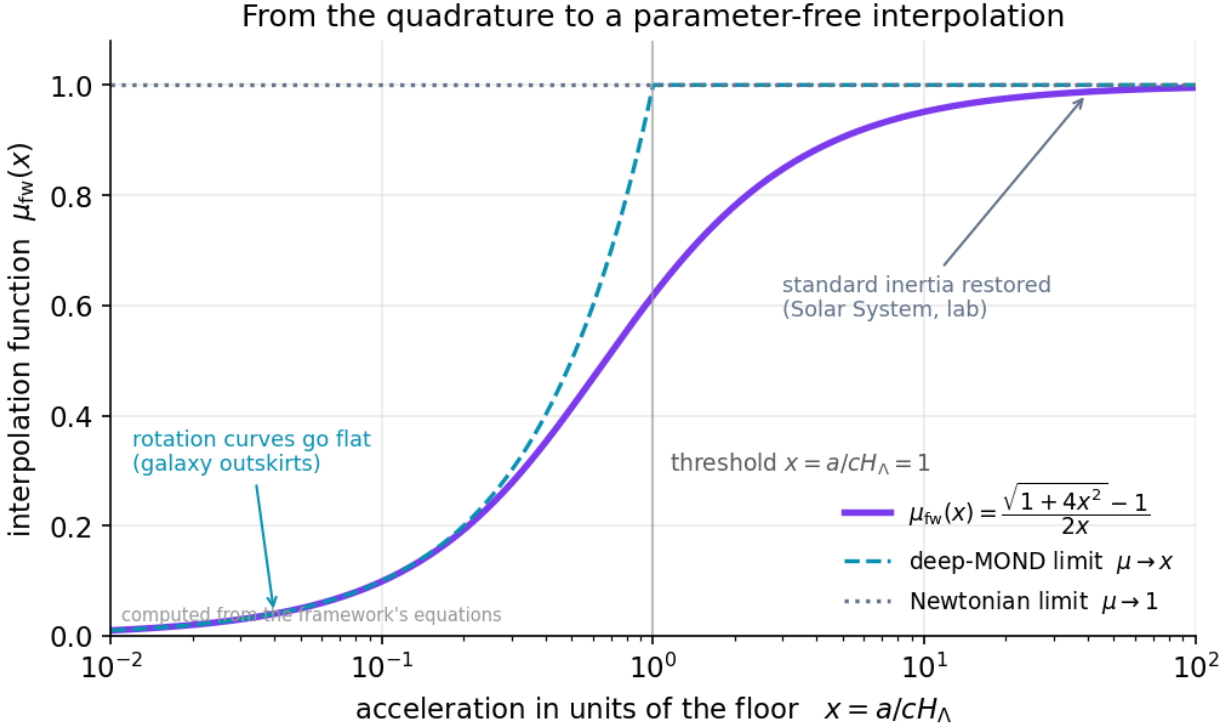
Figure 45: Semi-log plot of the framework interpolation function \mu_{fw} against acceleration in units of the floor, rising from the deep-MOND line toward the Newtonian value of one.
