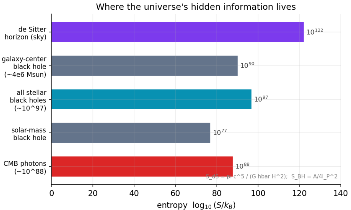
Figure 46: Bar chart of entropies, with the de Sitter horizon at 10^{122} dwarfing all others
