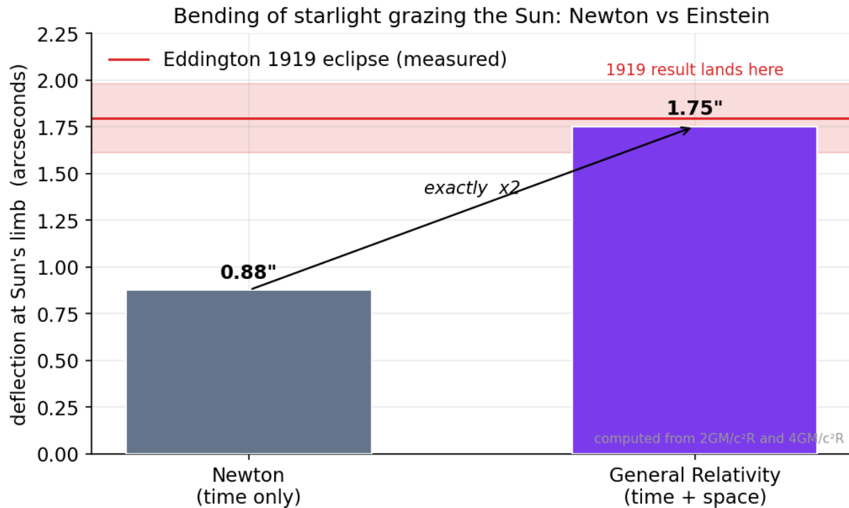
Figure 20: Bar chart of light deflection at the Sun’s limb: Newton 0.875 arcsec versus General Relativity 1.75 arcsec, with the 1919 Eddington measurement band
