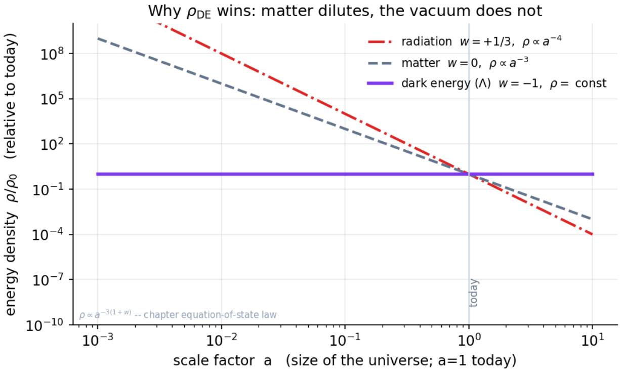
Figure 32: Log-log plot of energy density versus scale factor for radiation, matter and dark energy
