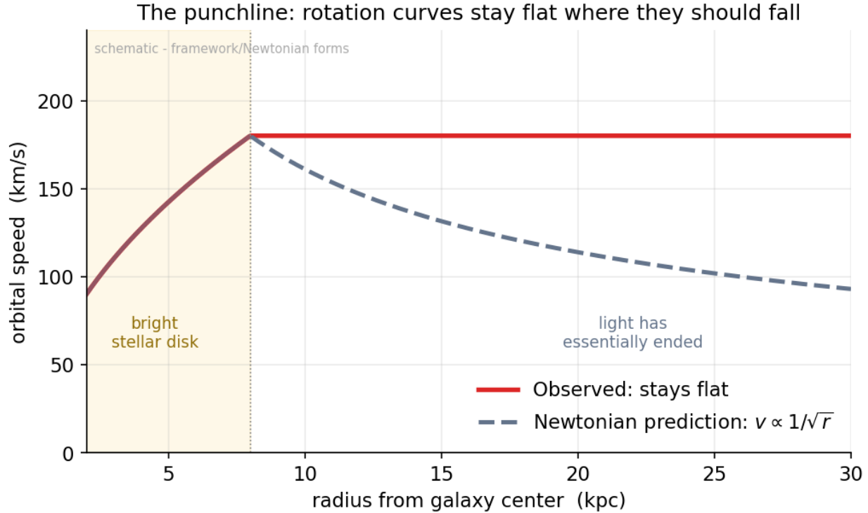
Figure 4: Rotation speed versus radius: a Newtonian curve falling as one over root r past the bright disk, against an observed curve that stays flat.
