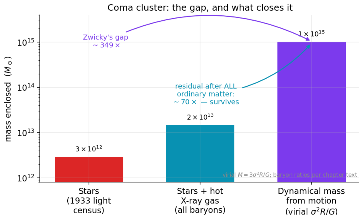
Figure 8: Bar chart comparing the mass of the Coma cluster from light, from stars-plus-gas, and from its motion
