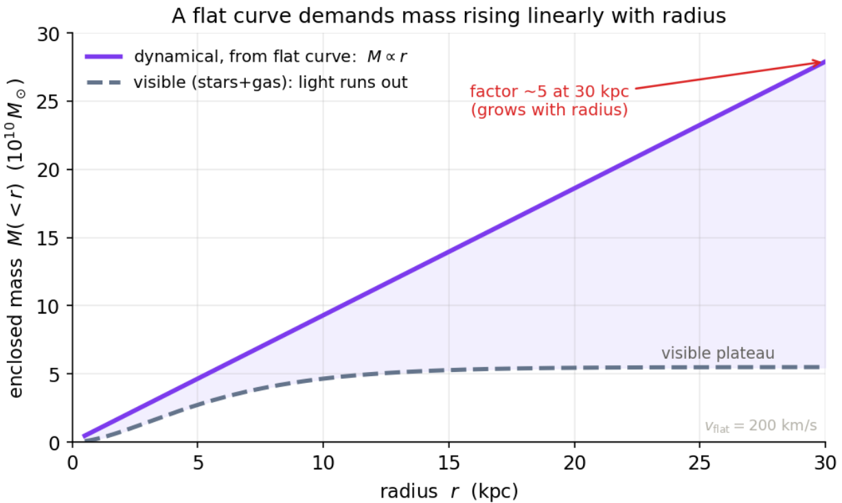
Figure 11: Enclosed mass versus radius: a straight purple line rising linearly from a flat curve, diverging from a grey dashed visible-mass curve that plateaus.
