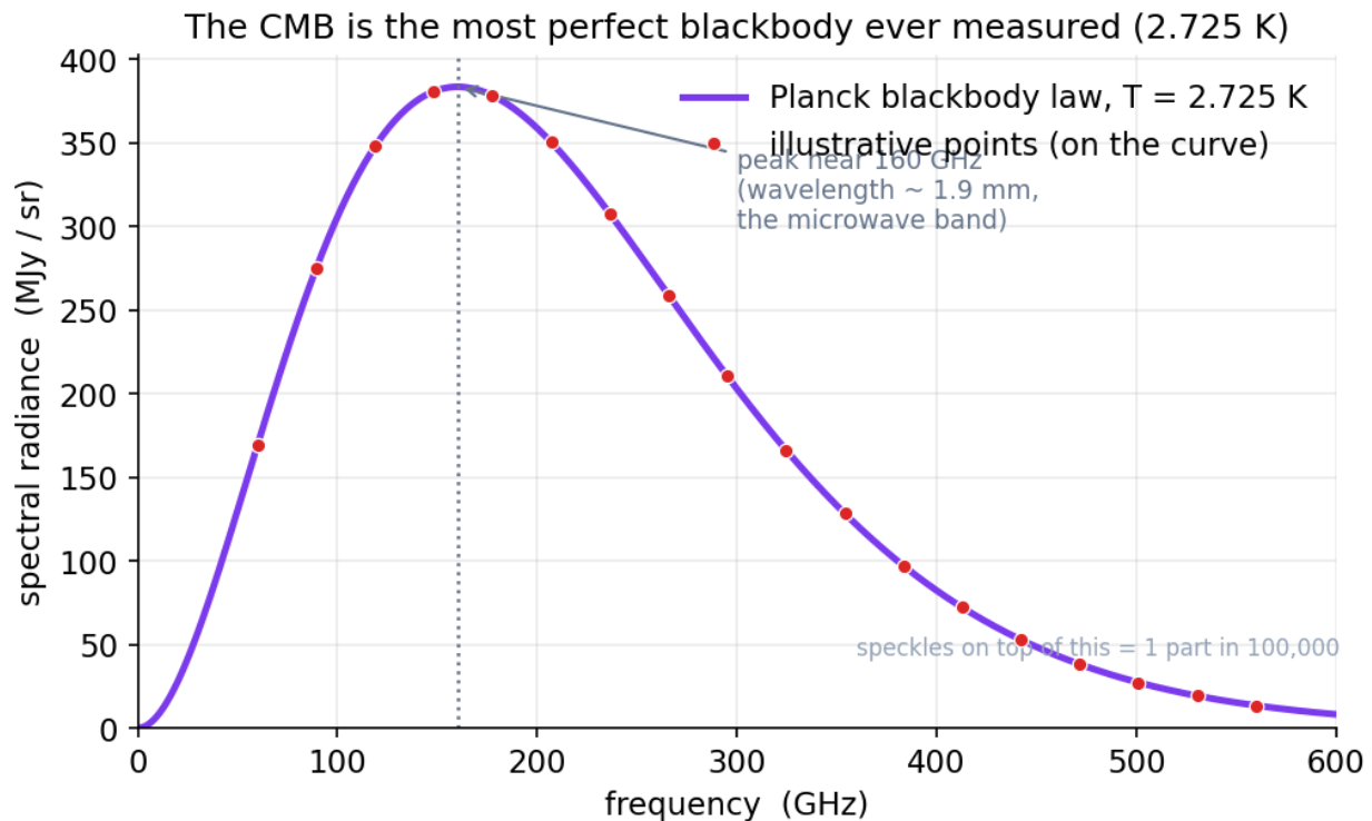
Figure 29: CMB blackbody spectrum at 2.725 K with illustrative points on the curve
