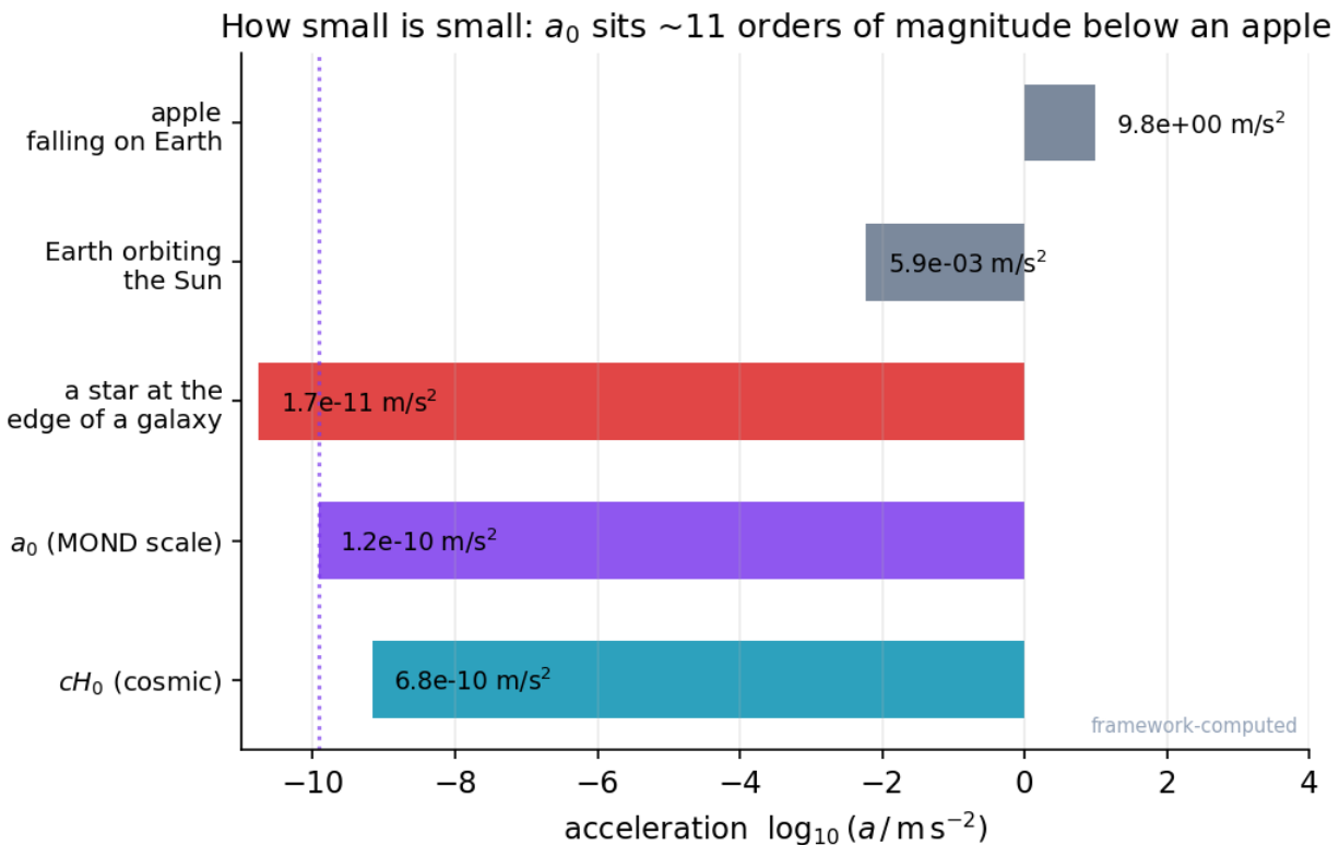
Figure 49: Log ladder of accelerations from an apple down to a_0 and cH_0
