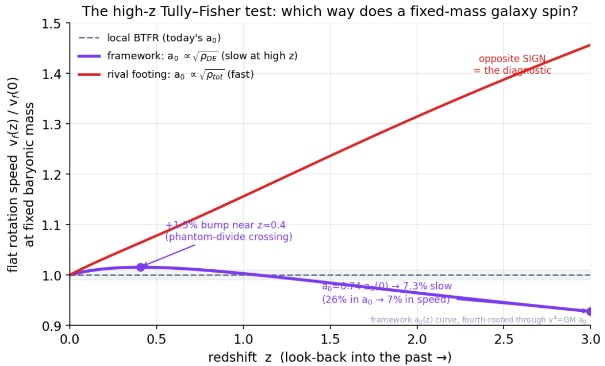
Figure 96: Two curves of rotation speed versus redshift diverging in opposite directions from the local Tully-Fisher line
