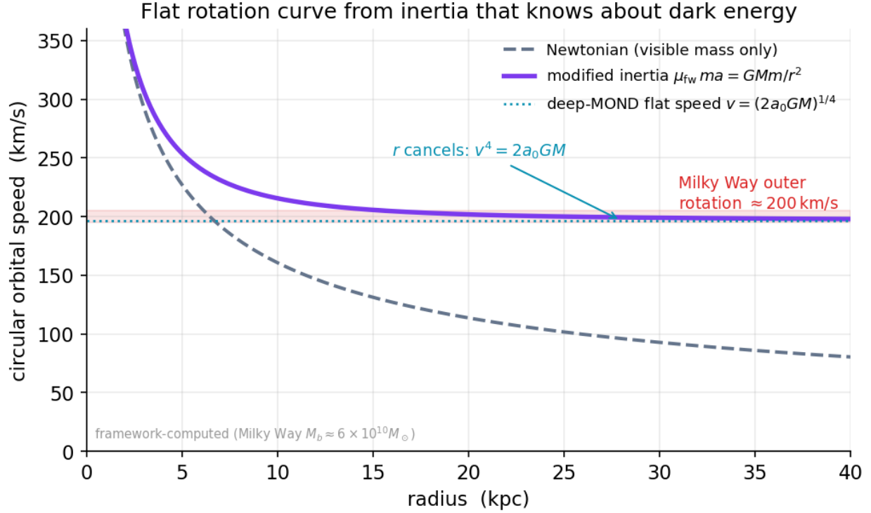
Figure 63: Rotation speed versus radius: the Newtonian curve falls off while the modified-inertia curve flattens to a constant near 200 km per second.
