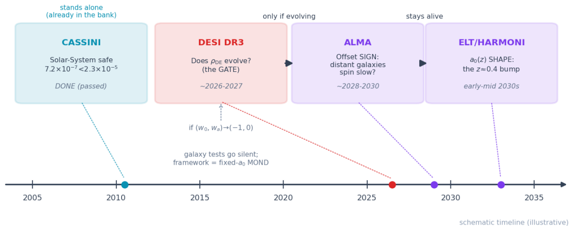
Figure 78: Four labeled test cards — Cassini, DESI DR3, ALMA, ELT/HARMONI — connected by gating arrows above a time axis from 2005 to 2035
