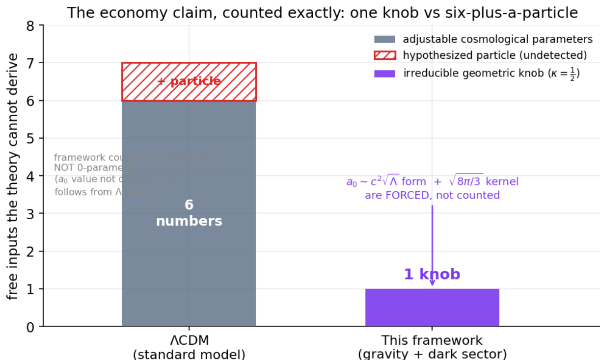
Figure 91: Bar chart comparing free inputs: \Lambda CDM’s six parameters plus an undetected particle versus the framework’s single geometric knob
