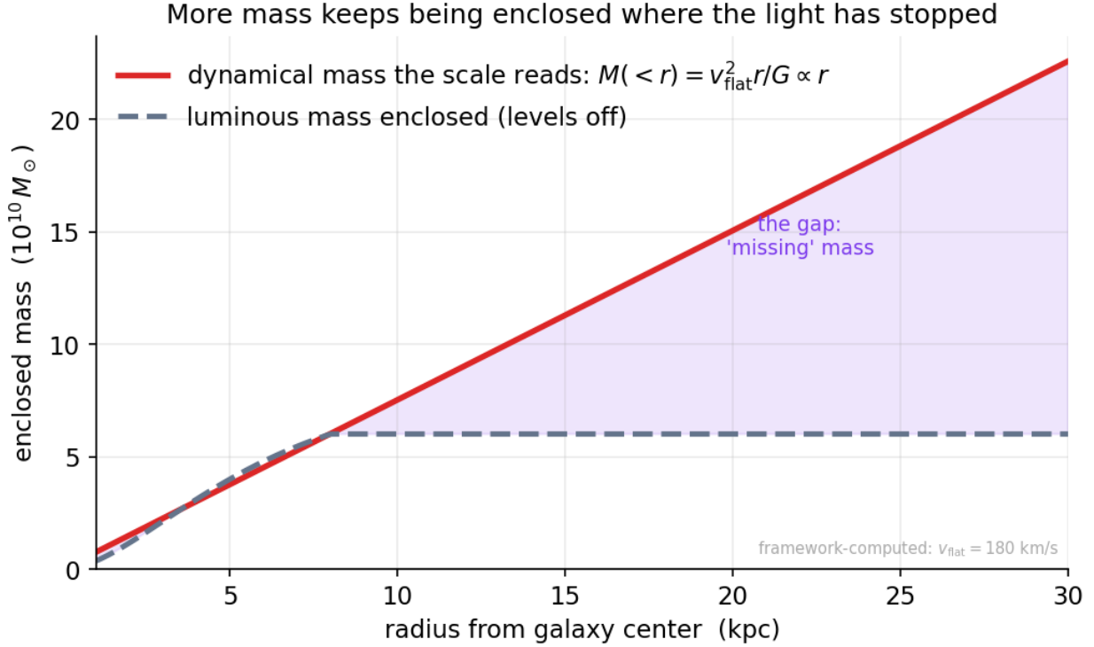
Figure 5: Enclosed mass versus radius: a straight line growing with radius for the dynamical mass, against a luminous-mass curve that flattens, with the widening gap shaded.
