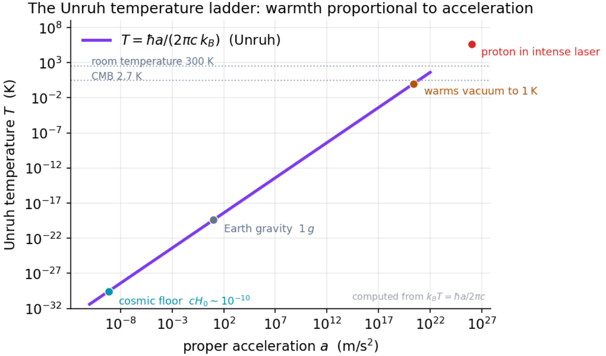
Figure 40: Log-log plot of Unruh temperature versus acceleration with marked scales
