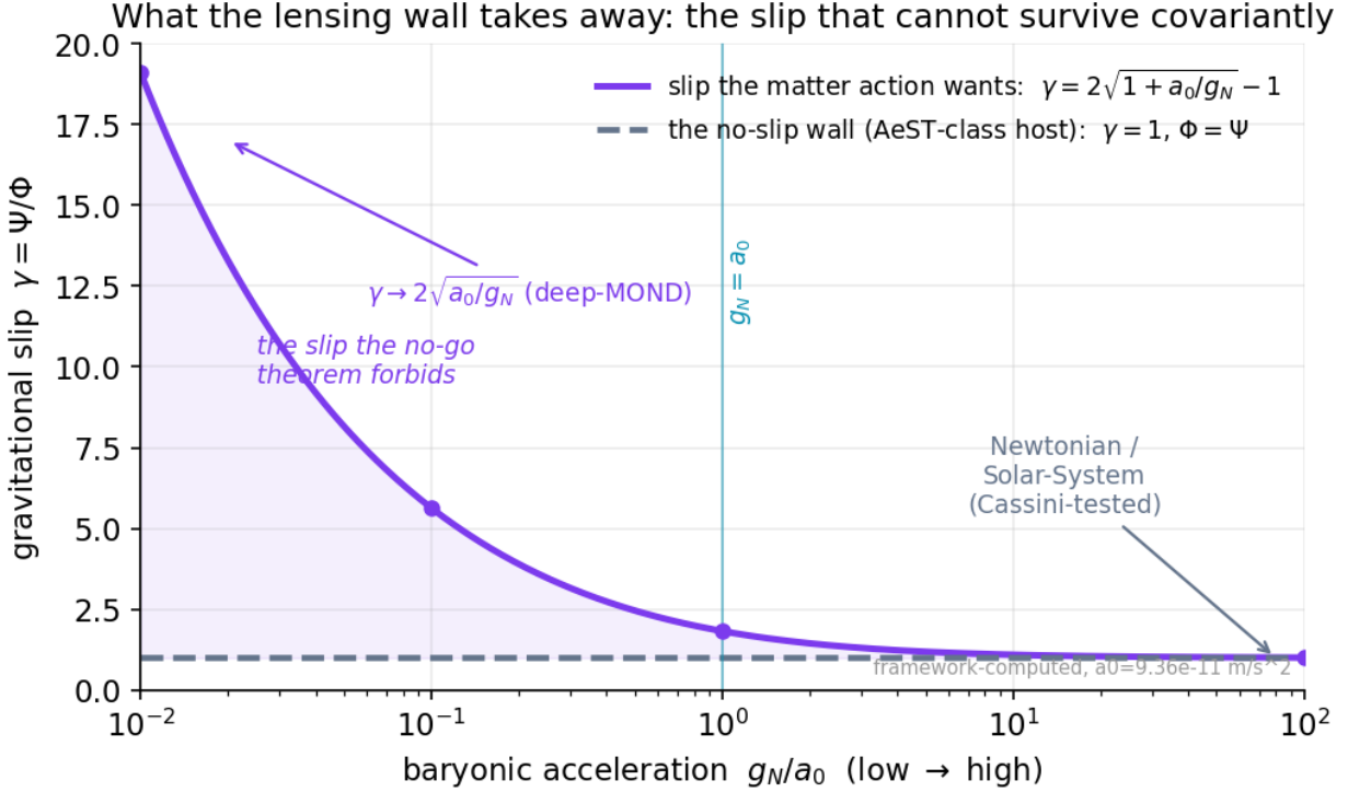
Figure 82: Gravitational slip the framework wants vs the flat no-slip line the theorem forces
