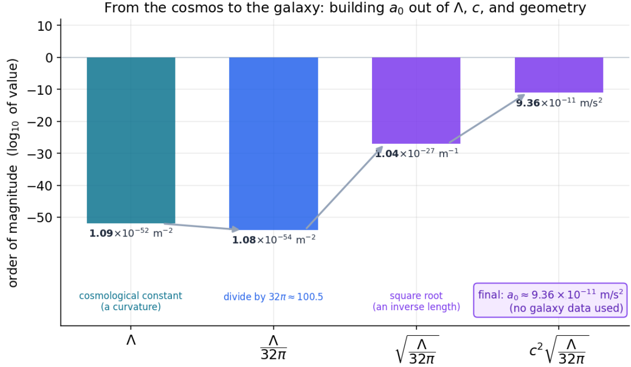
Figure 58: A four-step ladder turning the cosmological constant into the galactic acceleration scale
