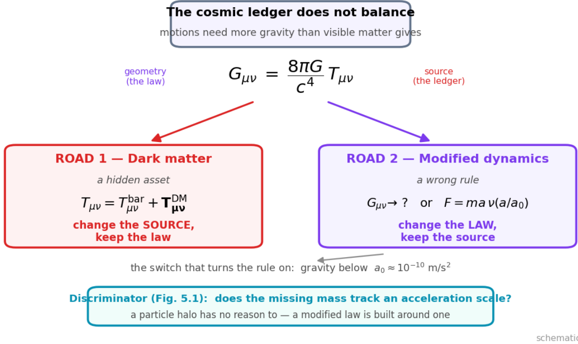
Figure 13: Schematic of the two roads: the Einstein equation forking into dark matter (change the source term T ) and modified dynamics (change the law G or inertia)
