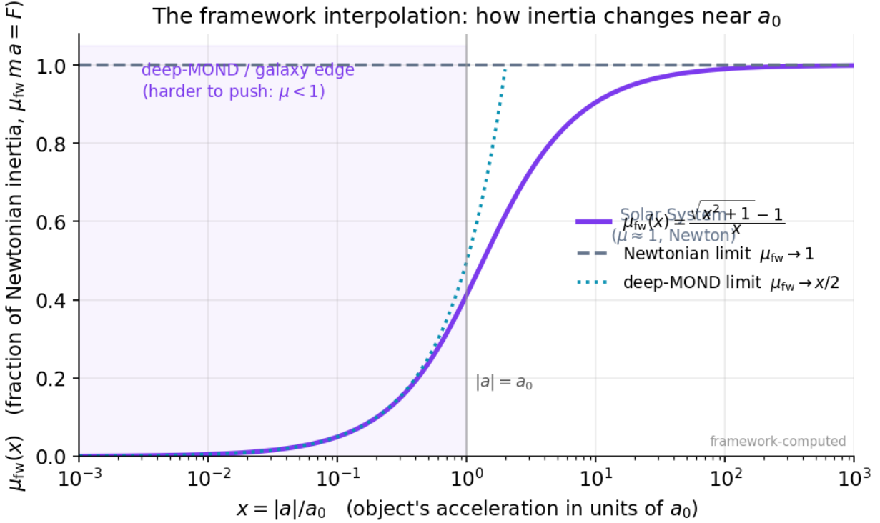
Figure 61: Semi-log plot of the framework interpolation function \mu_{fw} versus acceleration in units of a_0 , rising from the deep-MOND line toward 1.
