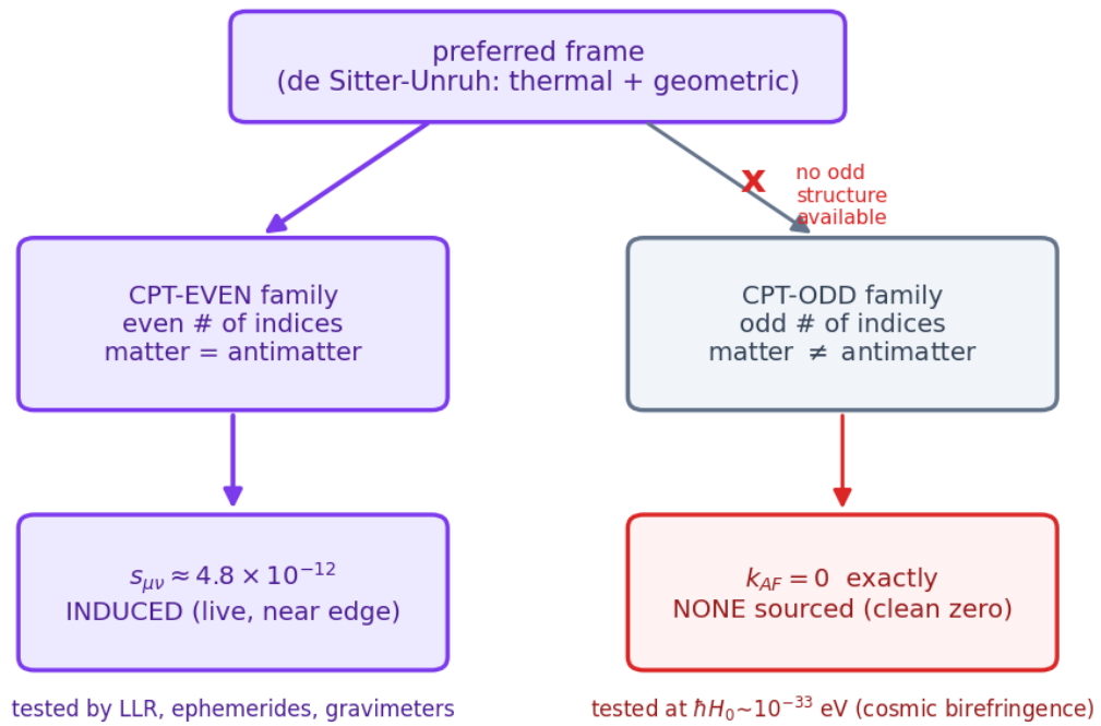
Figure 89: Schematic of the two SME families, with the framework sourcing only the CPT-even branch
