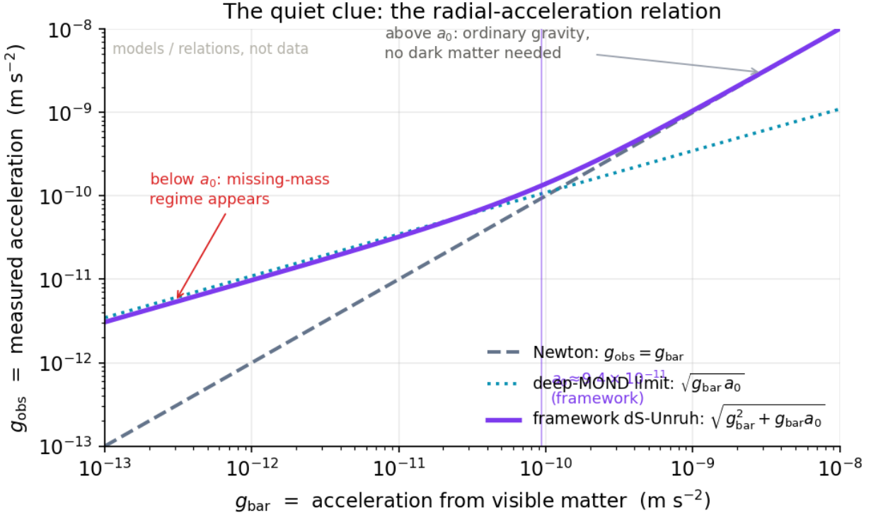
Figure 12: Log-log radial-acceleration relation: a purple framework curve that tracks the Newtonian line at high acceleration and bends to the deep-MOND square-root line below the scale a_0 .
