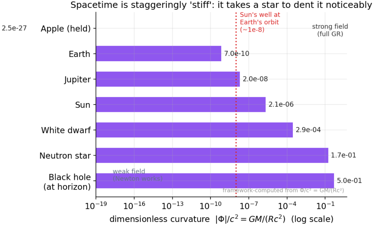
Figure 22: Bar chart of dimensionless spacetime curvature for objects from an apple to a black hole
