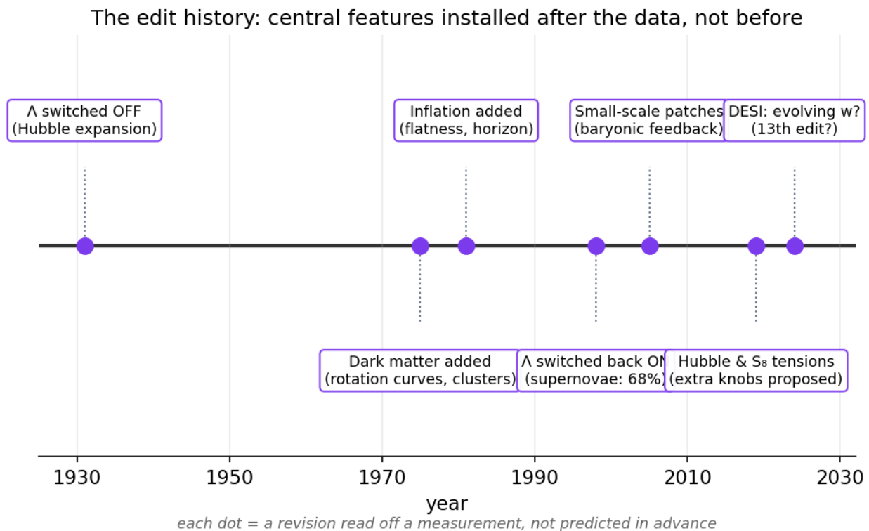
Figure 34: Timeline of seven revisions to the standard cosmological model from 1931 to 2024
