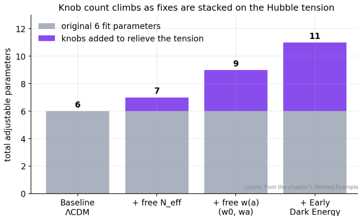
Figure 36: Bar chart of parameter count rising from 6 to 7 to 9 to 11 as fixes are added
