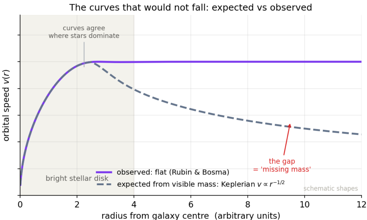
Figure 10: Schematic rotation curves: a grey dashed Keplerian decline versus a purple flat line, agreeing inside the bright disk and diverging beyond it.
