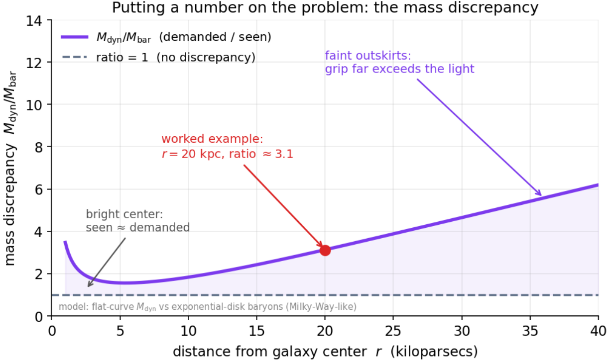
Figure 2: Mass discrepancy ratio climbing with radius
