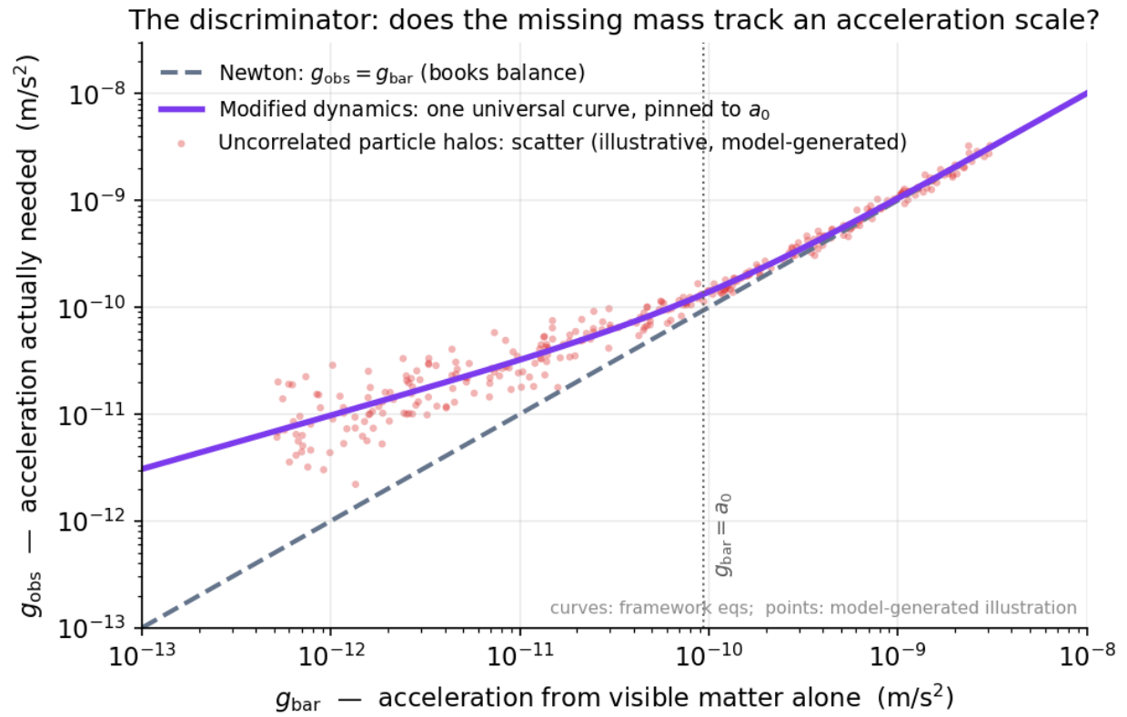
Figure 14: Acceleration plane g_{\text{obs}} versus g_{\text{bar}} : a single tight purple curve pinned to a_0 for modified dynamics, versus scattered red points for uncorrelated particle halos, both meeting the grey Newton line at high acceleration
