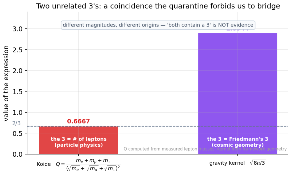
Figure 80: Bar comparison of the Koide Q and the gravity kernel, with their distinct origins of the number three
