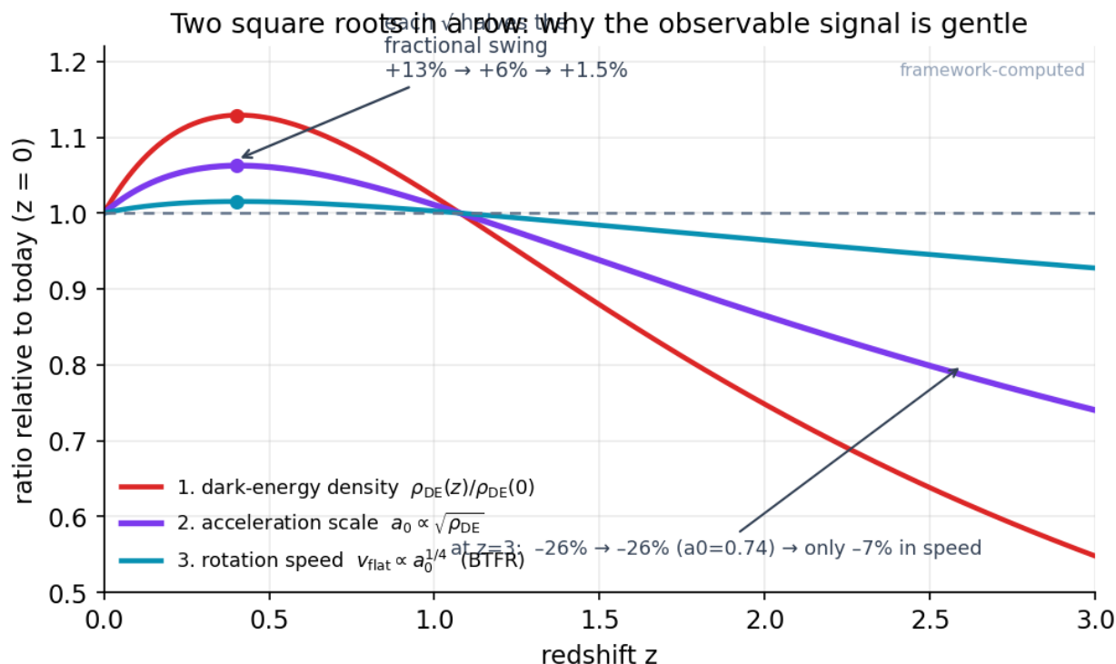
Figure 75: Three nested curves showing the dark-energy density swing shrinking from 13 percent to 6 percent to 1.5 percent as two square roots are applied
