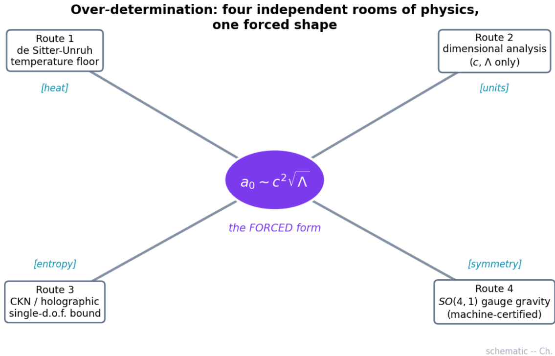
Figure 64: Four arrows from labeled boxes converging on a central node a_0 \sim c^2 \sqrt{\Lambda}
