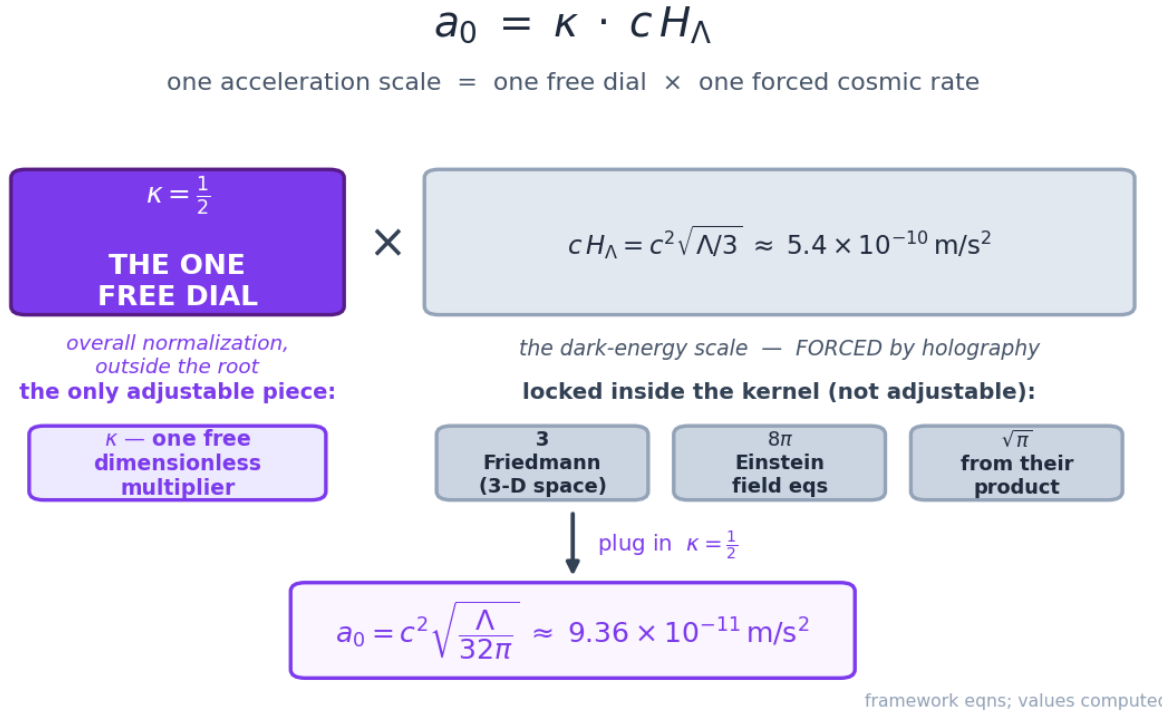
Figure 67: Anatomy diagram of a_0 equals \kappa times c H_\Lambda , with \kappa the one free dial and the kernel pieces locked
