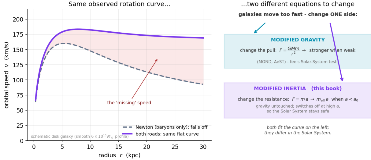
Figure 38: Left: a galaxy rotation curve where Newton falls off but the modified curve stays flat. Right: a fork showing modified gravity versus modified inertia
