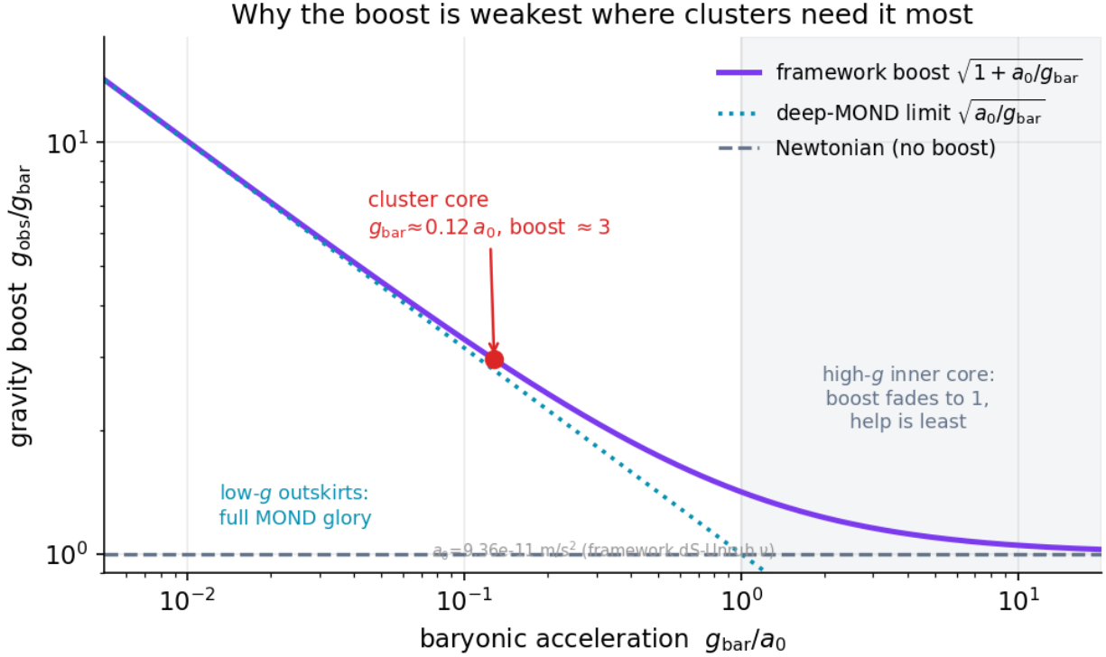
Figure 85: Gravity boost factor versus baryonic acceleration, falling toward 1 at high acceleration
