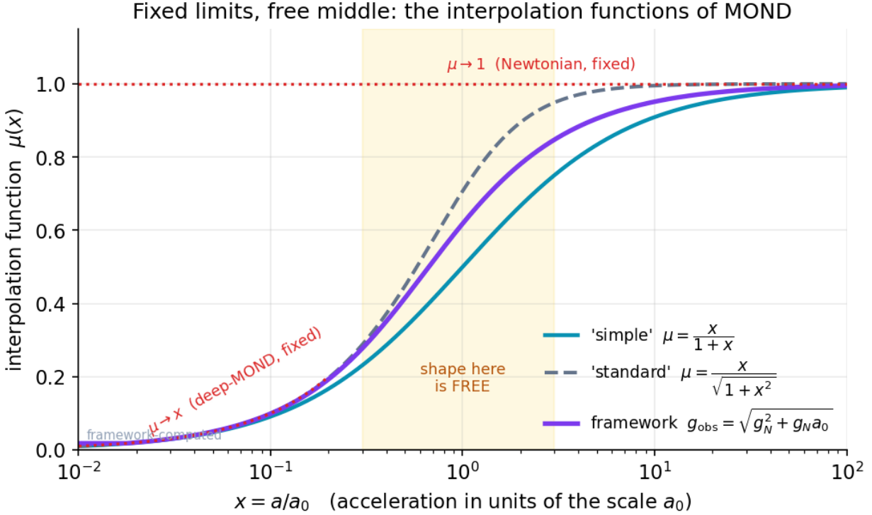
Figure 51: Interpolation functions \mu(x) for simple, standard, and framework forms
