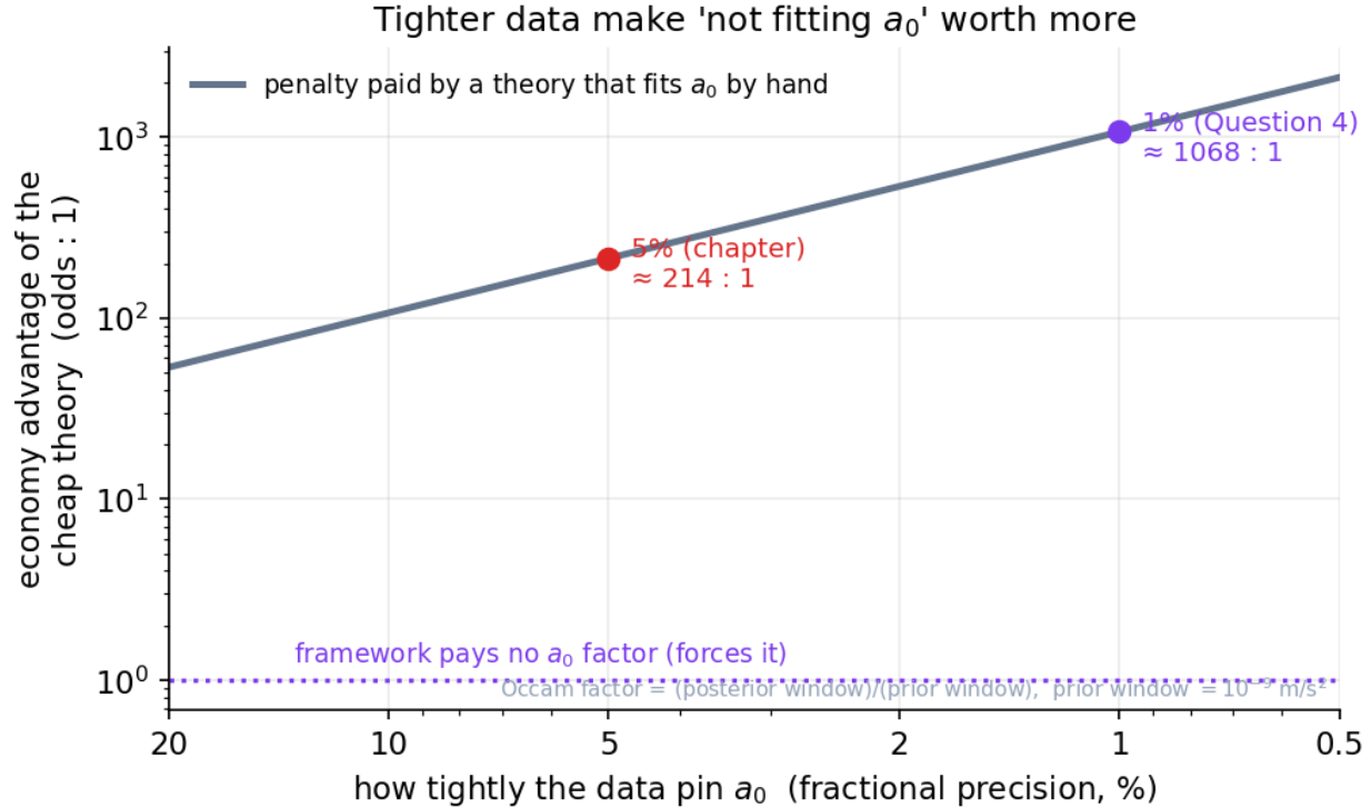
Figure 72: Curve showing the Occam evidence penalty an a_0 -fitting theory pays, growing as the data pin a_0 more tightly
