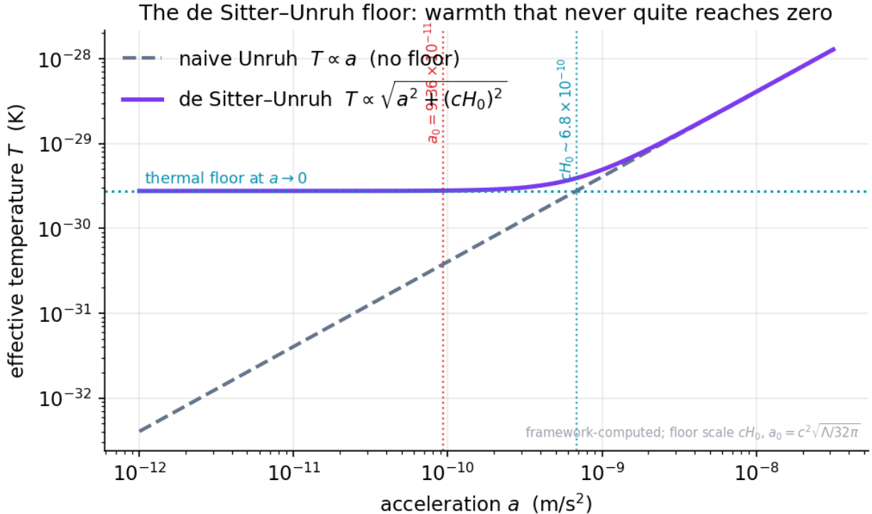
Figure 42: Log-log plot comparing the naive Unruh temperature against the de Sitter–Unruh form that flattens to a floor at low acceleration
