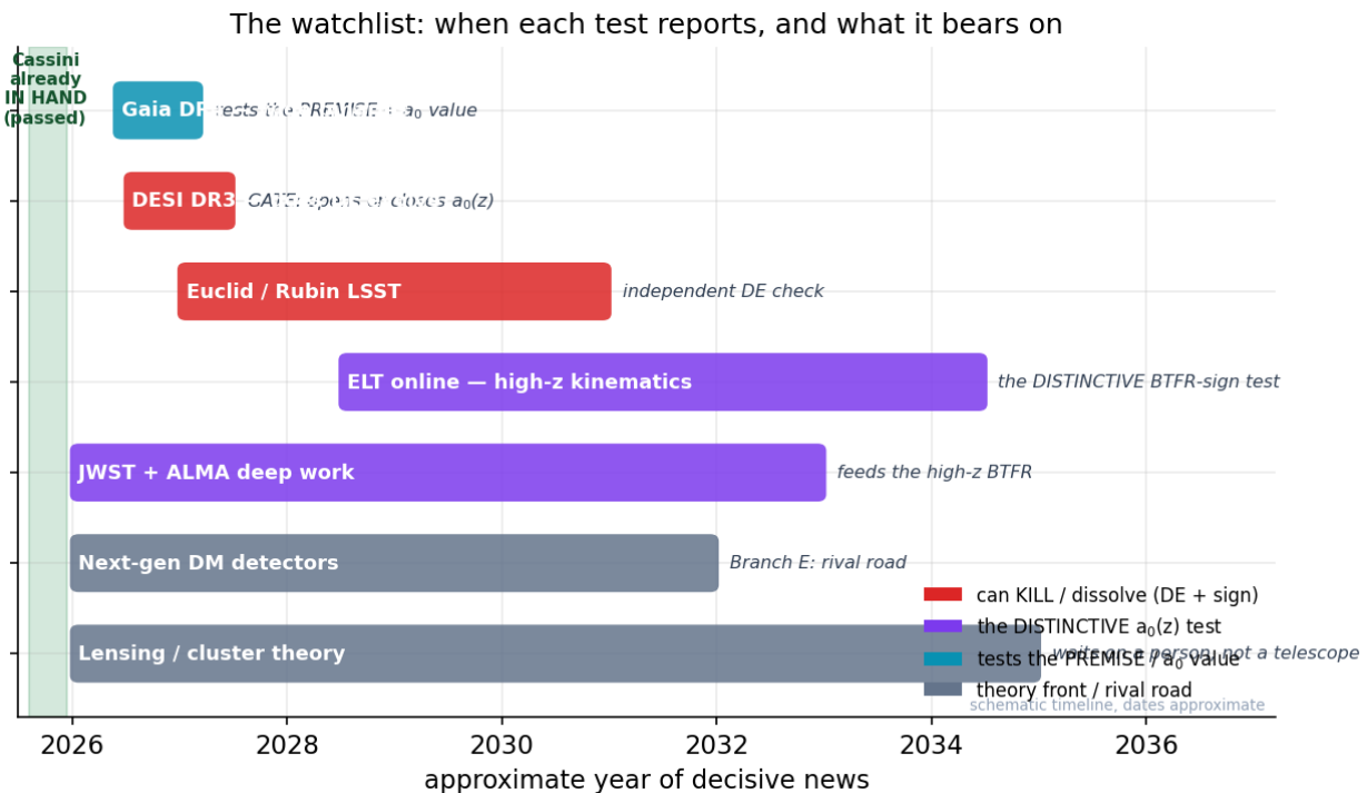
Figure 95: Horizontal timeline of upcoming experiments from 2026 to 2035, colored by what each one tests
