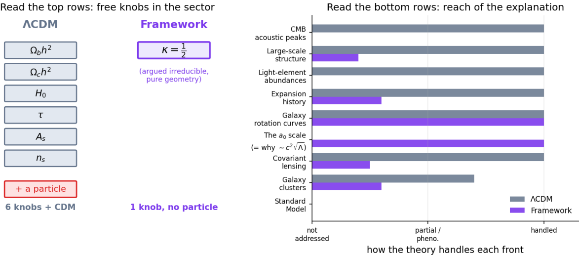
Figure 71: Two-panel scoreboard comparing LambdaCDM’s six parameters plus a dark-matter particle against the framework’s one geometric knob
