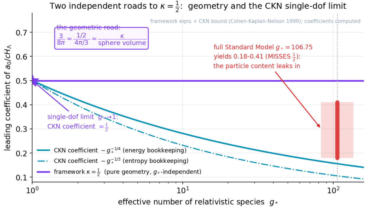
Figure 69: Plot of the CKN coefficient falling with the number of particle species, the framework's flat kappa equals one-half line, and the two roads meeting at the single-dof limit
