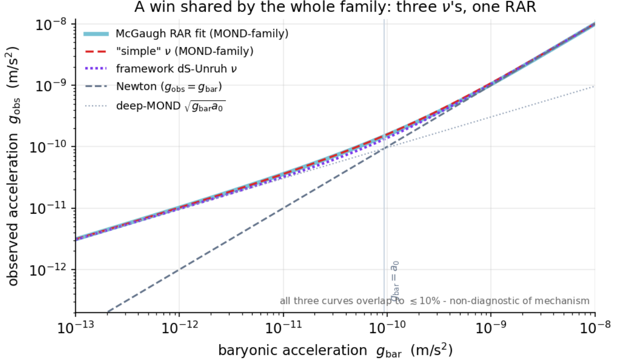
Figure 87: Radial acceleration relation with three nearly-overlapping interpolation curves above the Newtonian line
