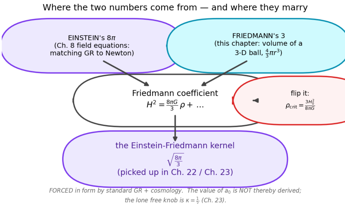
Figure 25: Genealogy diagram tracing Einstein’s 8-pi and Friedmann’s 3 into the Friedmann coefficient and then into the square-root-of-8-pi-over-3 kernel.
