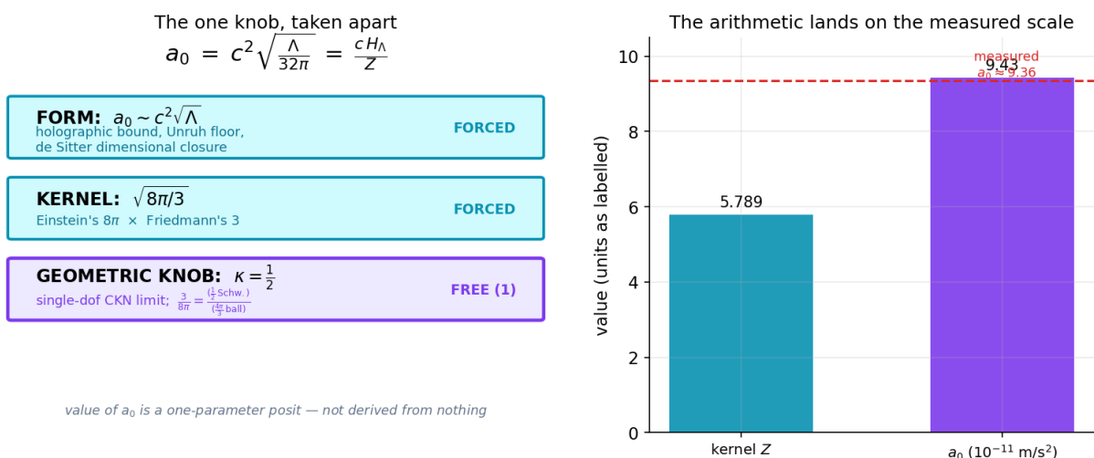
Figure 70: Decomposition of the a_0 formula into forced pieces and the one free geometric knob
