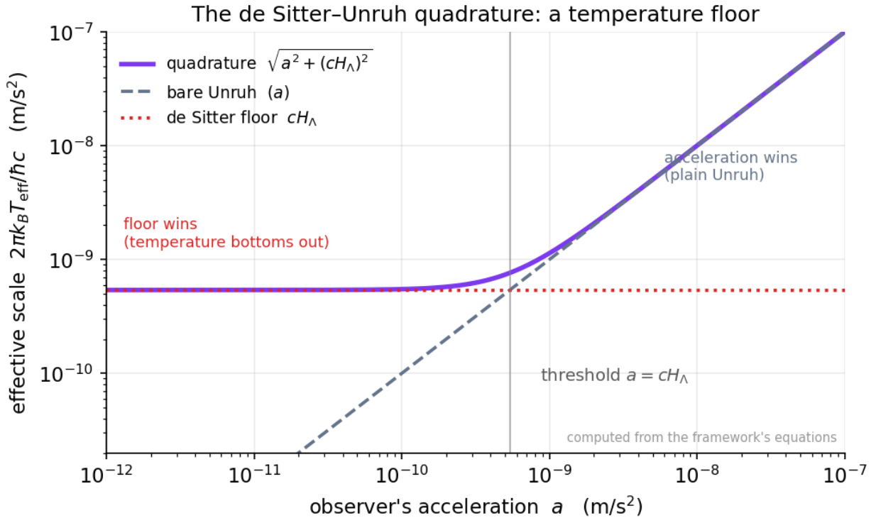
Figure 44: Log-log plot of the de Sitter-Unruh effective acceleration scale versus the observer's acceleration, showing a flat floor at low acceleration and a rising Unruh line at high acceleration.
