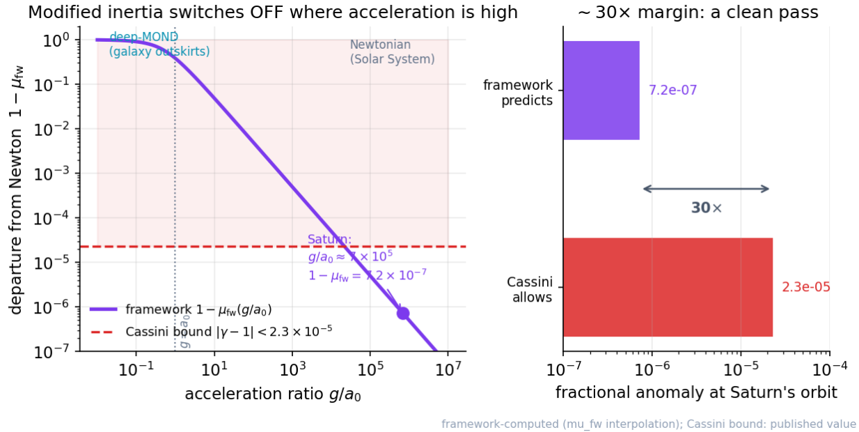
Figure 77: Left: the framework’s departure-from-Newton curve falling steeply with acceleration, Saturn far below the Cassini bound; right: bar chart of predicted versus allowed anomaly
