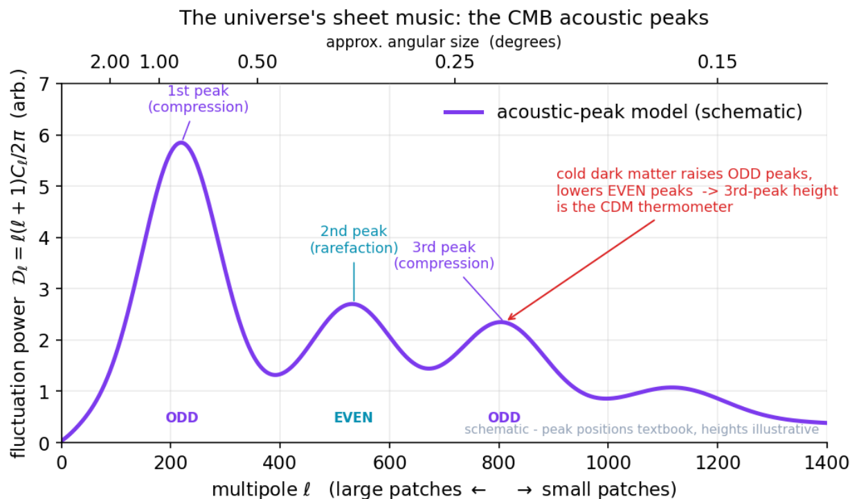
Figure 30: Schematic CMB angular power spectrum showing the acoustic peaks
