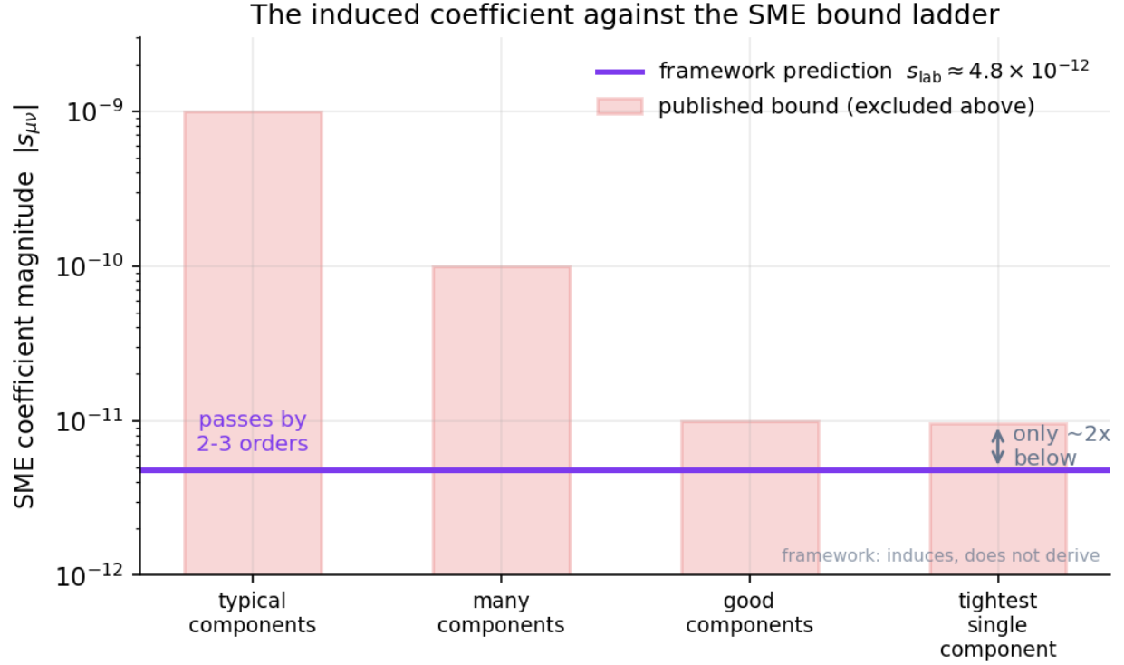
Figure 88: The framework’s predicted SME coefficient plotted against the ladder of published gravitational bounds
