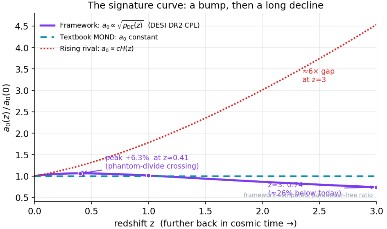
Figure 74: The a_0(z) signature curve rising to a small bump near z=0.4 then declining, against a flat constant-MOND line and a steeply rising rival
