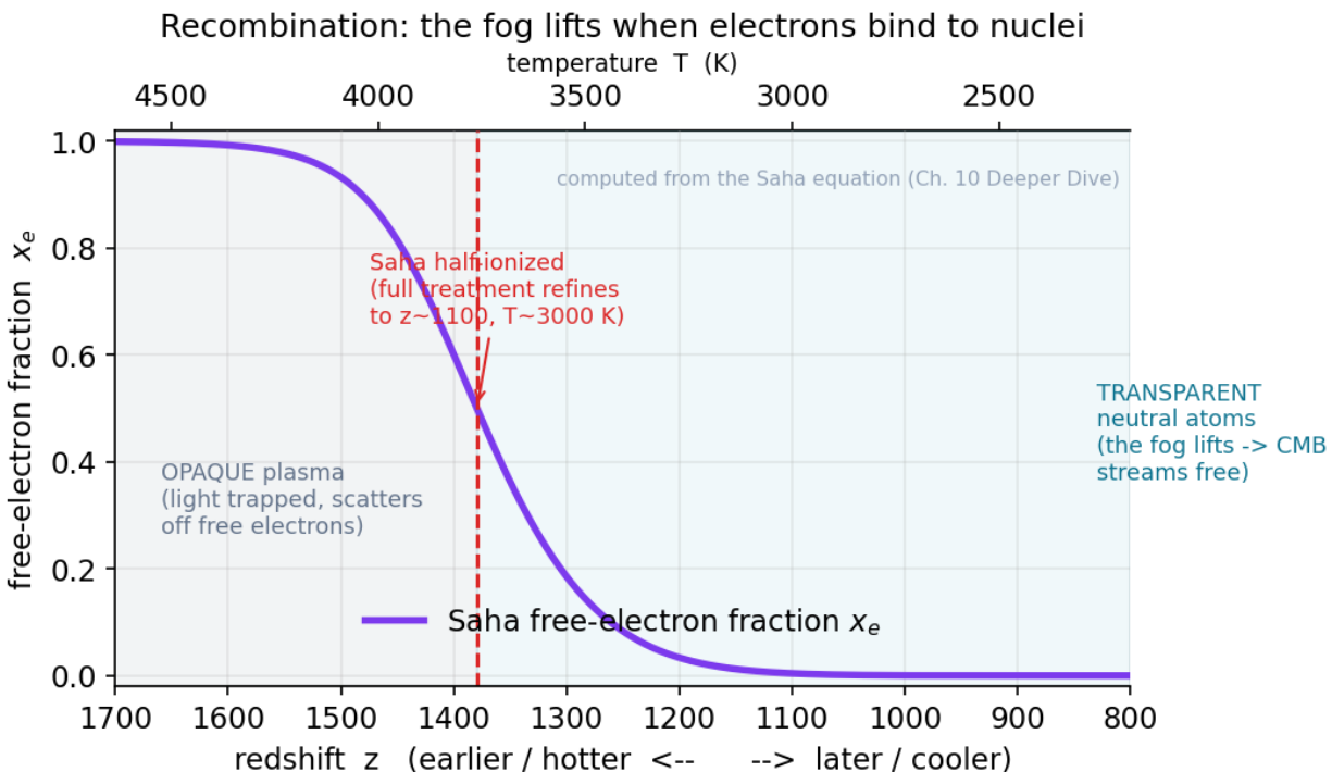
Figure 28: Free-electron fraction versus redshift from the Saha equation, marking recombination
