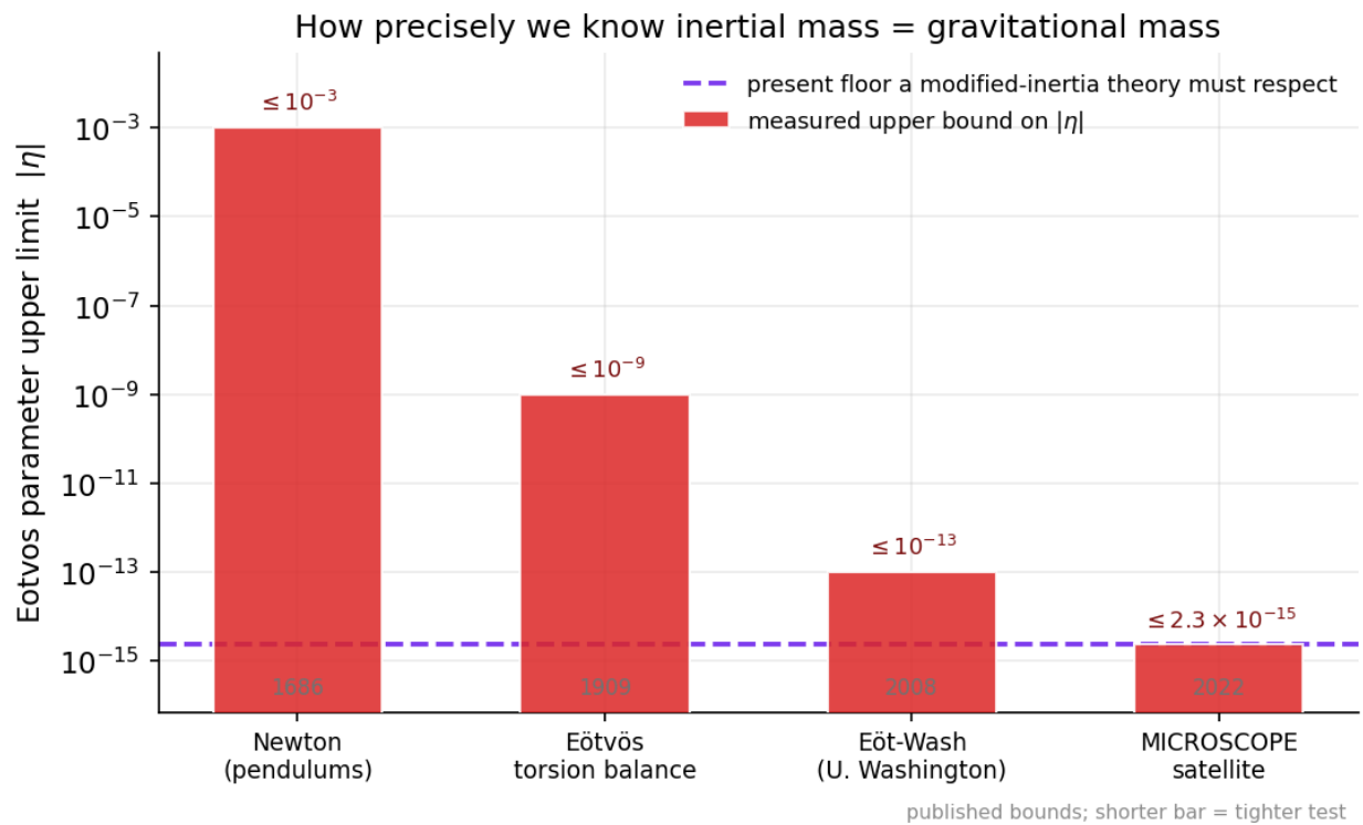
Figure 37: Bar chart of Eotvos-parameter upper limits from Newton to MICROSCOPE, shrinking by twelve orders of magnitude
