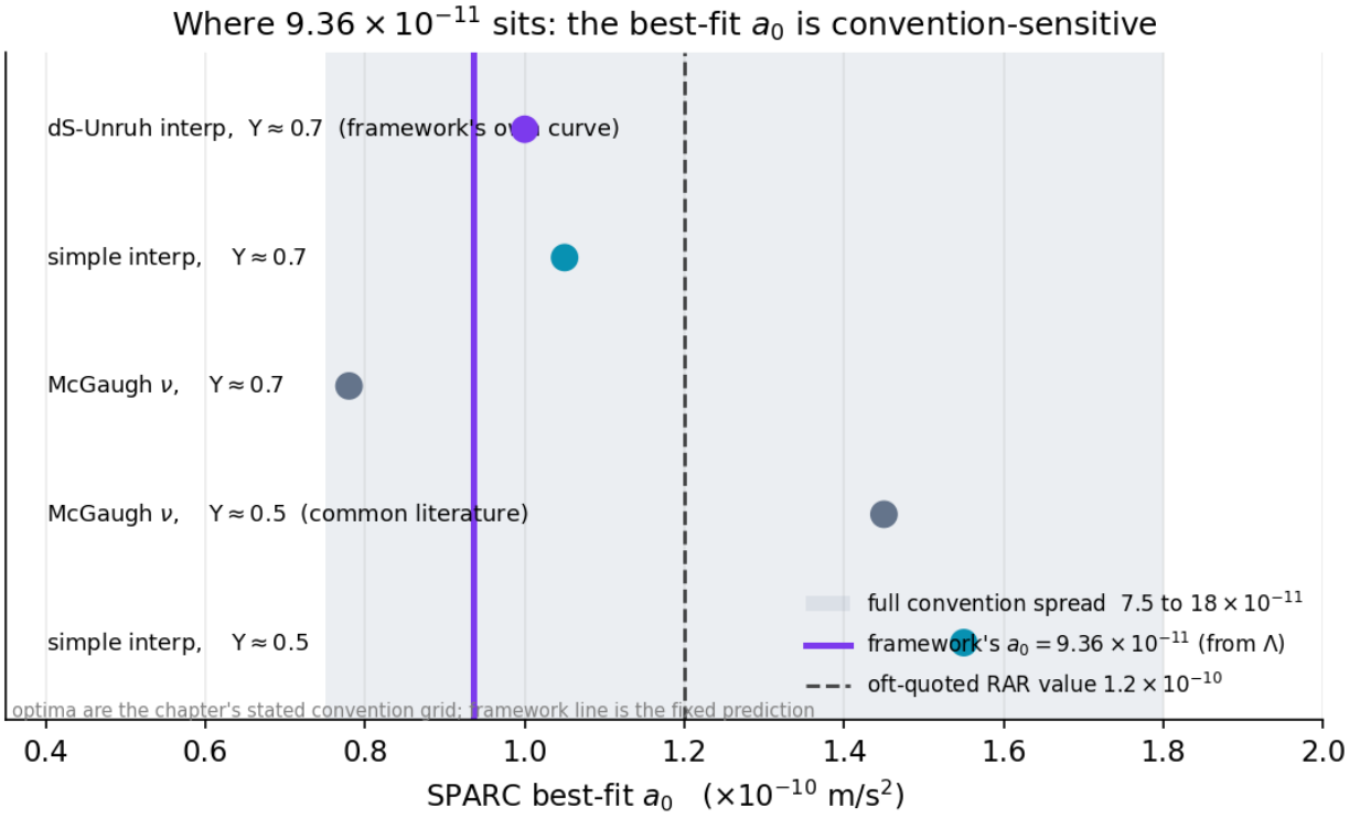
Figure 54: Horizontal spread chart of SPARC best-fit a_0 across five interpolation-and-mass-to-light conventions, with a shaded convention band and a vertical line at the framework's 9.36\text{e-}11 sitting inside it.
