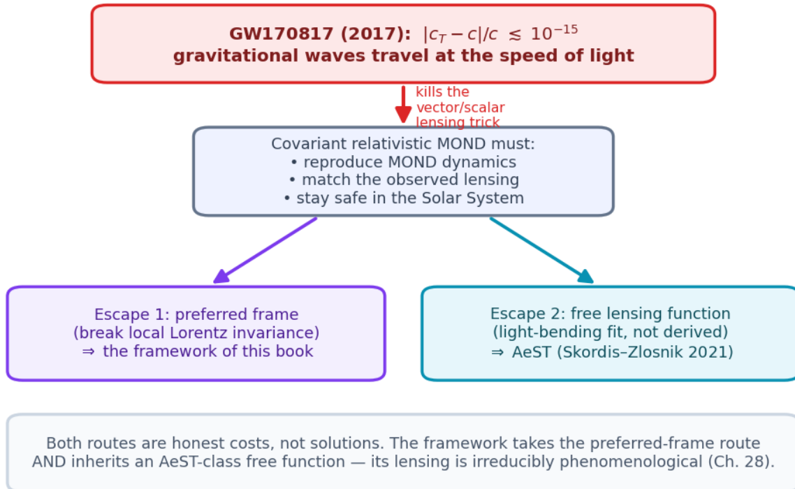
Figure 57: Flow schematic: the GW170817 speed-of-gravity bound kills the lensing trick, leaving two escape routes — a preferred frame (the framework) and a free lensing function (AeST)
