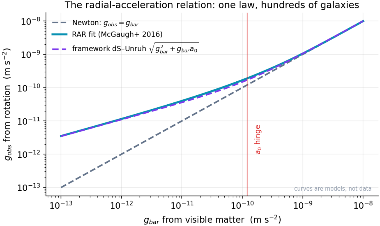
Figure 55: Log-log plot of observed vs baryonic acceleration showing the RAR fit and the framework’s interpolation curving above the Newtonian line below a_0
