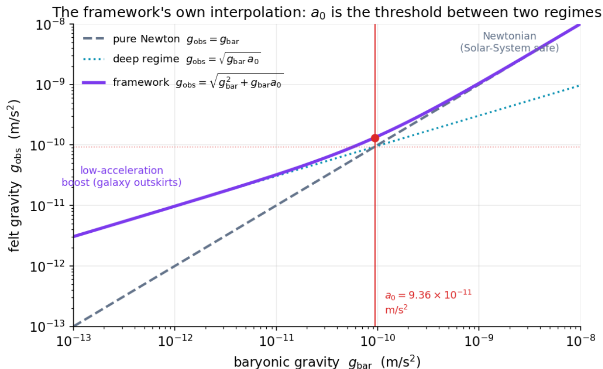
Figure 60: The framework's interpolation curve breaking away from Newton below a_0
