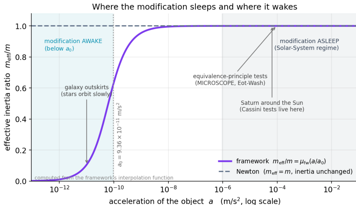
Figure 39: Curve of effective inertia ratio versus acceleration, rising from near zero below a_0 to one above it
