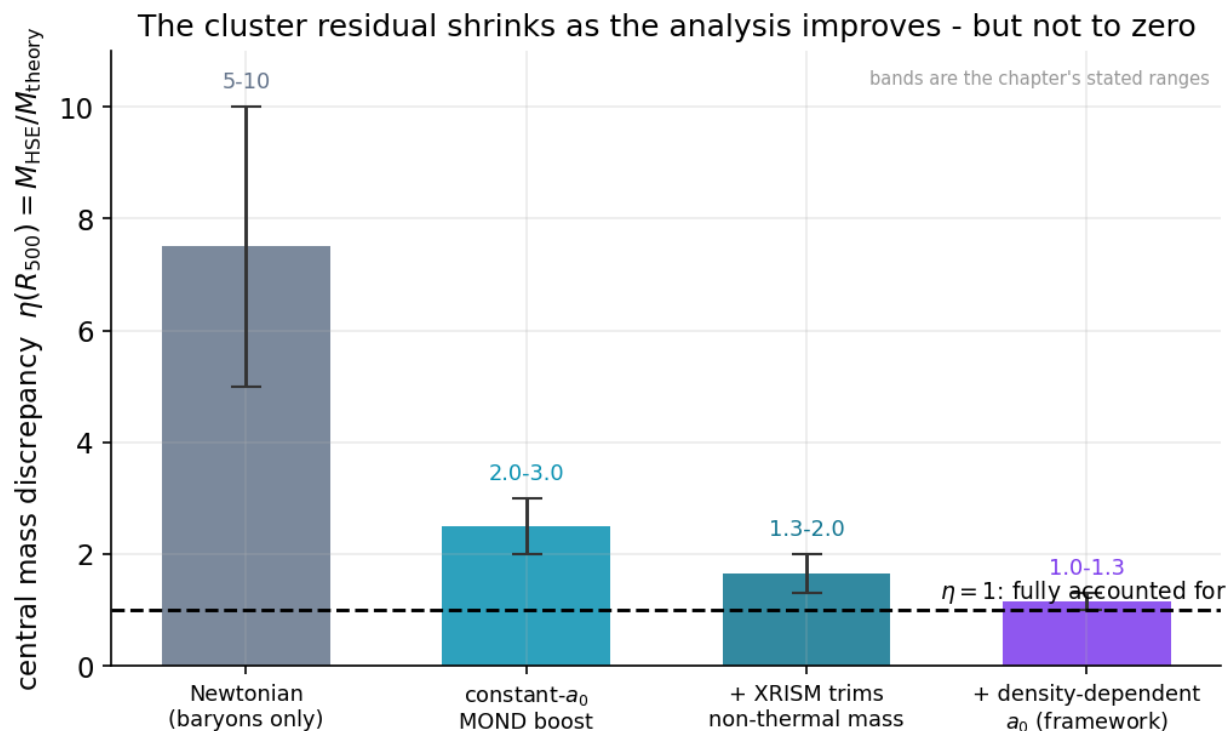
Figure 86: Bar chart of the cluster mass-discrepancy ratio shrinking from about 7 to near 1 across four analysis stages
