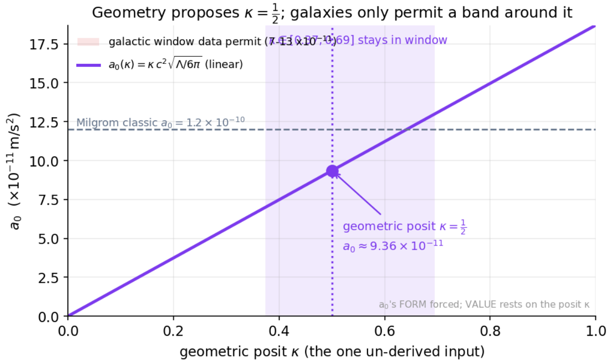
Figure 81: a_0 versus the geometric posit \kappa , with the data-permitted band
