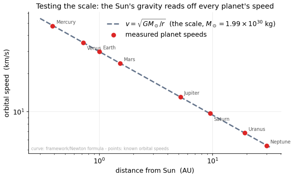
Figure 6: Log-log plot of planet orbital speed versus distance from the Sun; all eight planets sit on the single one-over-root-r scale curve.
