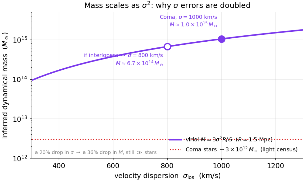
Figure 9: Curve of inferred cluster mass against velocity dispersion, with Coma marked and the interloper question shown
