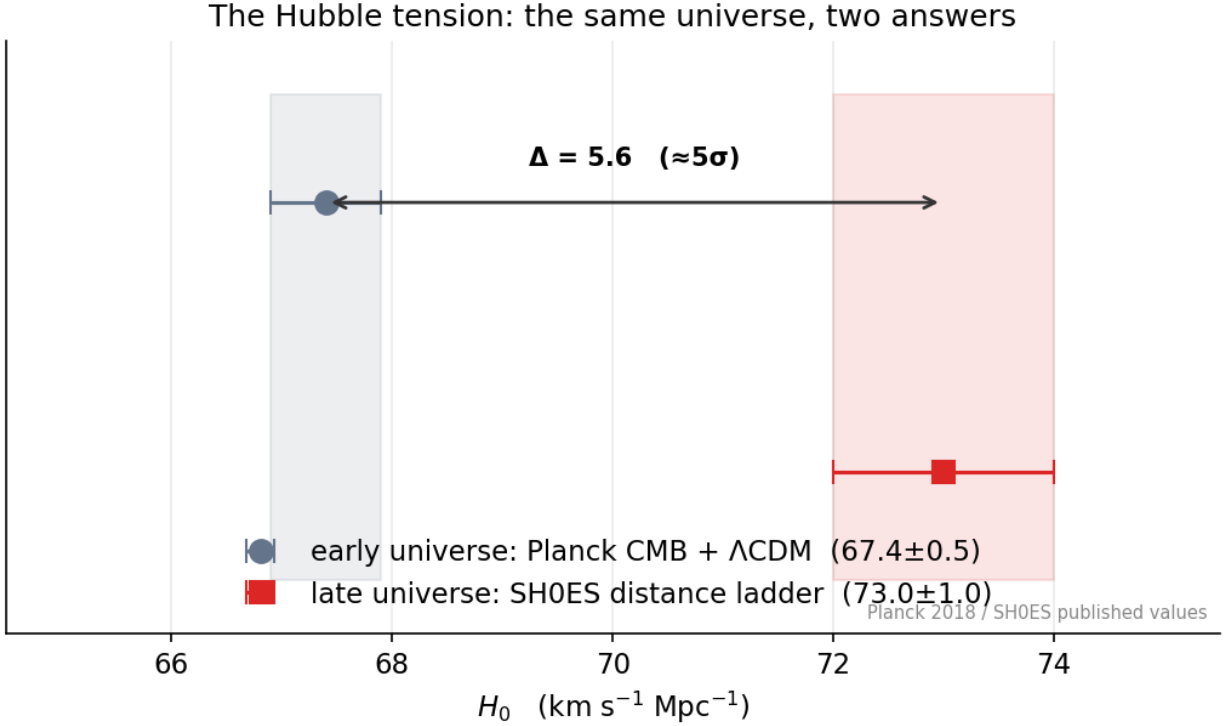
Figure 35: Two measurements of the Hubble constant, near 67 and near 73, with non-overlapping error bars
