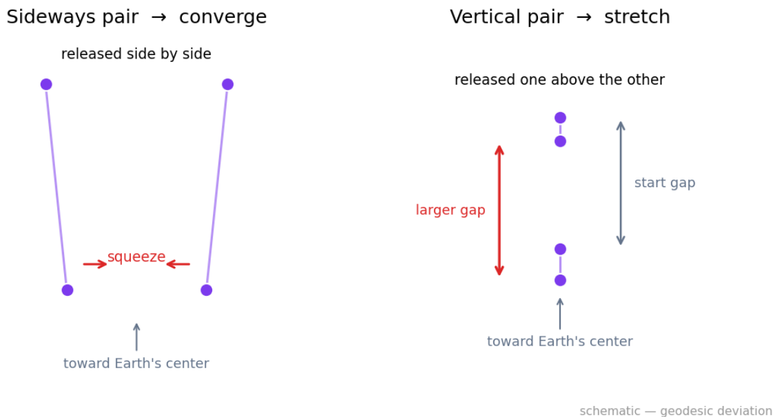
Figure 19: Two-panel schematic: left, two balls released side by side converge as they fall toward Earth's center; right, two balls released one above the other separate vertically
