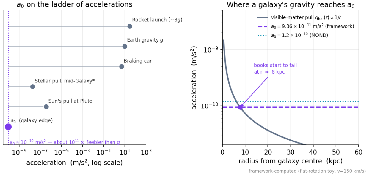
Figure 15: Left: a log ladder of accelerations from rocket launch down to a_0 , showing a_0 about eleven orders of magnitude below Earth gravity. Right: a galaxy's visible-matter pull falling as 1/r and crossing a_0 near 8 kpc
