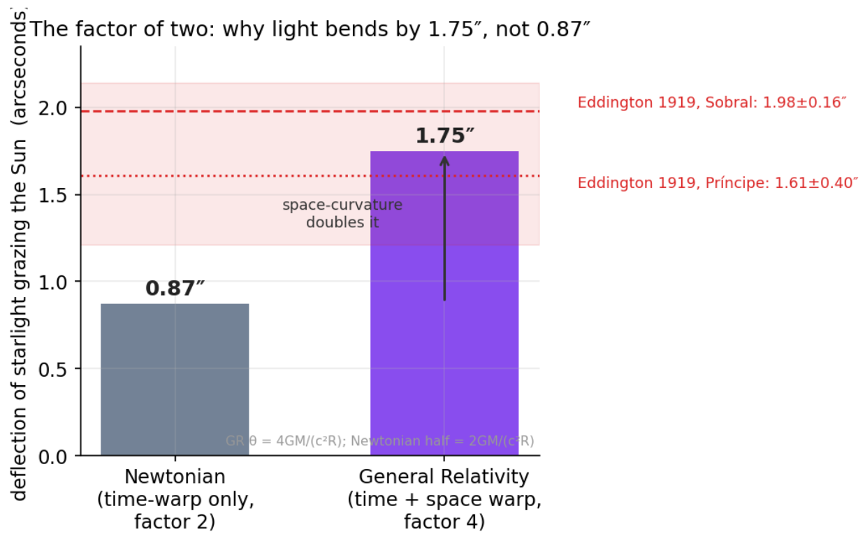
Figure 24: Bar chart comparing Newtonian 0.87 and GR 1.75 arcsecond light bending with the 1919 eclipse band
