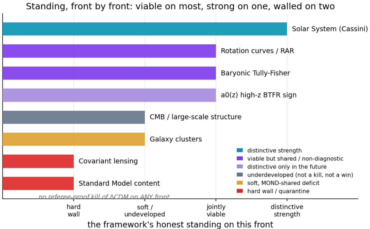
Figure 93: Horizontal scorecard placing eight assessment fronts on an axis from hard wall to distinctive strength, colored by category
