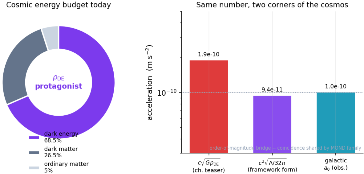
Figure 33: Donut of the cosmic energy budget beside a bar chart bridging \rho_{\text{DE}} to the galactic a_0
