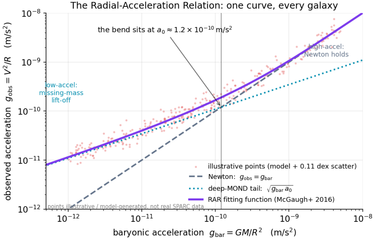
Figure 52: Radial-acceleration relation: observed vs baryonic acceleration on log-log axes, hugging the Newtonian diagonal at high acceleration and lifting onto a square-root tail at low acceleration, with the bend marked at a_0 .
