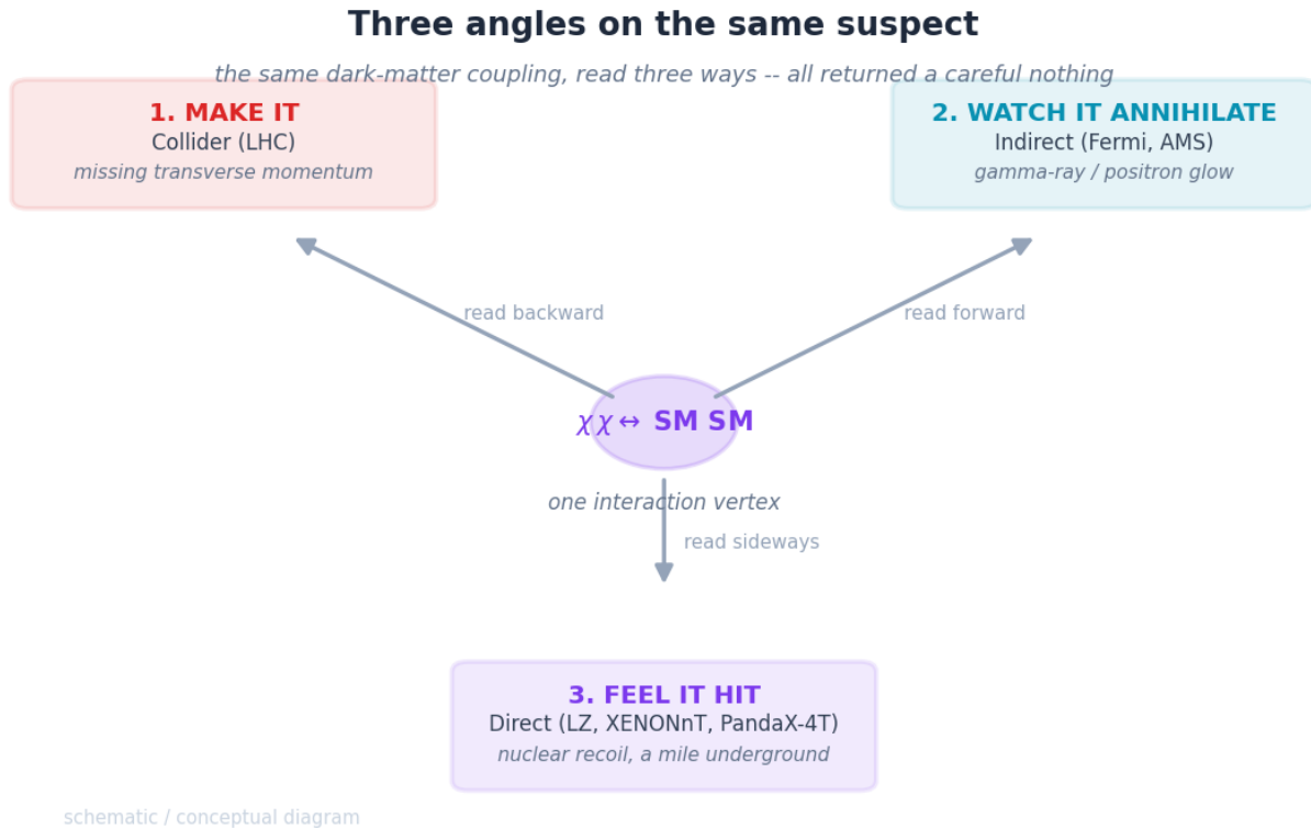
Figure 17: Conceptual diagram: a central dark-matter interaction vertex with three arrows reading it as collider production, indirect annihilation, and direct nuclear recoil
