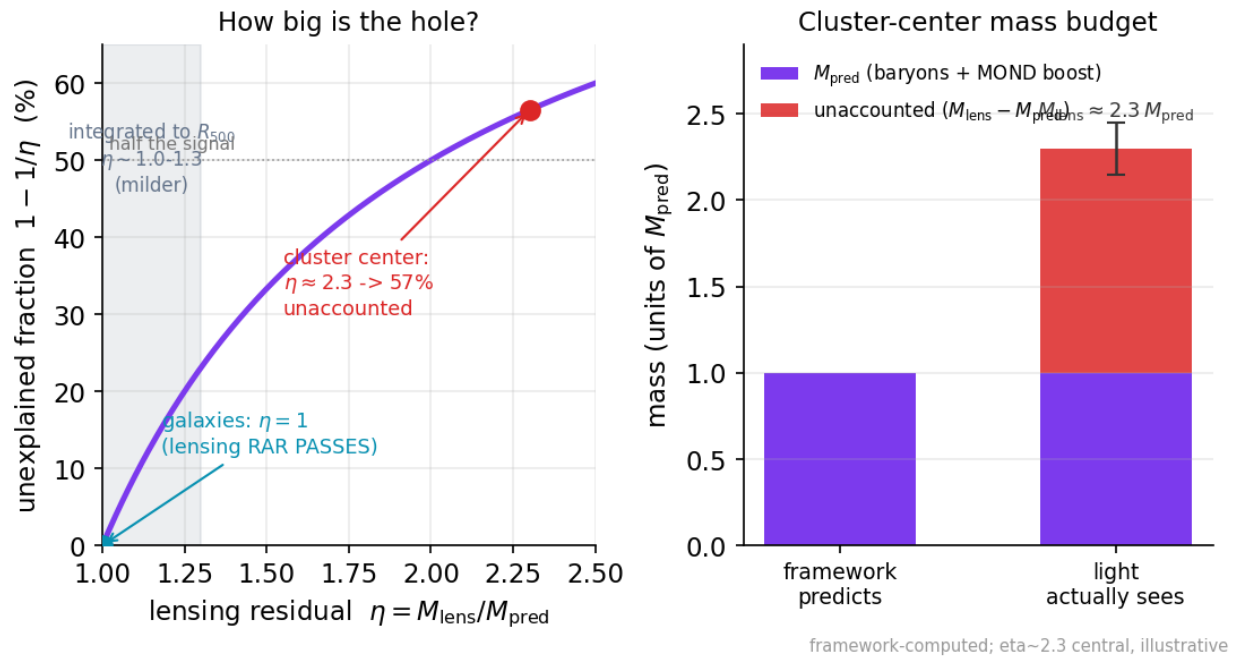
Figure 84: Left: the unexplained lensing fraction rising with the residual eta, with galaxy, integrated-cluster, and central-cluster points marked; right: a mass-budget bar showing the framework predicting M_{\text{pred}} and light seeing 2.3 times more
