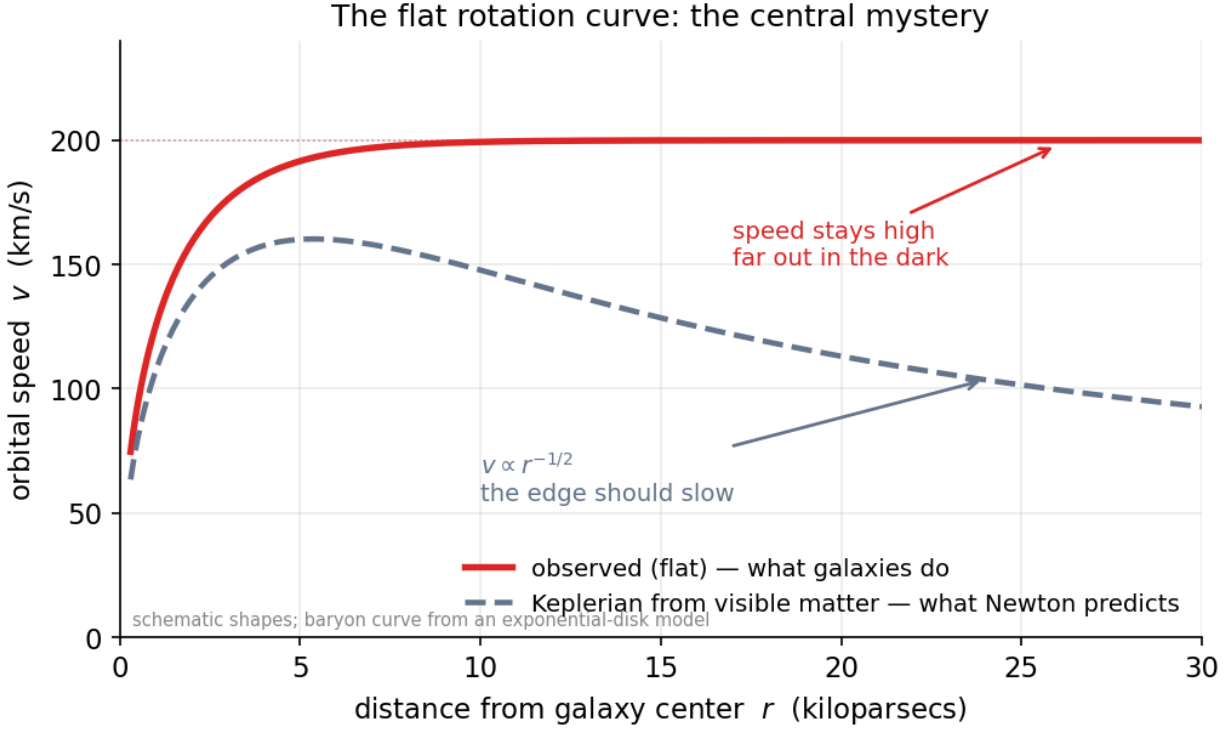
Figure 1: Rotation curve: predicted Keplerian falloff versus the observed flat curve
