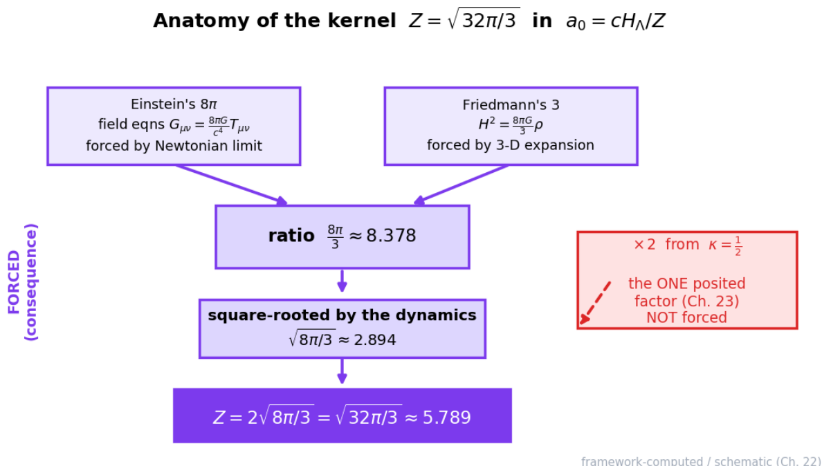
Figure 65: Flow diagram: Einstein’s 8\pi and Friedmann’s 3 combine to 8\pi/3 , square-rooted, times kappa, giving Z = 5.789
