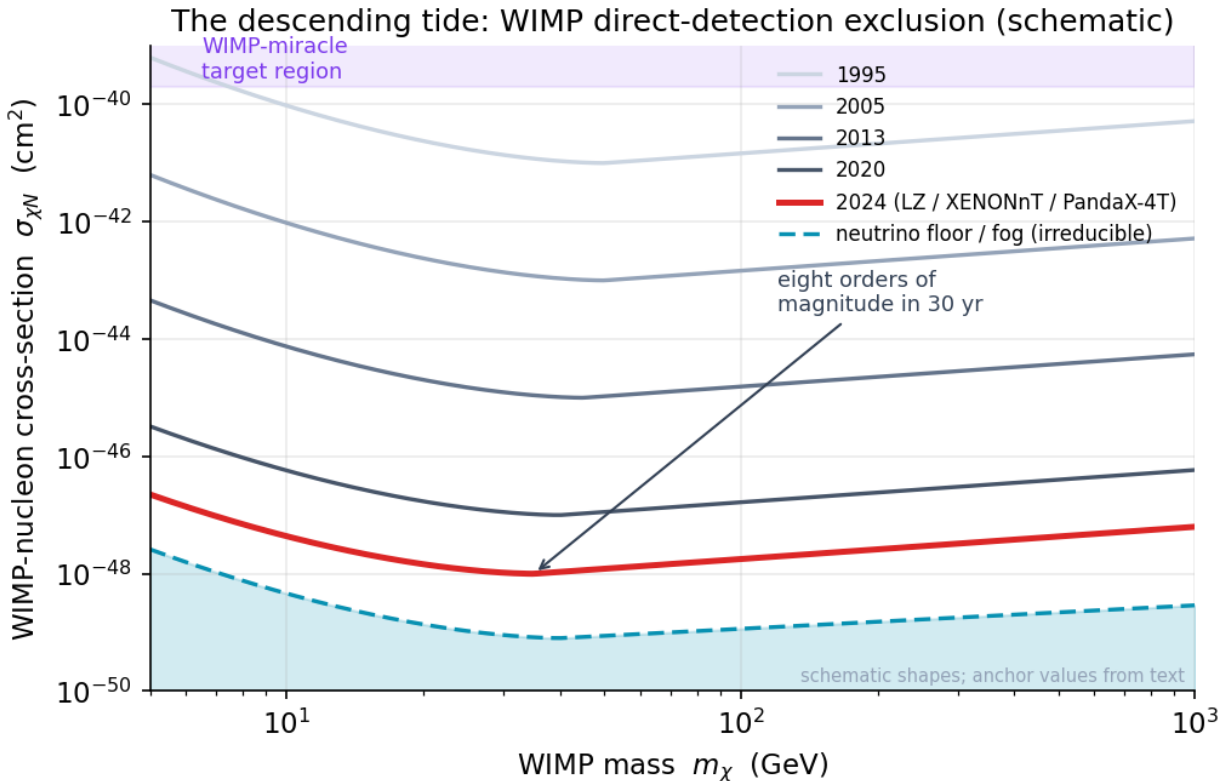
Figure 18: Five stacked exclusion curves stepping downward by decade, each a valley with a minimum near tens of GeV, approaching a shaded neutrino-floor band
