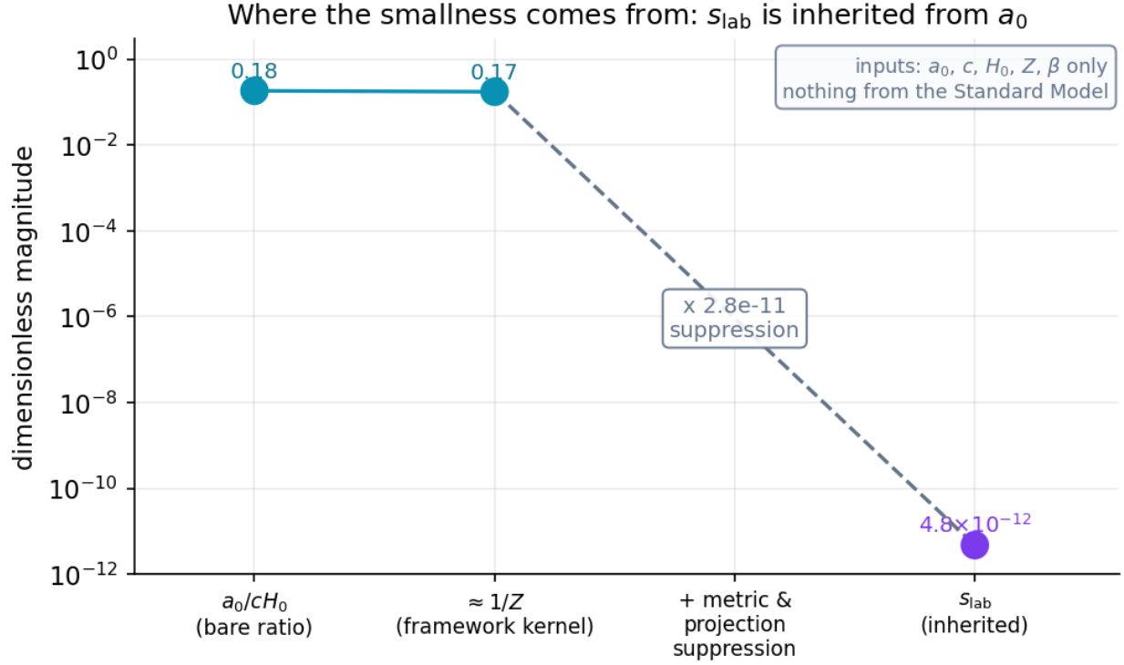
Figure 90: Log-scale waterfall showing the bare ratio a_0/cH_0 dropping to the tiny inherited coefficient
