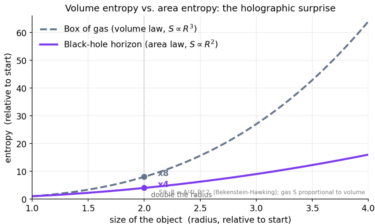
Figure 48: Entropy scaling: gas grows with volume, a black hole with area
