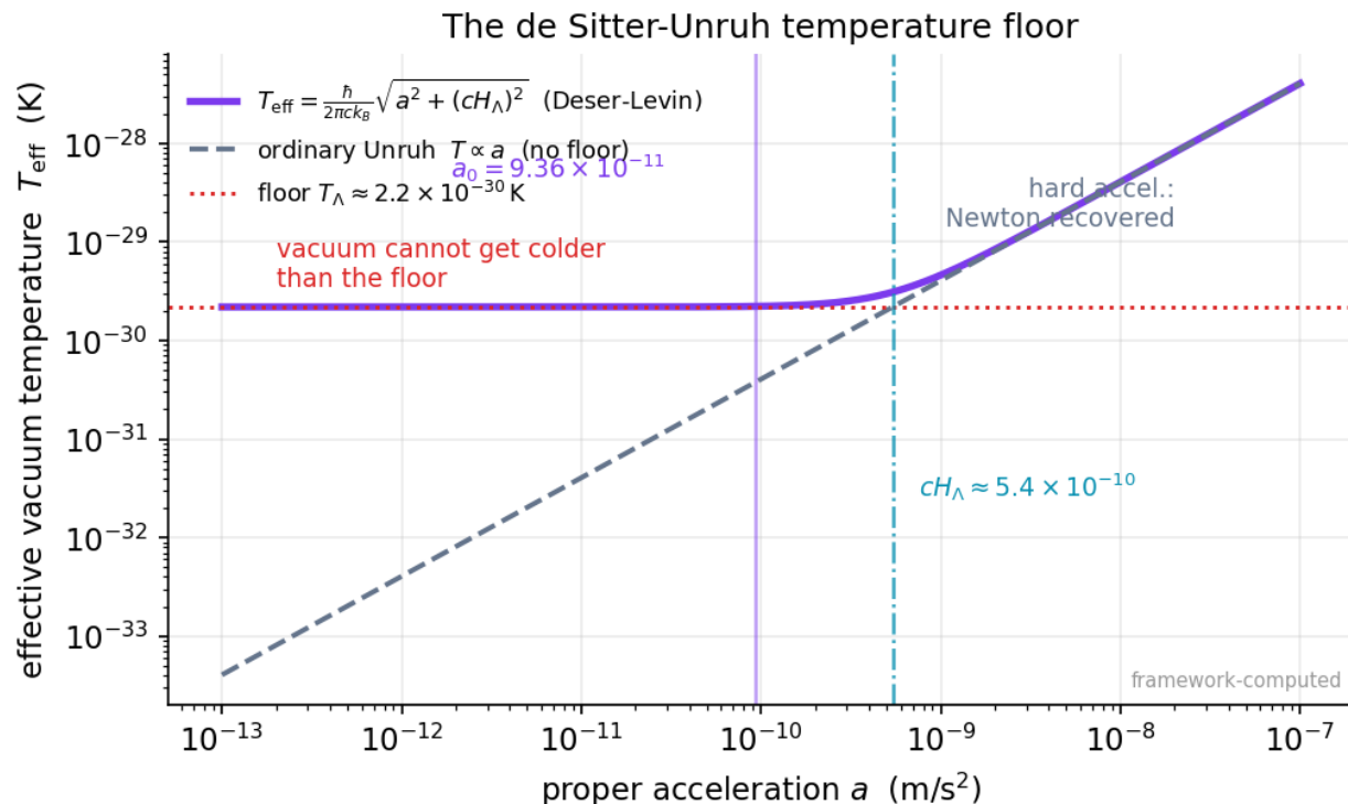
Figure 62: Log-log plot of effective vacuum temperature versus acceleration, showing the ordinary Unruh line bending into a constant floor.
