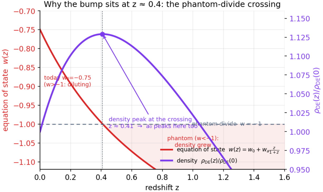
Figure 73: The CPL equation of state w(z) crossing minus one while the dark-energy density reaches its maximum at the same redshift near 0.4
