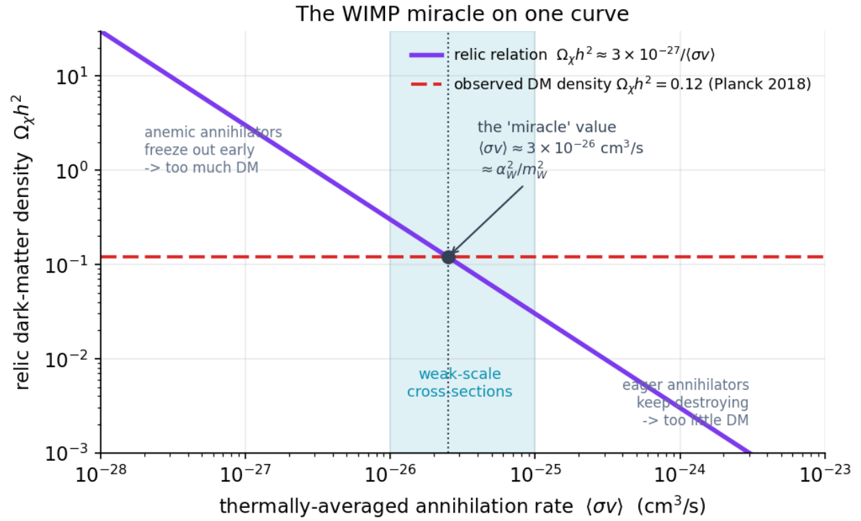
Figure 16: Relic dark-matter abundance falling as one over the annihilation cross-section, crossing the observed Planck density exactly at the weak-scale value
