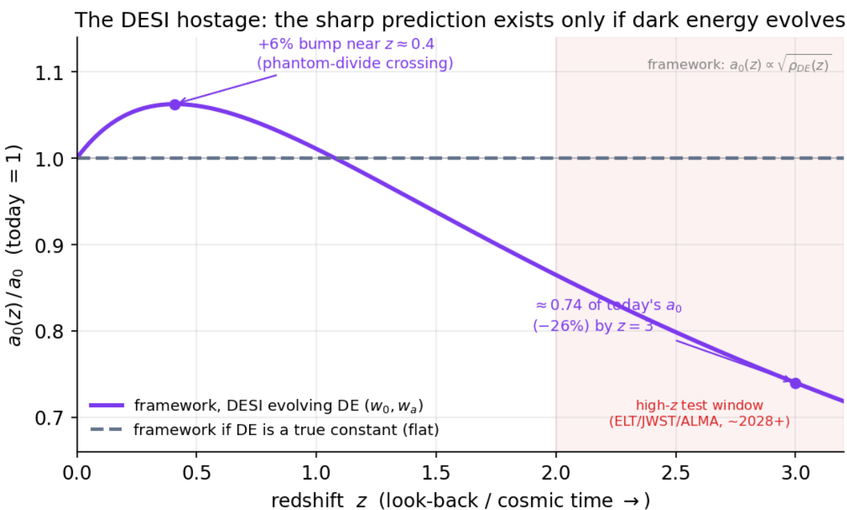
Figure 92: Curve of a_0 versus redshift: a purple line rising 6% near z=0.4 then declining to 0.74 by z=3 , against a flat grey dashed line
