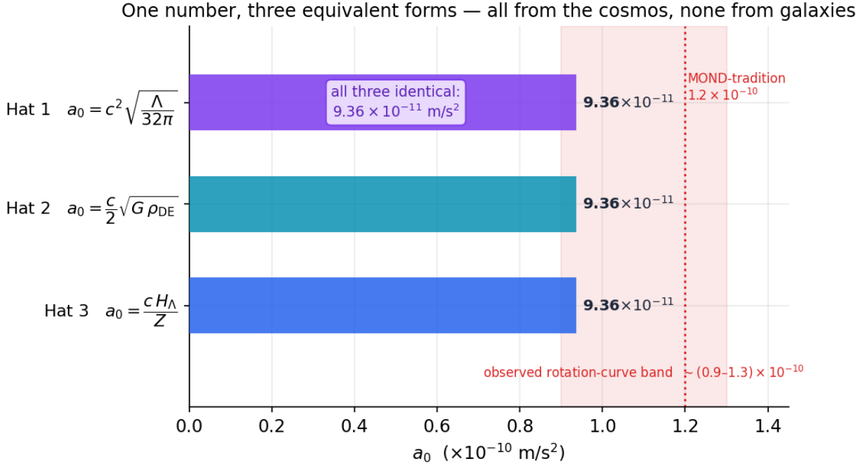
Figure 59: Three equivalent forms of a-naught all landing on the same value
