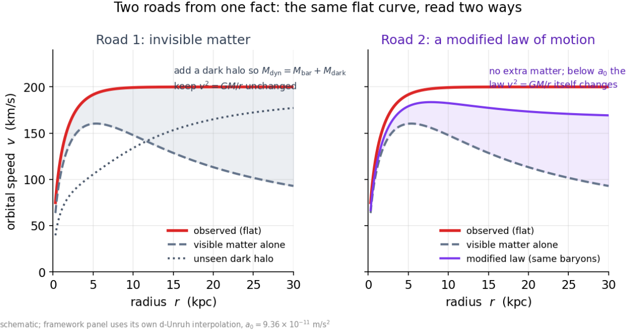
Figure 3: Two panels: dark matter halo versus a modified law of motion, both fitting the same flat curve
