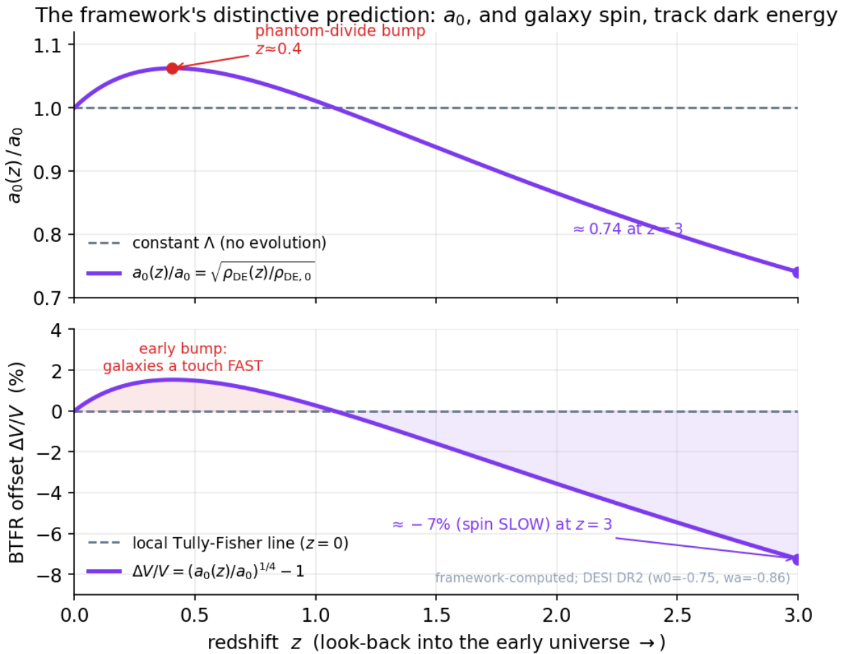
Figure 76: Two stacked curves: a_0 relative to today and the resulting Tully-Fisher rotation-speed offset, both versus redshift
