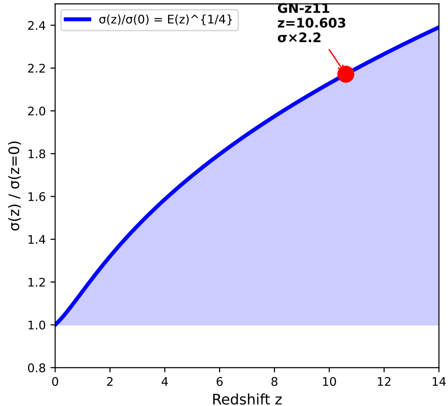
C. Velocity Dispersion Enhancement
