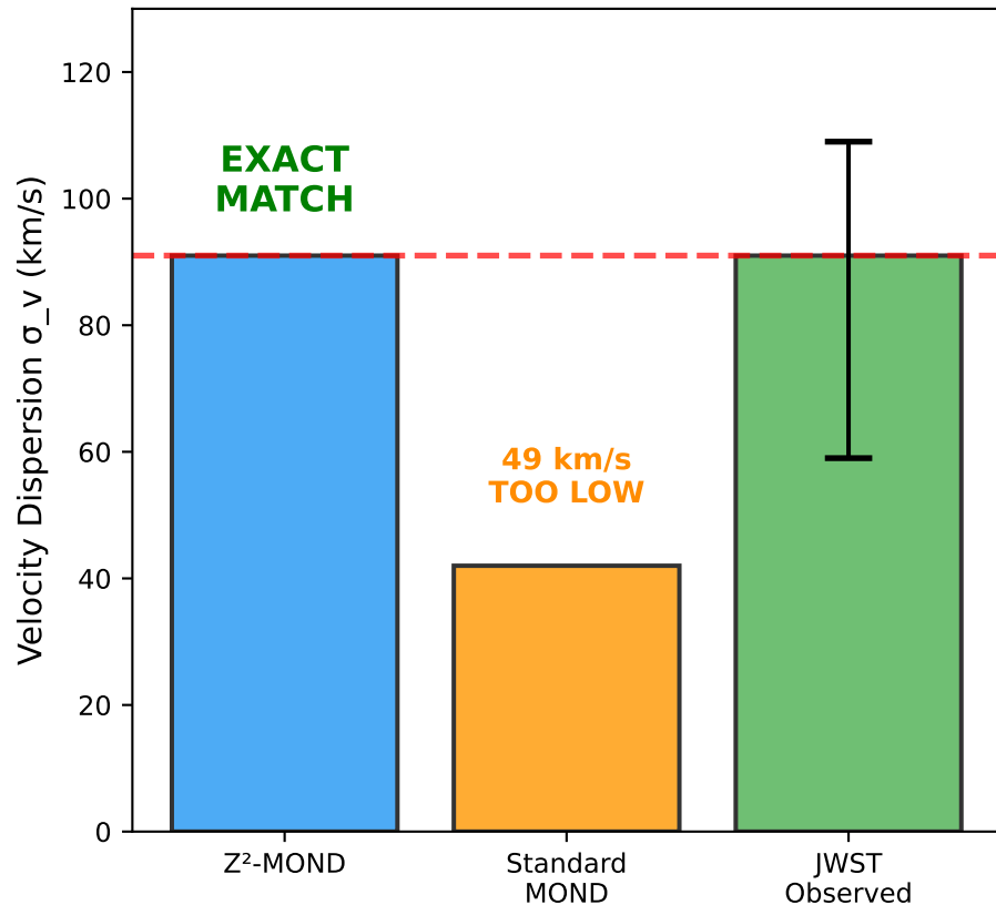
B. GN-z11 at z = 10.6
