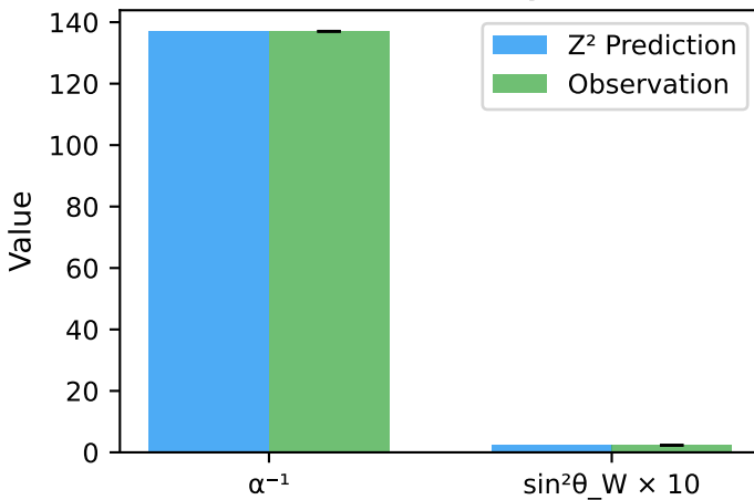
B. Particle Physics
