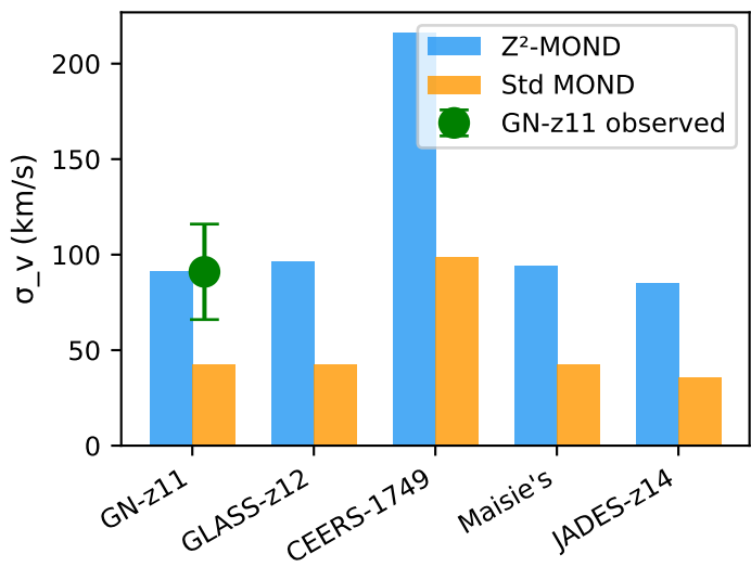
G. Predictions for z>10 Galaxies
