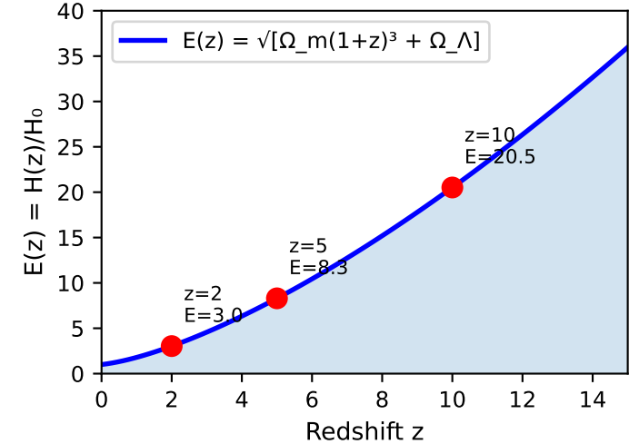
G. Predictions for z>10 Galaxies
