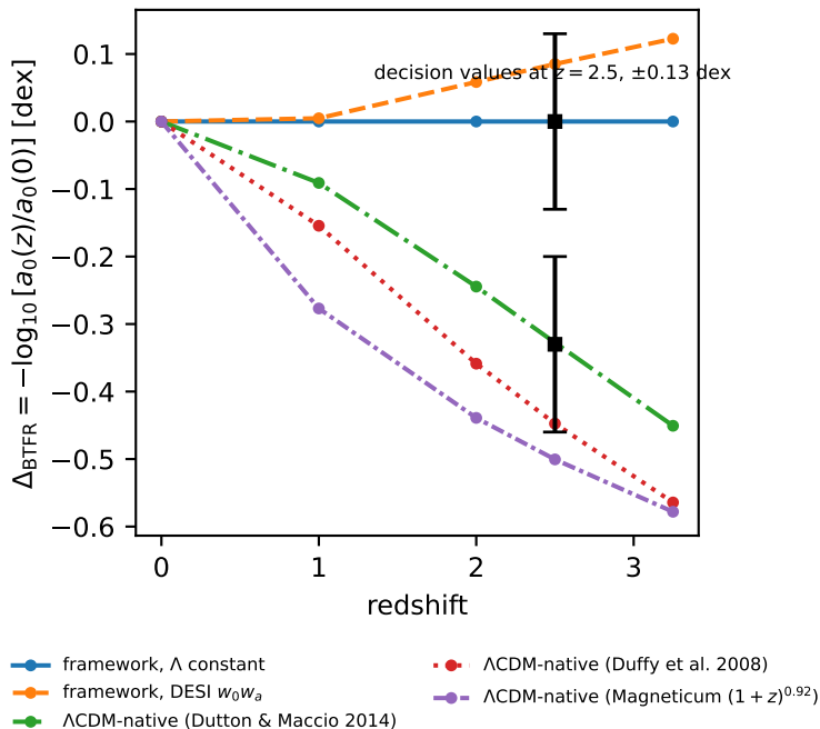
deep-MOND Tully--Fisher zero point vs z
