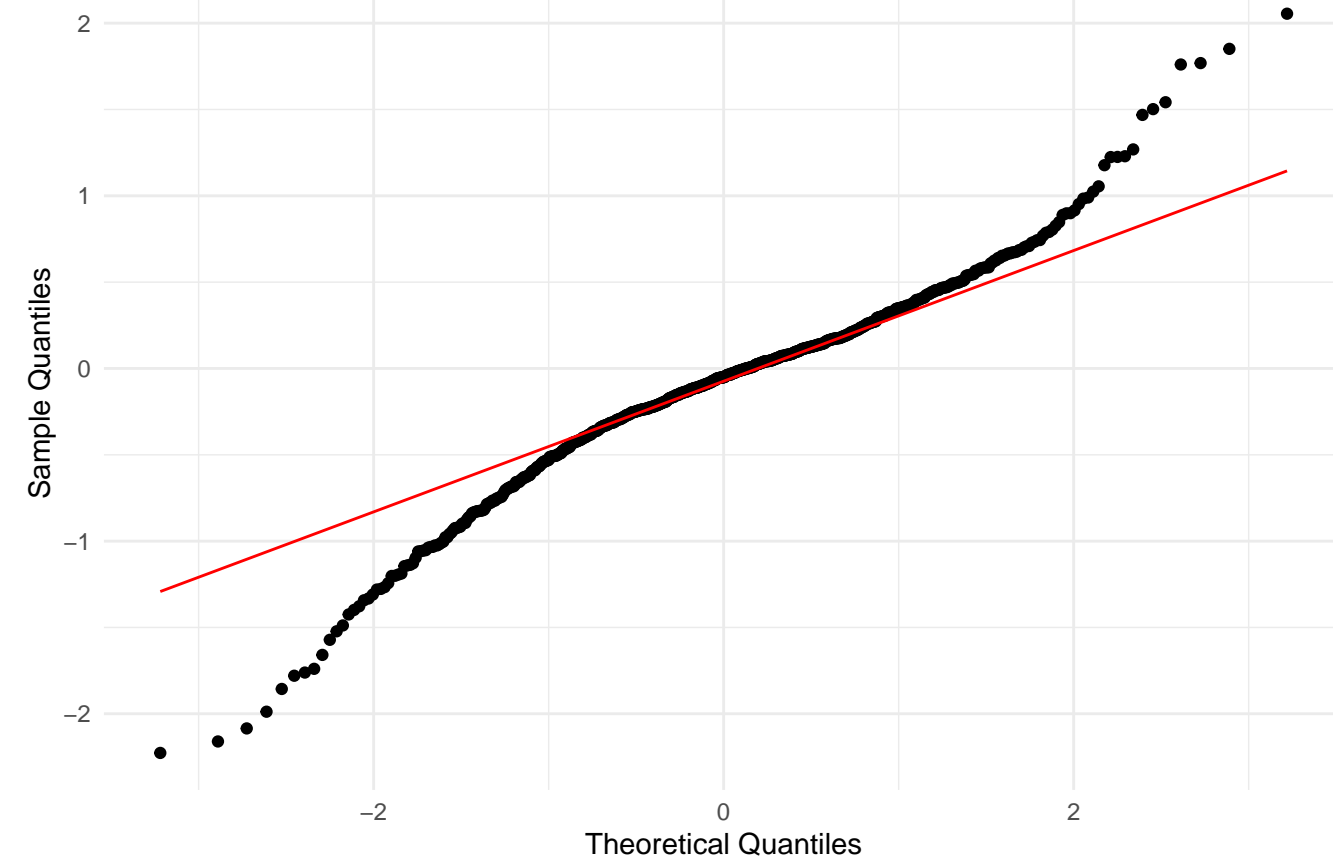
Severity Model: Q-Q Plot
