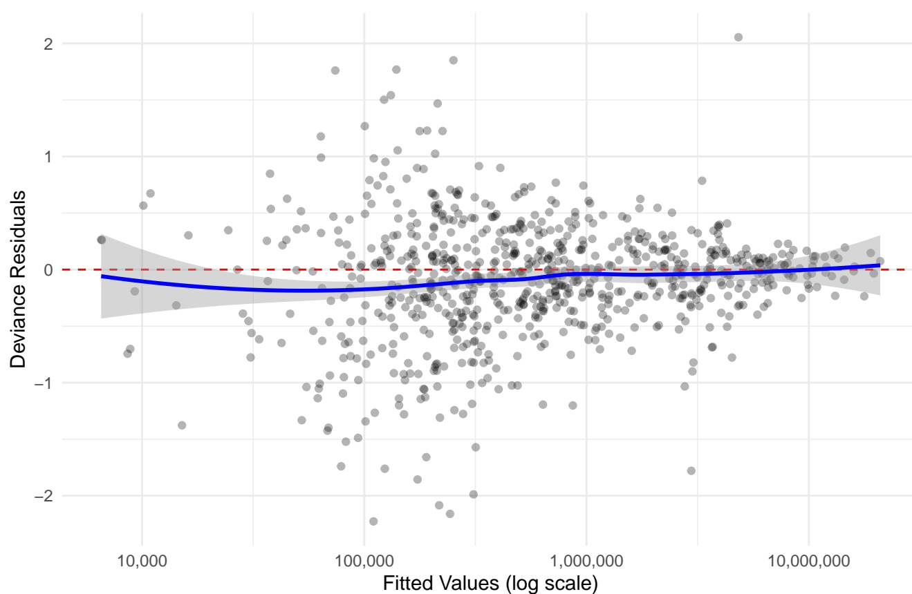
Severity Model: Residual Plot
