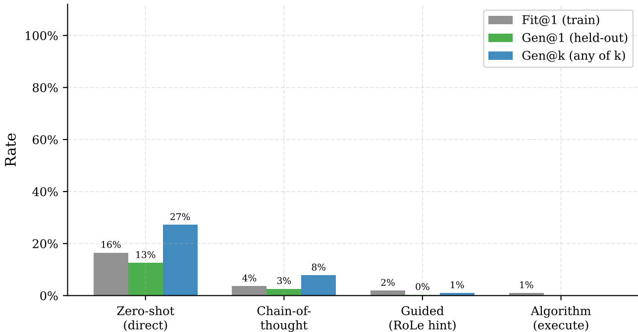
Generalisation by prompting mode
