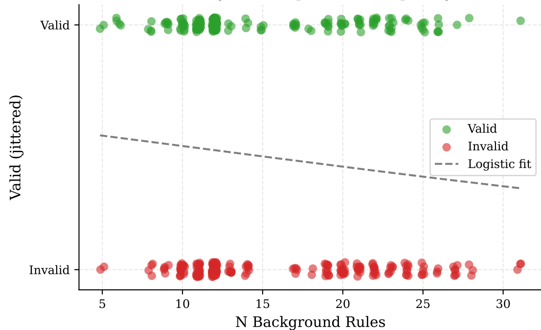
Validity rate vs. problem complexity
