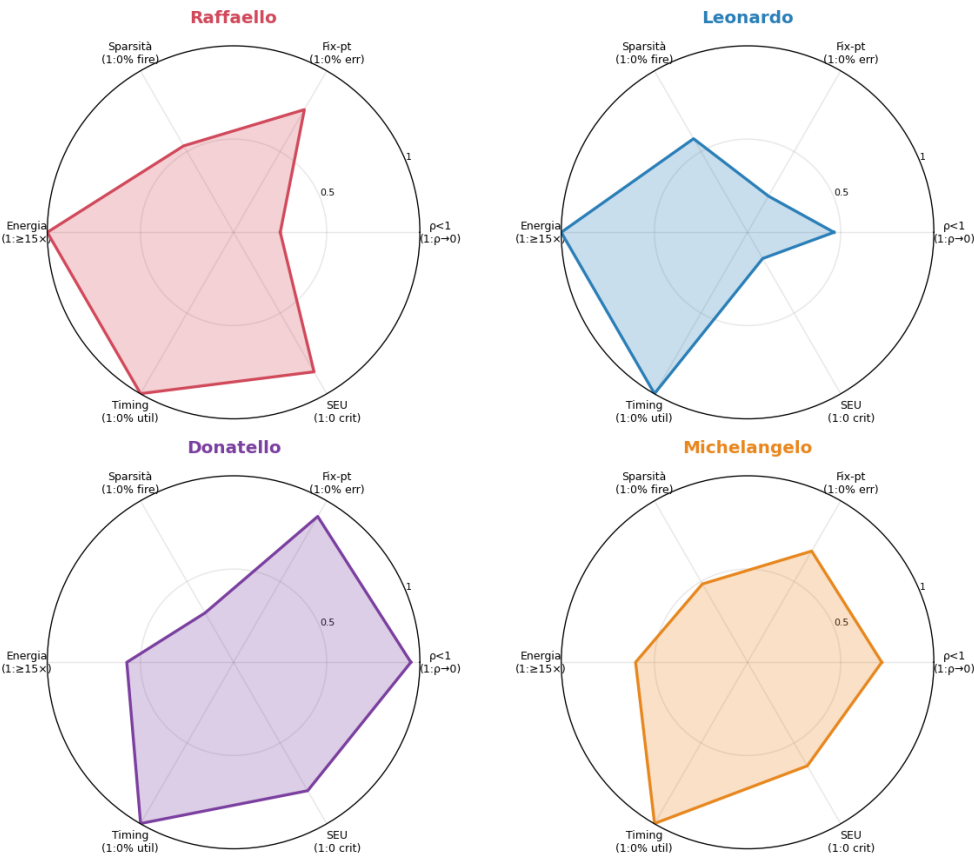
Readiness Radar
