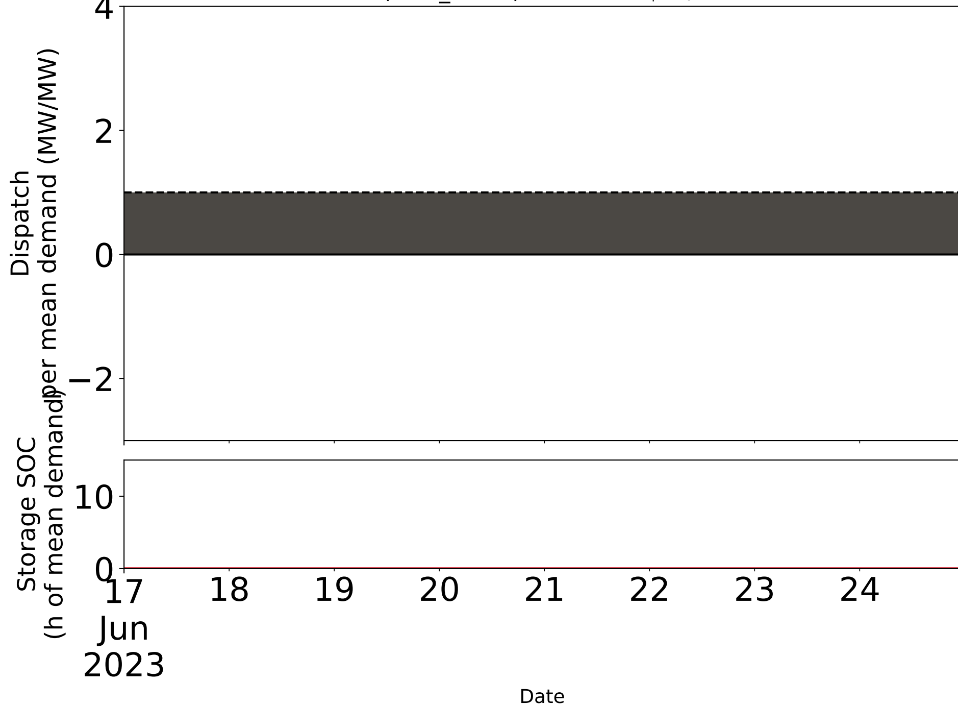
Dispatch Curve for Germany Cell (8.75_48.25) - Gas Cost $50/MWh
