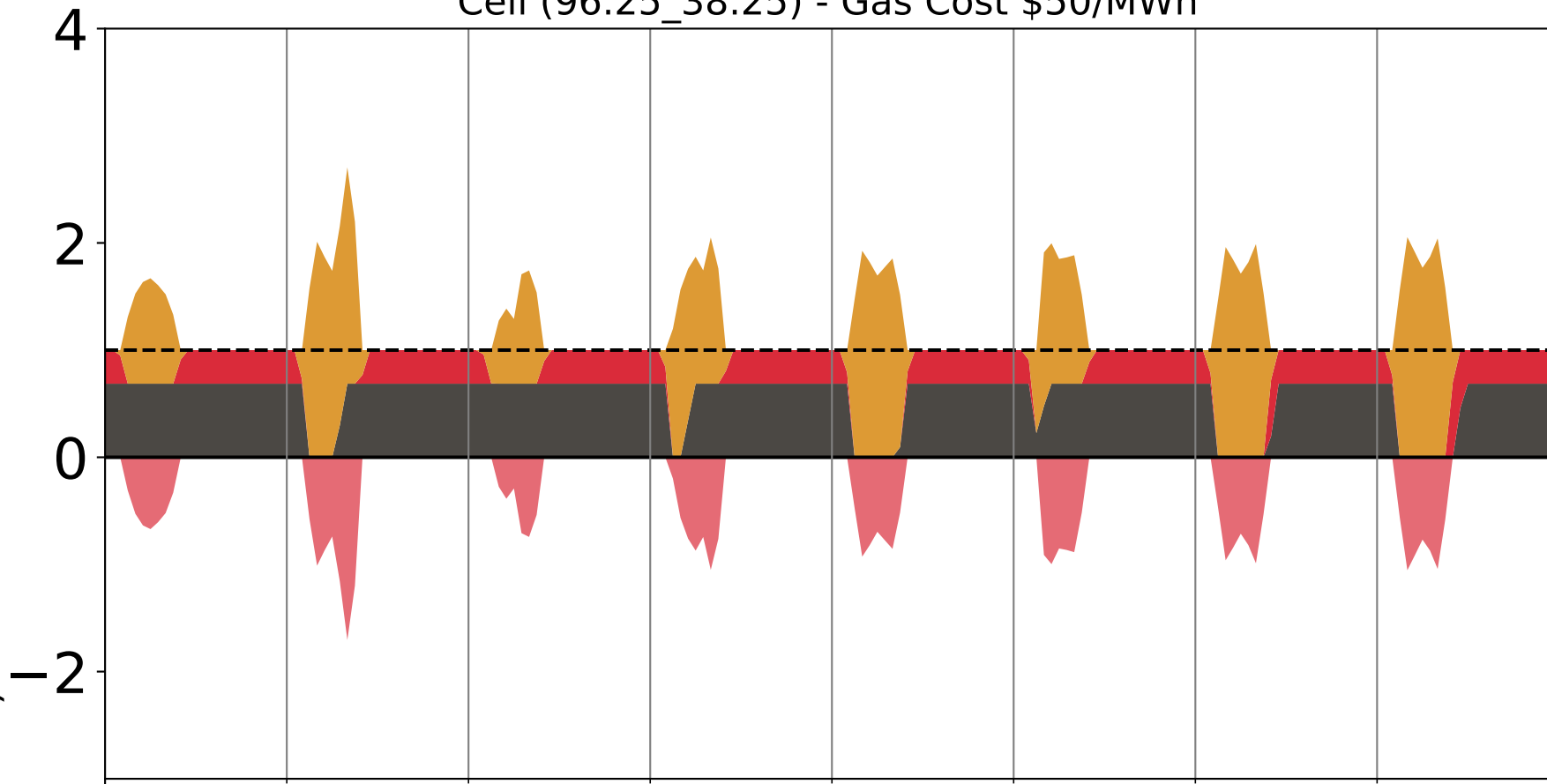
Dispatch Curve for China Cell (96.25_38.25) - Gas Cost $50/MWh
