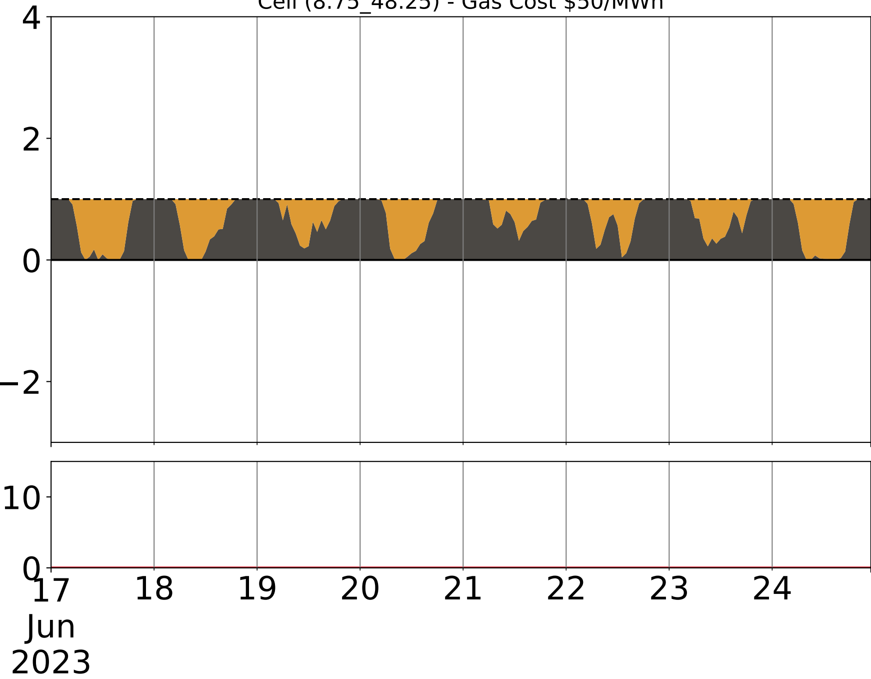
Dispatch Curve for Germany Cell (8.75_48.25) - Gas Cost $50/MWh
