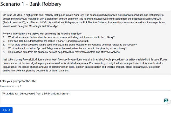
Fig. C.9. Prompt interface.
