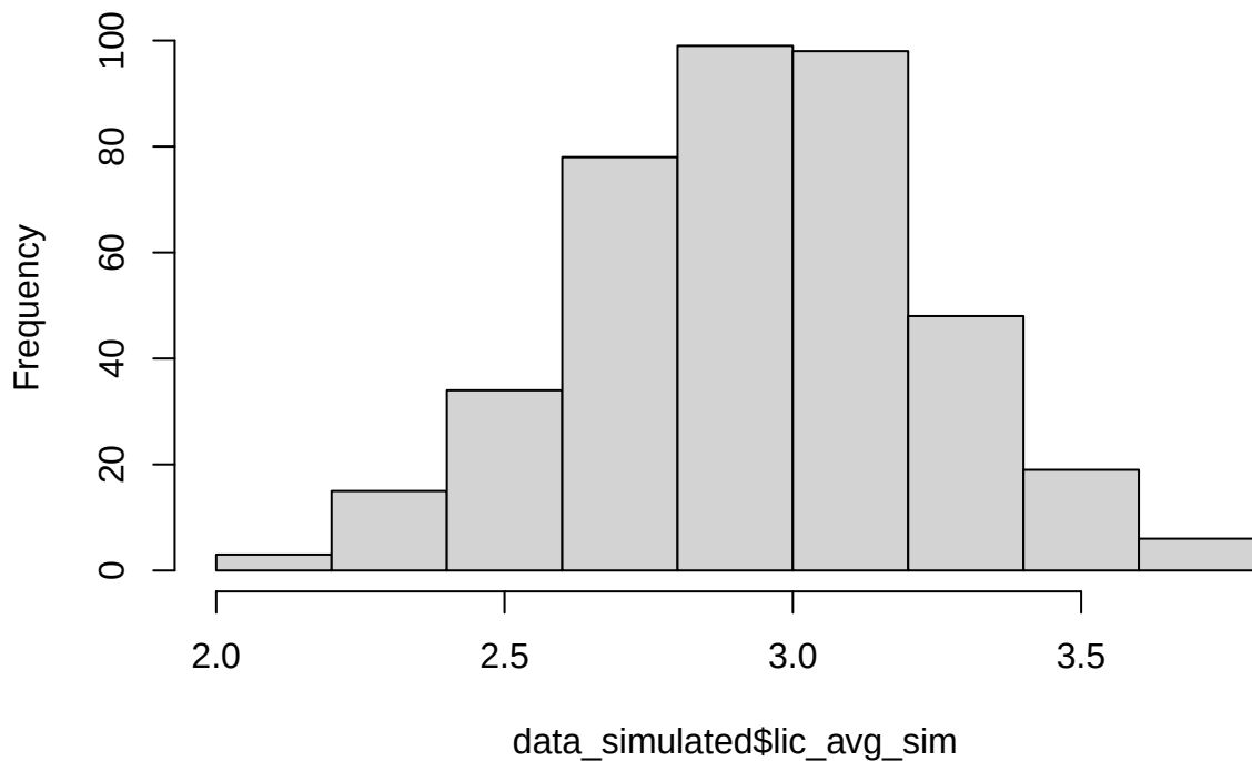
Histogram of data_simulated$lic_avg_sim
