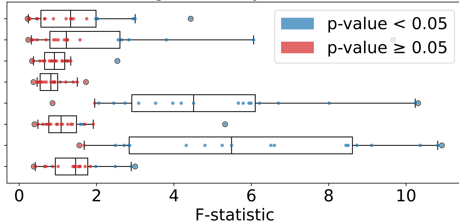
Granger Causality F-statistics
