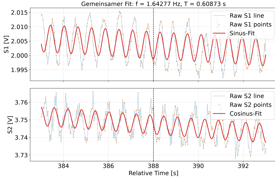
Figure 5.10: Detailed evaluation of the quadrature homodyne signals. The fitted sine and cosine curves show a phase shift of 90^\circ , confirming the quadrature relation between the two photodiode signals.
