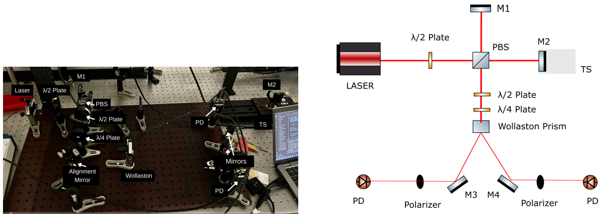
Figure 5.8: Laboratory setup and schematic representation of the quadrature homodyne interferometer. The setup extends the Michelson interferometer with polarization optics in order to generate two phase-shifted photodiode signals for direction-sensitive displacement detection. M1–M4 denote mirrors, PD denotes the photodiode, TS denotes the translation stage, and PBS denotes the polarizing beam splitter. Although the polarizers at the end are included in the schematic for completeness, they are omitted in the actual setup photograph, as the Wollaston prism theoretically acts as a perfect polarizing beam splitter.
