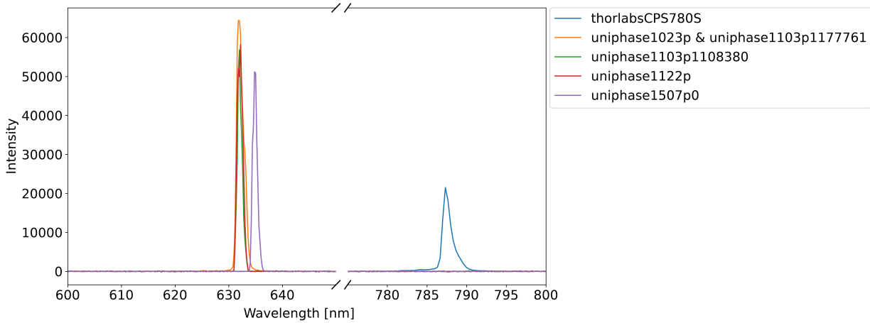
Figure 3.2: Background-corrected spectra of the investigated laser sources used for determining the peak emission wavelengths. The spectra of the Uniphase 1023P and the Uniphase 1103P (1177761) were identical apart from saturation in the latter. Therefore, the unsaturated spectrum was used to represent both laser sources.
