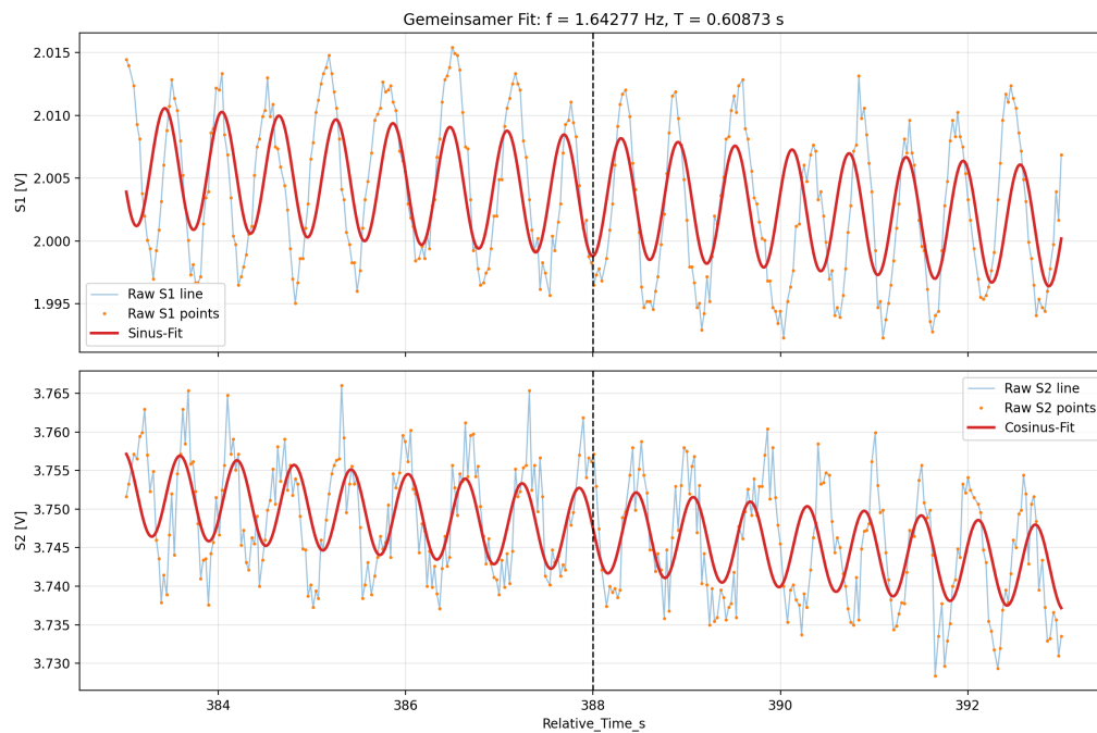
Figure 5.11: Detailed evaluation of the quadrature homodyne signals. The fitted sine and cosine curves show an approximate phase shift of 90^\circ , confirming the quadrature relation between the two photodiode signals.
