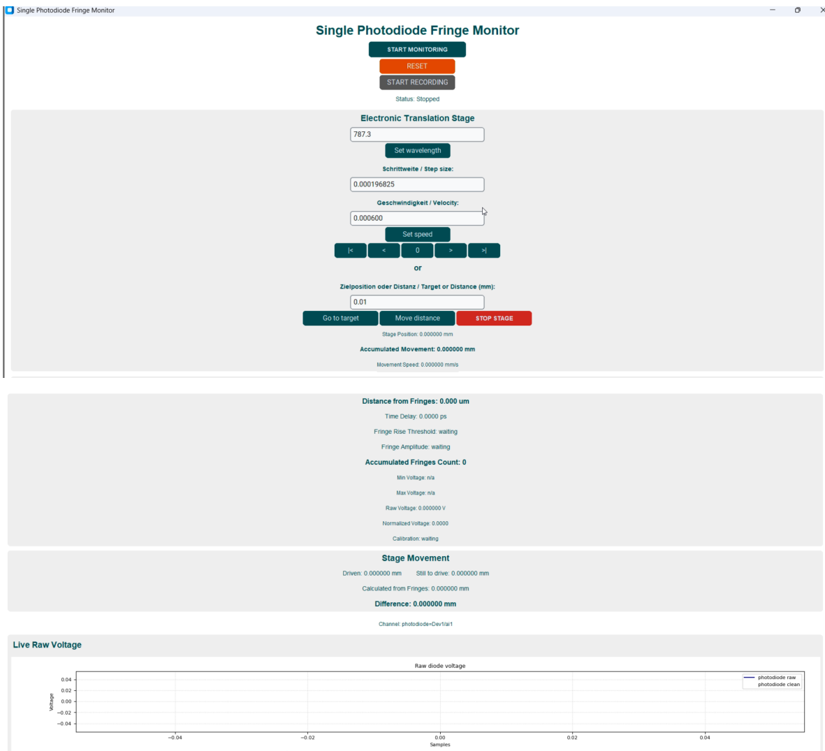
Figure 4.2: Graphical user interface of the single diode software. Top: upper part of the scrollable interface. Bottom: lower part of the interface.
