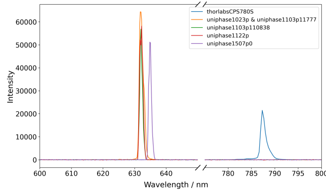
Figure 3.2: Background-corrected spectra of the investigated laser sources used for determining the peak emission wavelengths.
