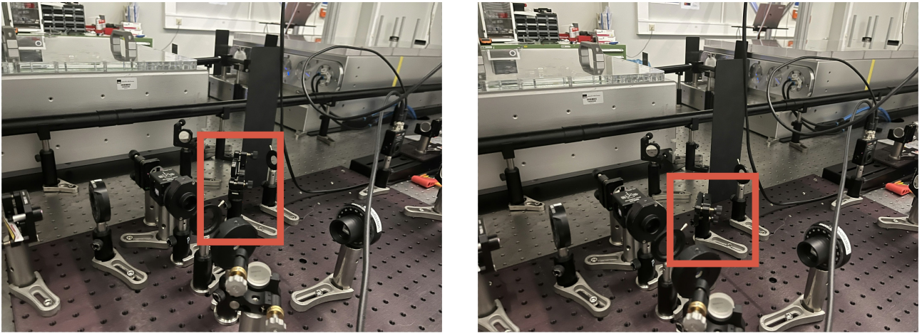
Figure 6.1: Integration of the interferometer into the electro-optic sampling setup. Left: integrated configuration with the flip mirror raised, so that the signal from the external setup is coupled into the interferometer. Right: standalone configuration with the flip mirror lowered, so that the interferometer can be used with the local translation stage.
