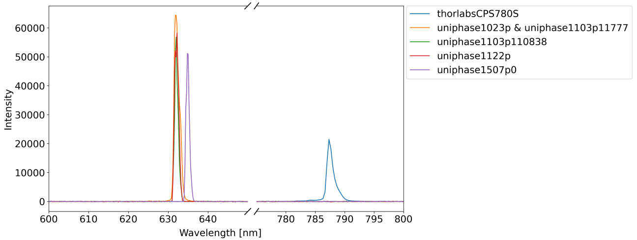
Figure 3.2: Background-corrected spectra of the investigated laser sources used for determining the peak emission wavelengths. The spectra of the Uniphase 1023P and the Uniphase 1103P (1177761) were identical apart from saturation in the latter. Therefore, the unsaturated spectrum was used to represent both laser sources.
