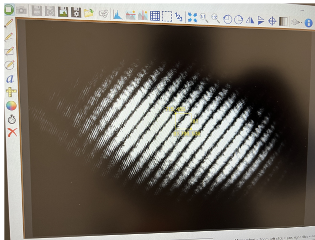
Figure 5.2: Stable interference fringes observed with the camera in the ThorCam software.
