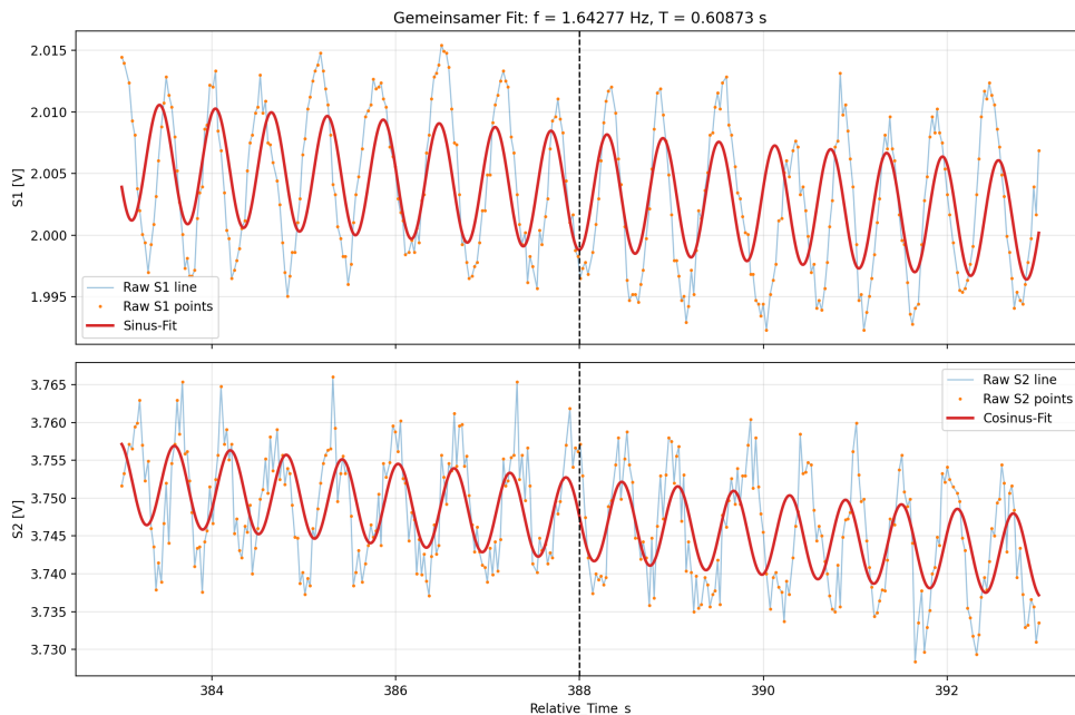
Figure 5.11: Detailed evaluation of the quadrature homodyne signals. The fitted sine and cosine curves show a phase shift of 90^\circ , confirming the quadrature relation between the two photodiode signals.
