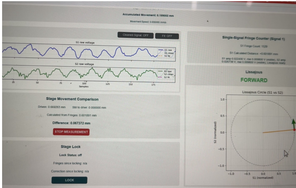
Figure 5.10: Measurement result obtained with the quadrature homodyne interferometer. The two photodiode signals were detected successfully, and the Lissajous representation was used to evaluate the direction-dependent phase relation.
