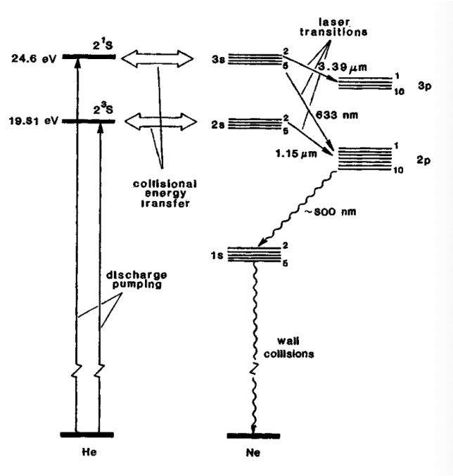
Figure 2.7: Simplified energy level diagram of the HeNe laser (obtained from [21]).
