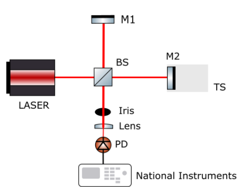
Figure 5.4: Electronic signal detection using a photodiode, schematic representation. BS denotes the beam splitter, M1 the reference mirror, M2 the measurement mirror, TS the translation stage, and PD the photodiode.
