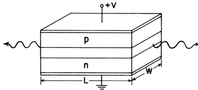
Figure 2.8: Schematic structure of a semiconductor diode laser. The active region is located at the pn-junction, where injected electrons and holes recombine and generate optical radiation. Obtained from [16]
