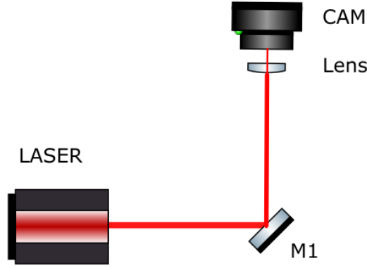
Figure 3.3: Experimental setup and schematic representation of the beam profile measurements with the RayCi beam profiling camera. In the schematic, M1 denotes the mirror and CAM denotes the RayCi beam profiling camera.
