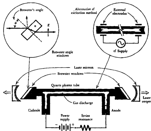
Figure 2.6: Schematic setup of a HeNe laser (obtained from [19]).
