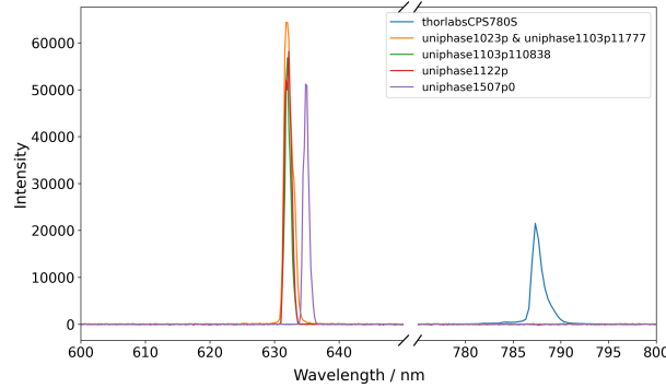
Figure 3.2: Background-corrected spectra of the investigated laser sources used for determining the peak emission wavelengths. The spectra of the Uniphase 1023P and the Uniphase 1103P (1177761) were identical apart from saturation in the latter. Therefore, the unsaturated spectrum was used to represent both laser sources.
