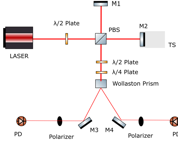
Figure 2.2: Setup for quadrature homodyne interferometry. This configuration visualizes the principle of quadrature signal generation. PBS denotes a polarizing beam splitter, BS describes a beam splitter, M1 – M4 Mirrors, PD a photodiode.
