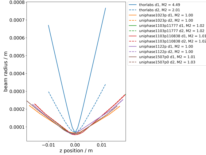
Figure 3.4: Measured beam radii and fitted beam propagation curves. The beam propagation model was fitted independently for both transverse beam axes.
