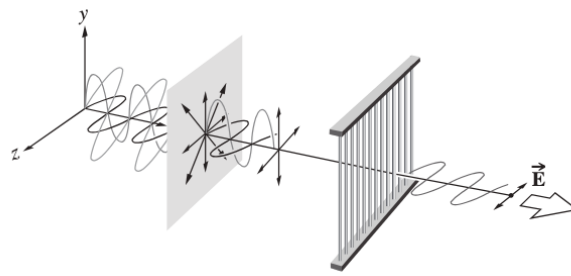
Figure 2.5: Principle of a wire-grid polarizer. The electric field component parallel to the conducting wires is mostly reflected or absorbed, while the perpendicular component is transmitted. Obtained from [39].
