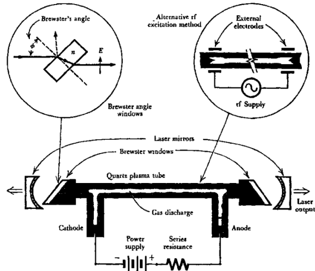
Figure 2.5: Schematic setup of a HeNe laser (obtained from [19]).
