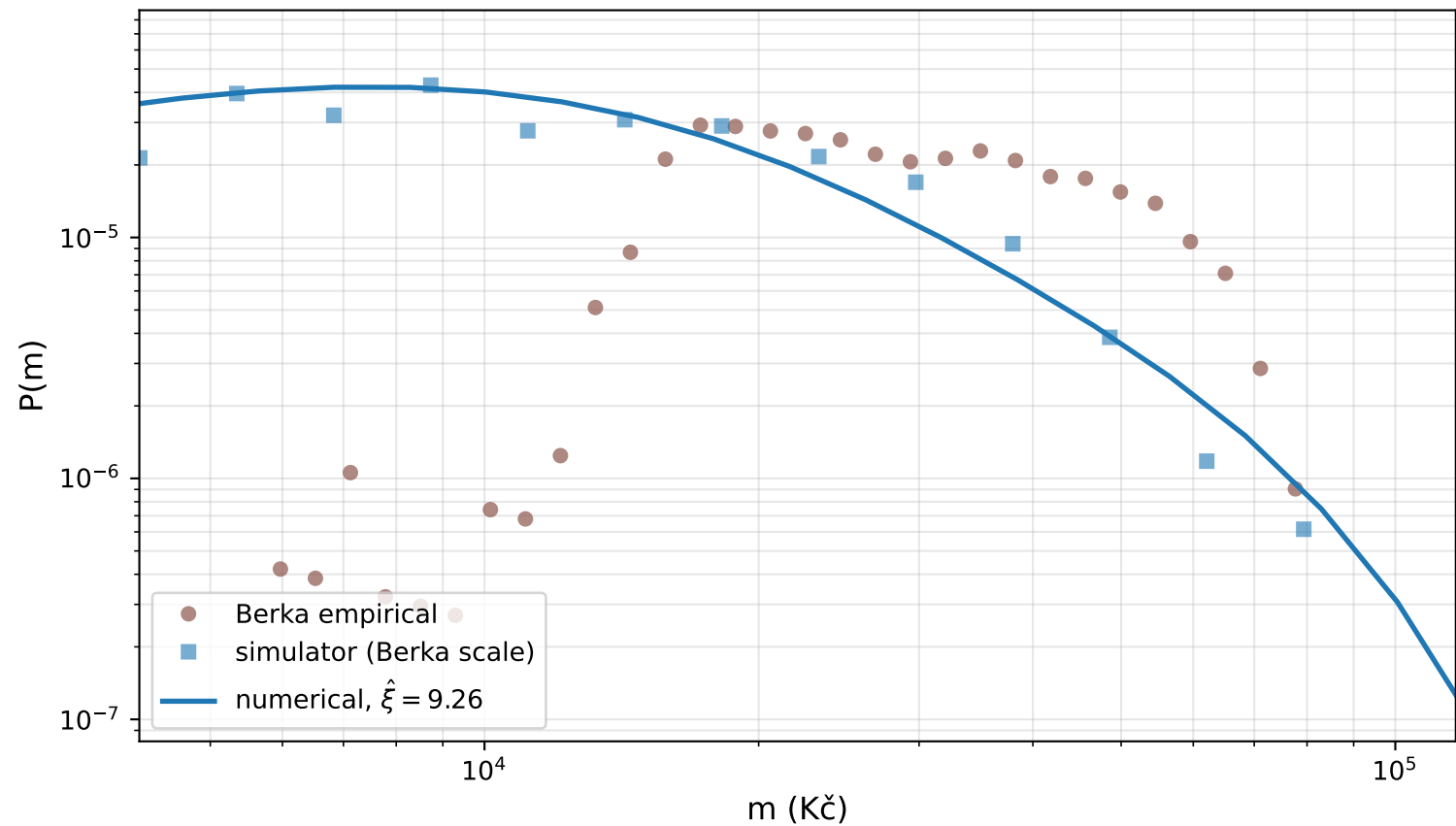
B.1 Berka empirical P(m) — BetaBin ( \hat{\xi} = 9.26 )
