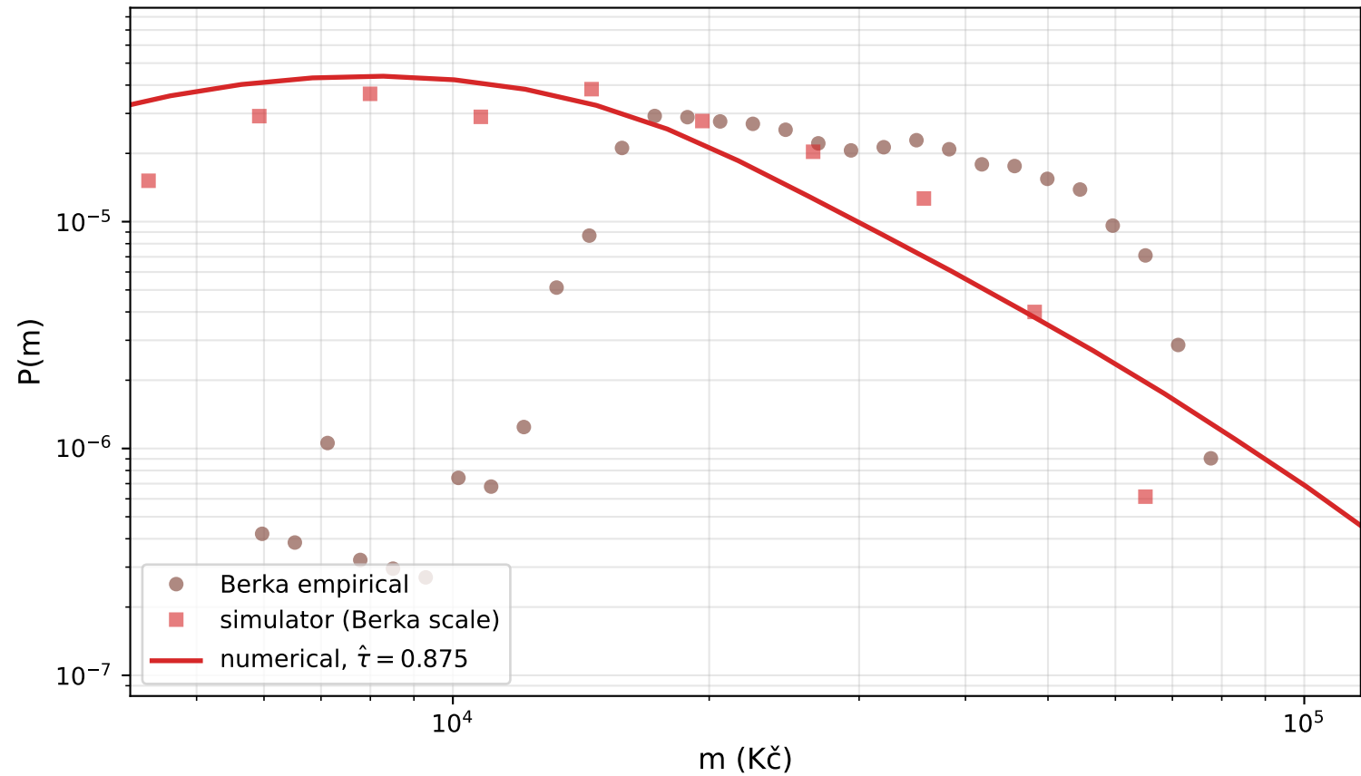
B.1 Berka empirical P(m) — LogitN ( \hat{\tau} = 0.875 )
