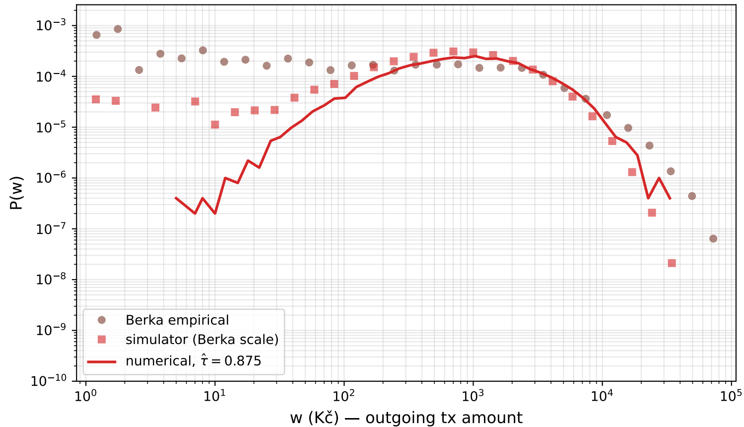
B.2 Berka empirical P(w) — LogitN ( \hat{\tau} = 0.875 )
