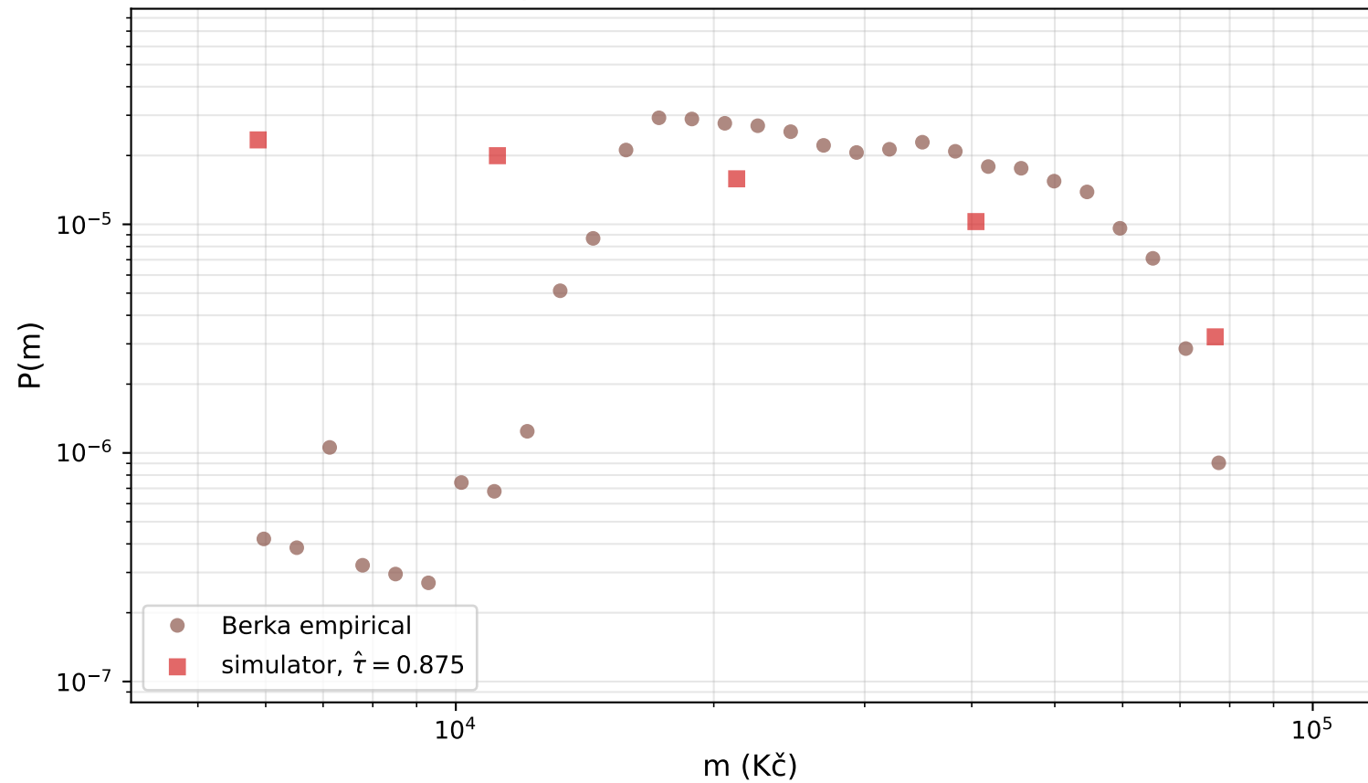
B.1 Berka empirical P(m) vs simulator — LogitN ( \hat{\tau} = 0.875 )
