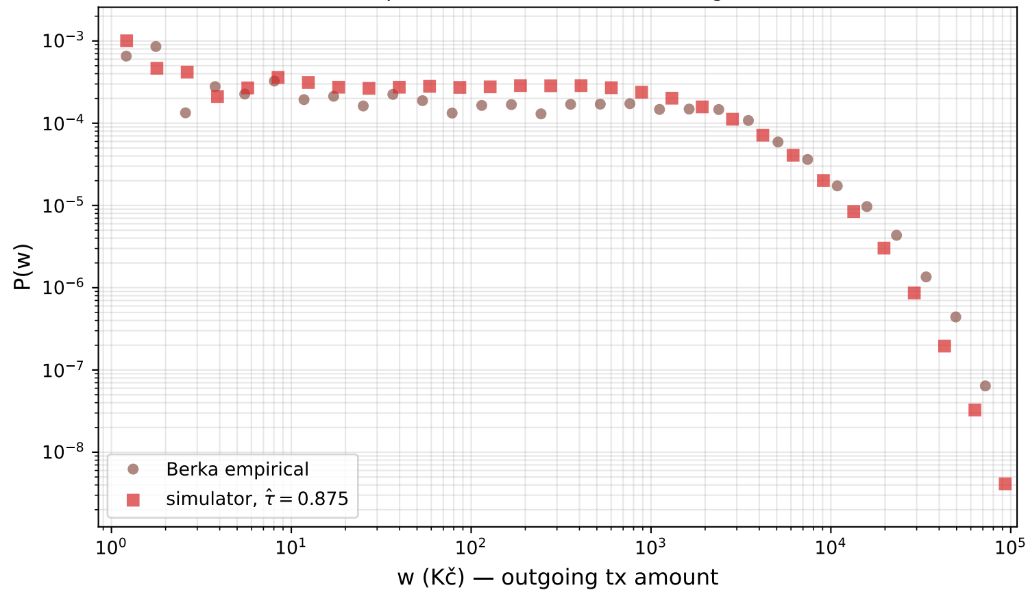
B.2 Berka empirical P(w) vs simulator — LogitN ( \hat{\tau} = 0.875 )
