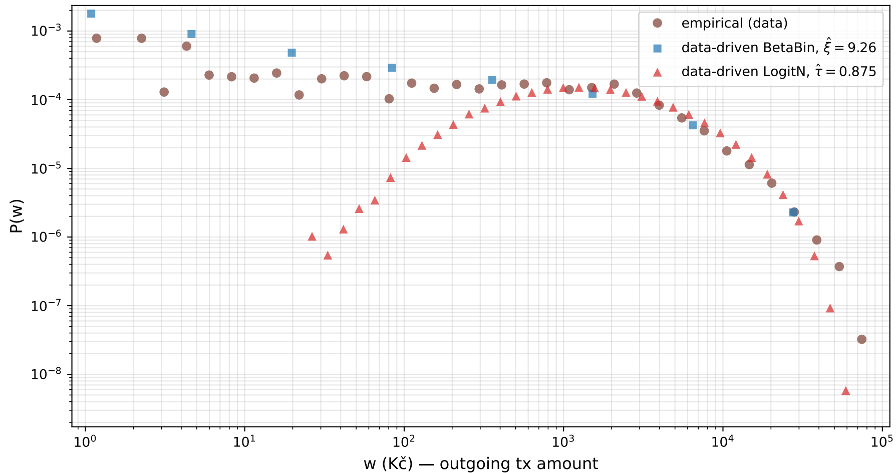
B.3 Data-driven P(w) : w_i = q_i \cdot m_i with q_i drawn per-tx (voluntary debits)
