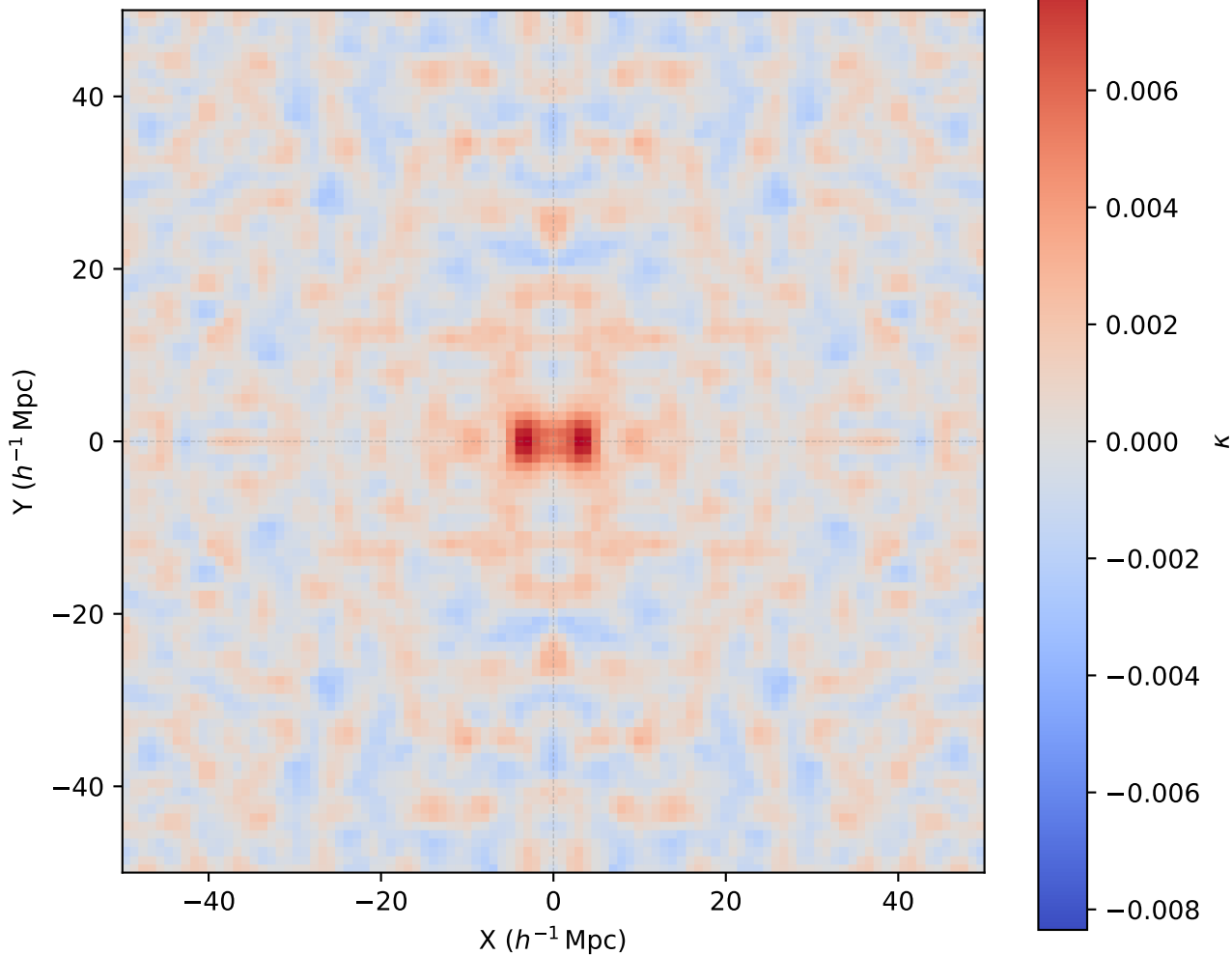
(6) Corrected Pairs = (2)-(4)
