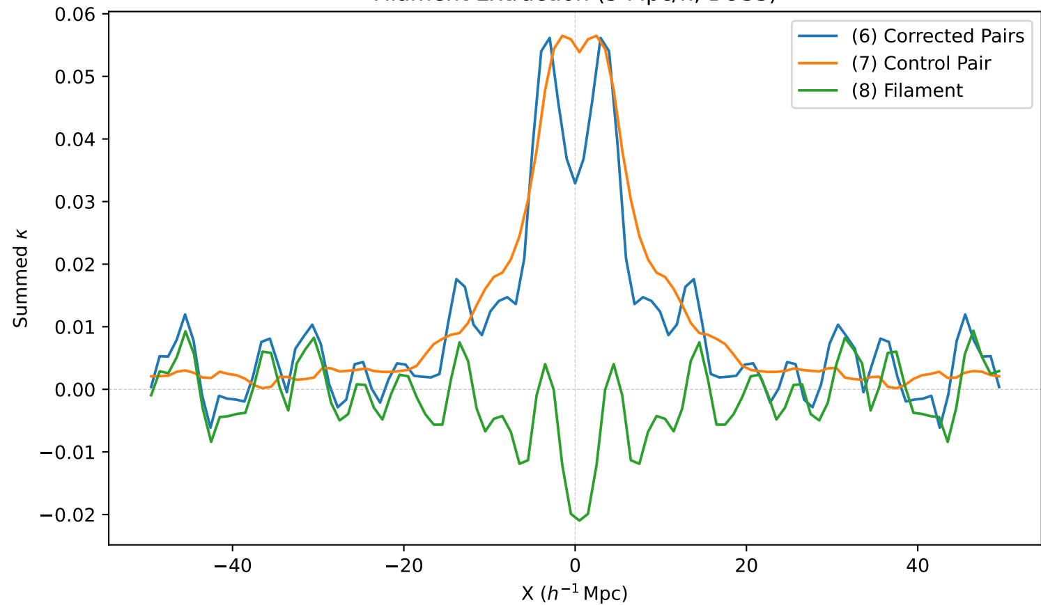
Filament Extraction (5 Mpc/h, BOSS)
