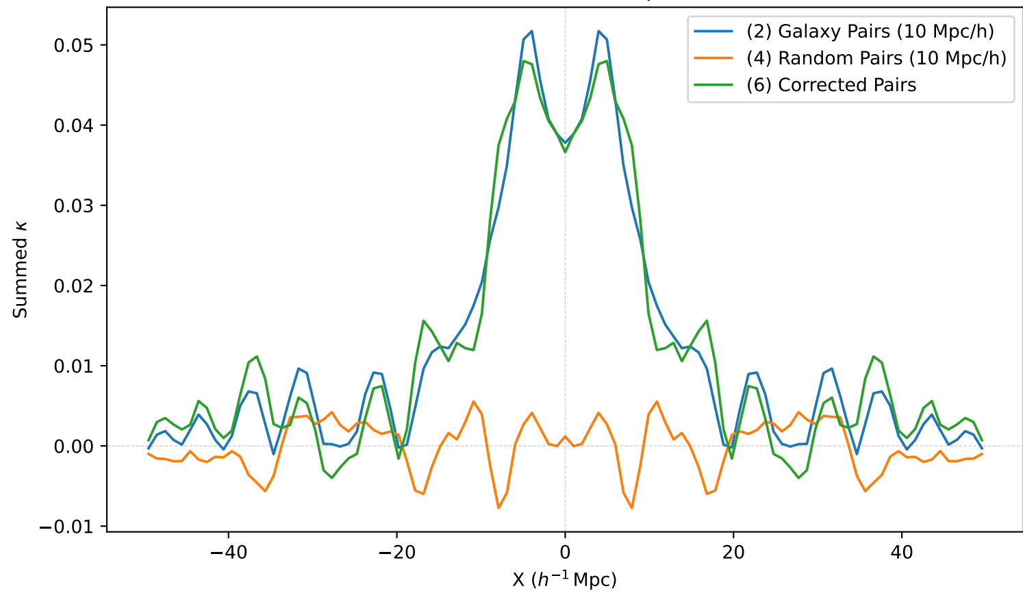
Pair-Stacked Profiles (10 Mpc/h, BOSS)
