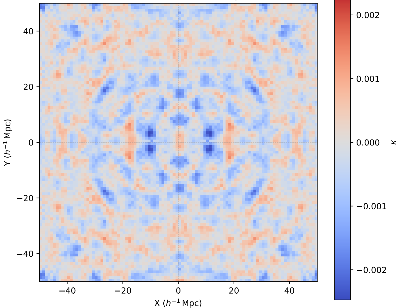
(8) Filament = (6)-(7) [20 Mpc/h]
