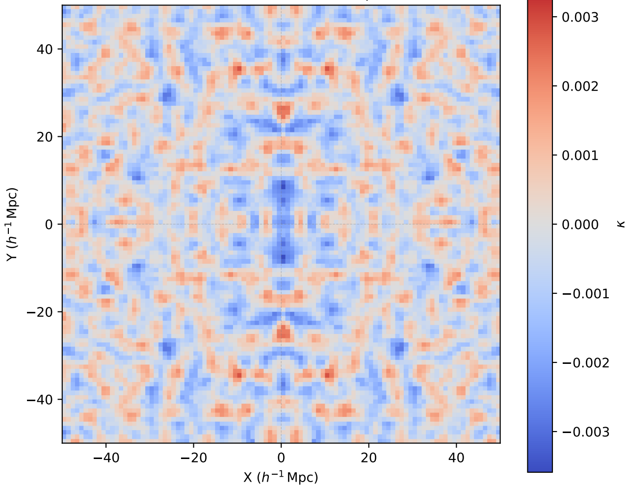
(8) Filament = (6)-(7) [5 Mpc/h]
