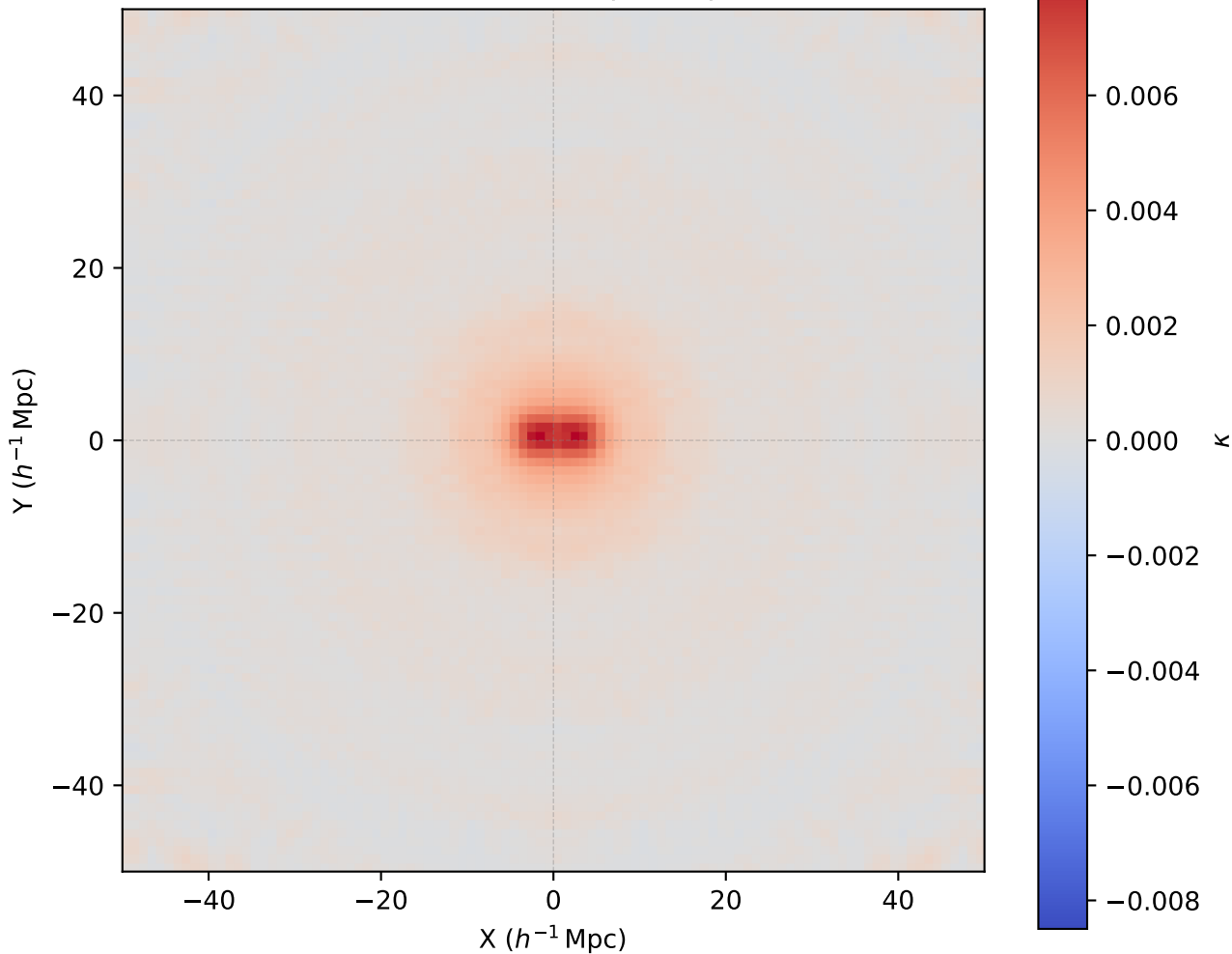
(7) Control Pair Map (5 Mpc/h)
