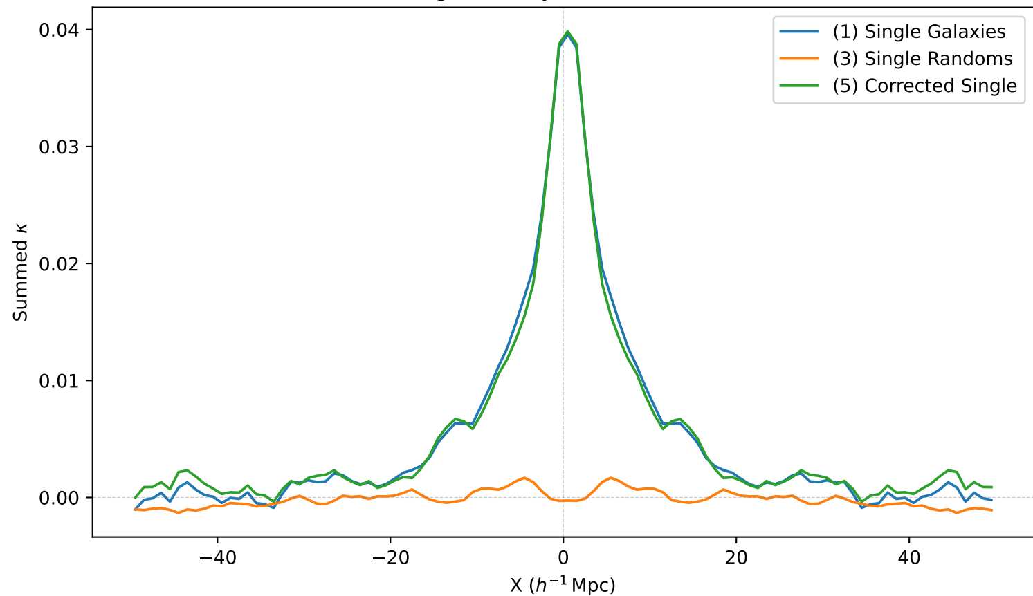
Single-Galaxy Profiles (BOSS)
