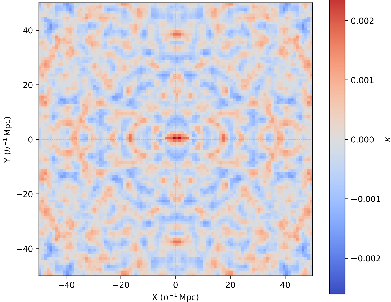
(8) Filament = (6)-(7) [10 Mpc/h]
