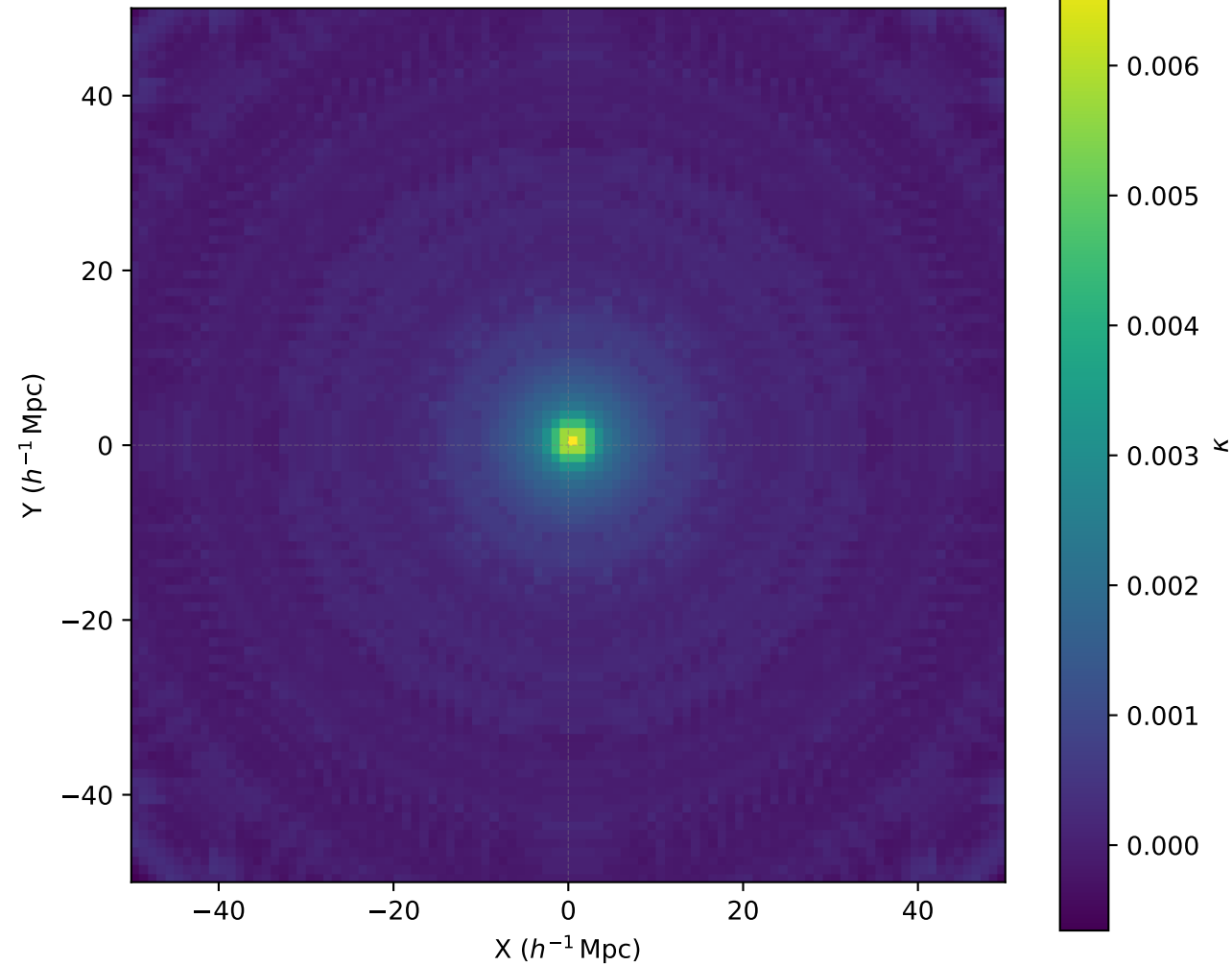
(1) Single Galaxies (BOSS)
