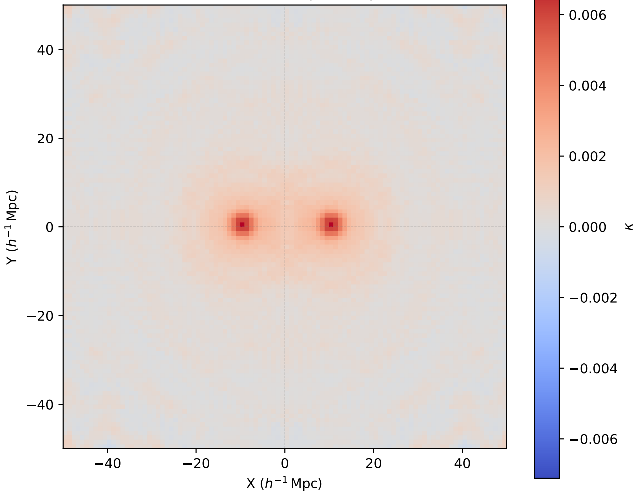
(7) Control Pair Map (20 Mpc/h)
