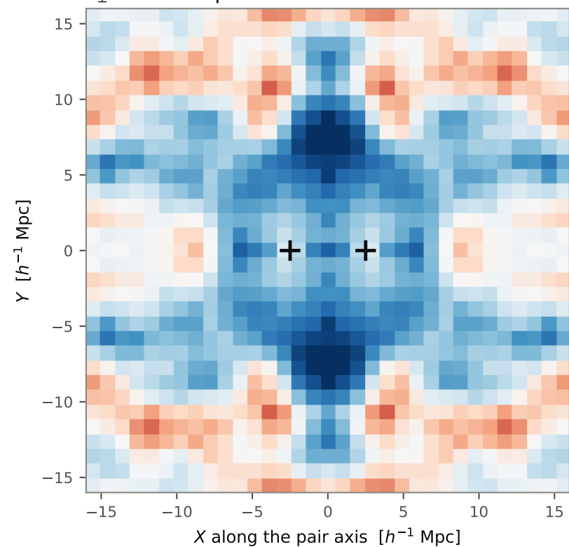
r_{\perp} = 10 h^{-1}\text{Mpc} — observed
