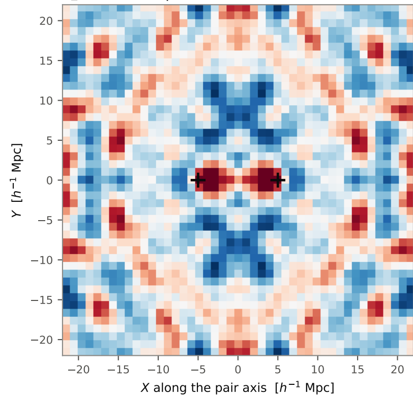
r_{\perp} = 20 h^{-1}\text{Mpc} — observed
