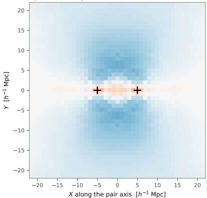
r_{\perp} = 20 h^{-1}\text{Mpc} — theoretical
