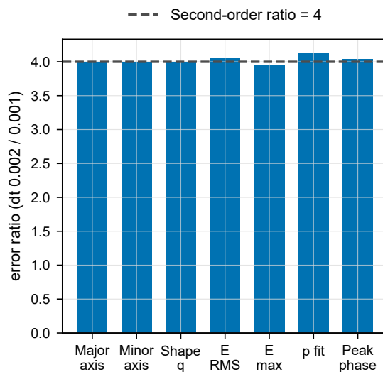
f Effect of halving the time step
