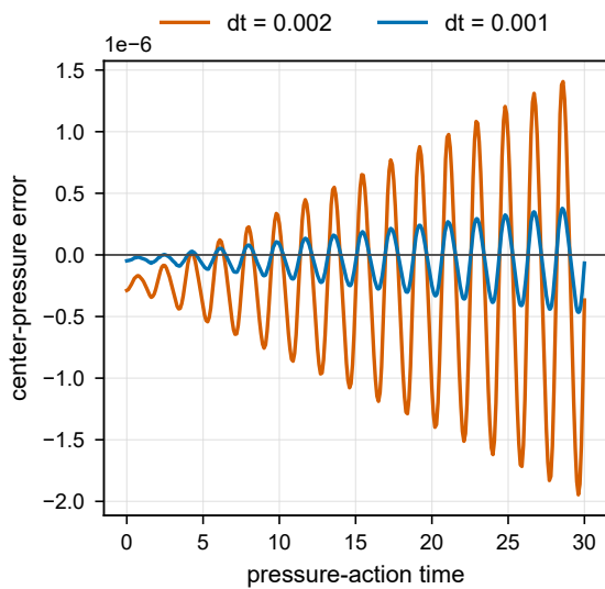
e Center-pressure accuracy
