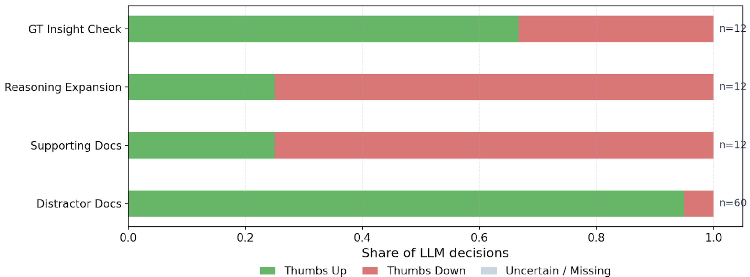
Chosen LLM Judge Vote Distribution
