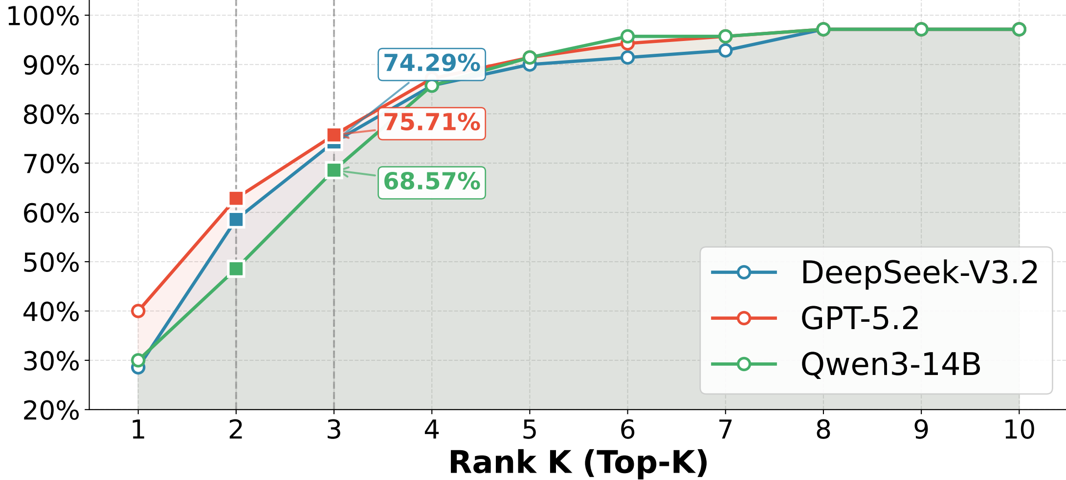
Cumulative Hit Rate
